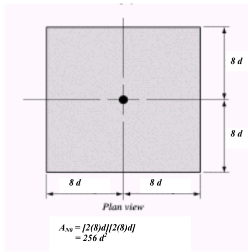
Figure 3-3 Calculation of A_{N0} for the uniform bond stress model using the anchor diameter
