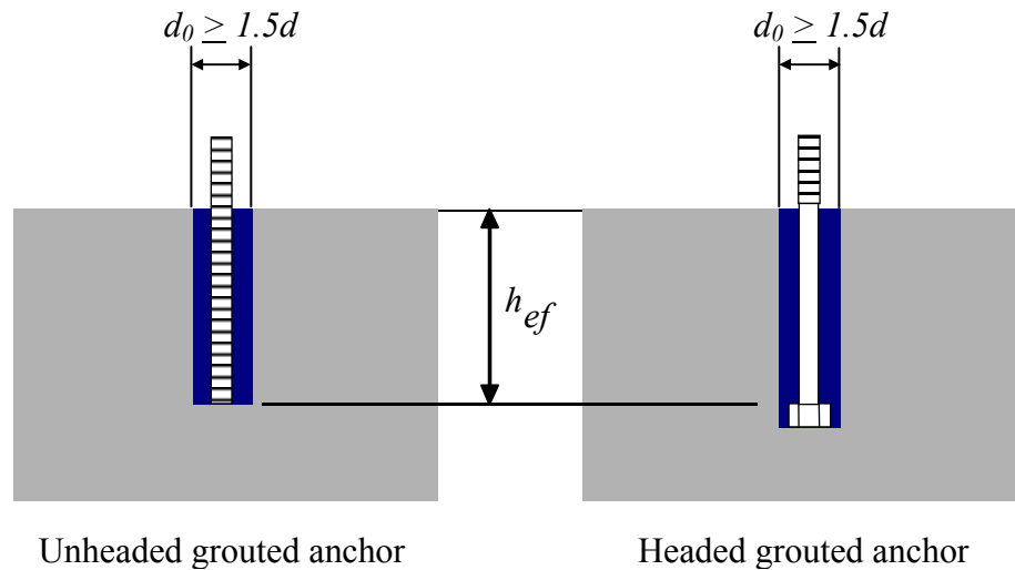
Figure 2-2 Examples of typical unheaded and headed grouted anchors
