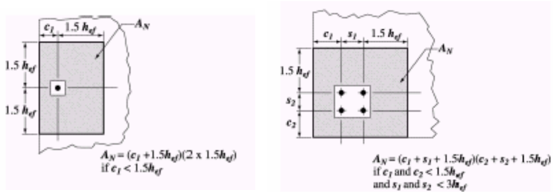
Figure 3-2 Projected areas for single anchors and anchor groups for the CCD method
