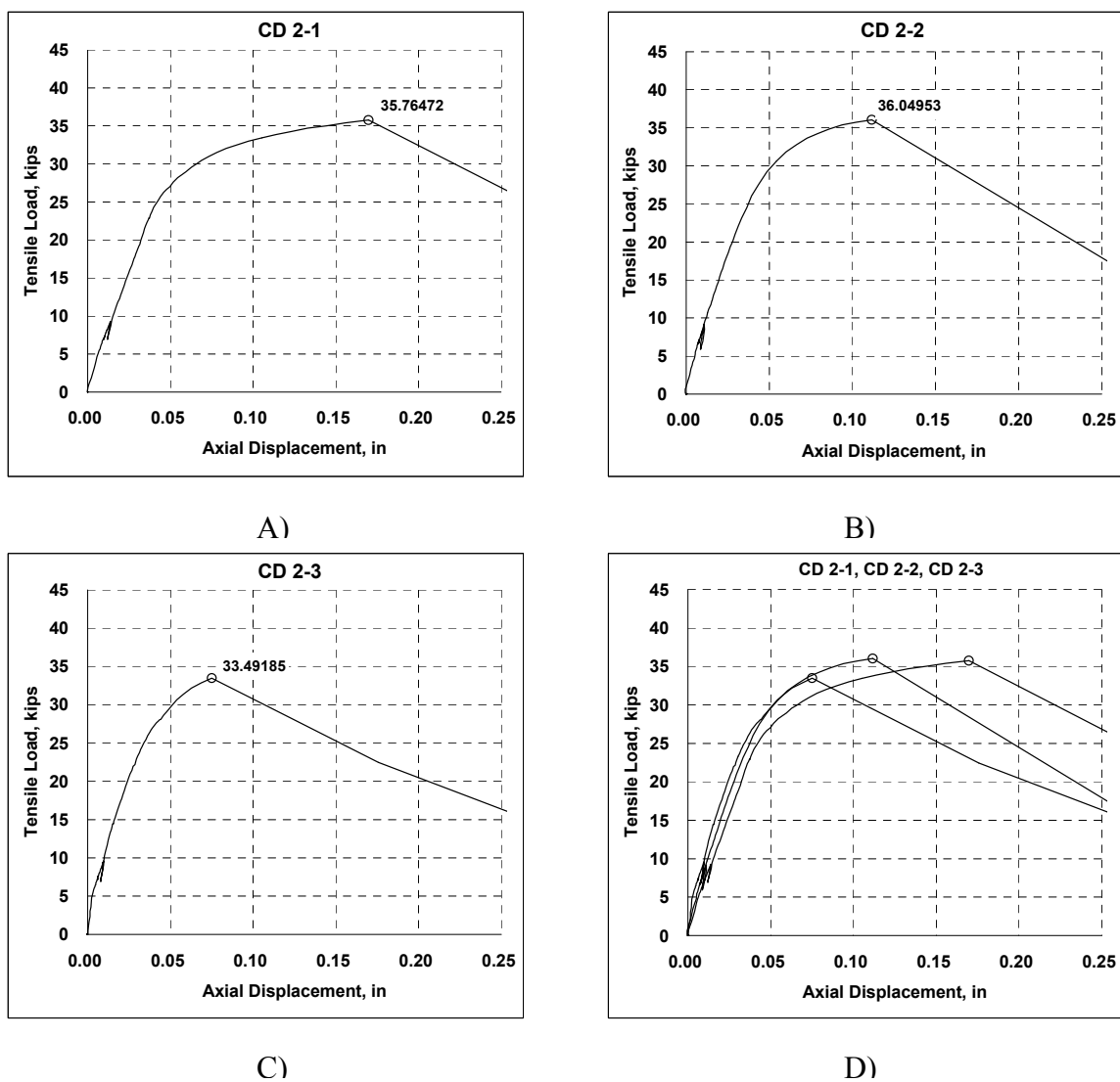
Figure B-2 Graphs of test results of second installation of core-drilled anchors A) First test in series; B) Second test in series; C) Third test in series; D) Comparison of all test in series
