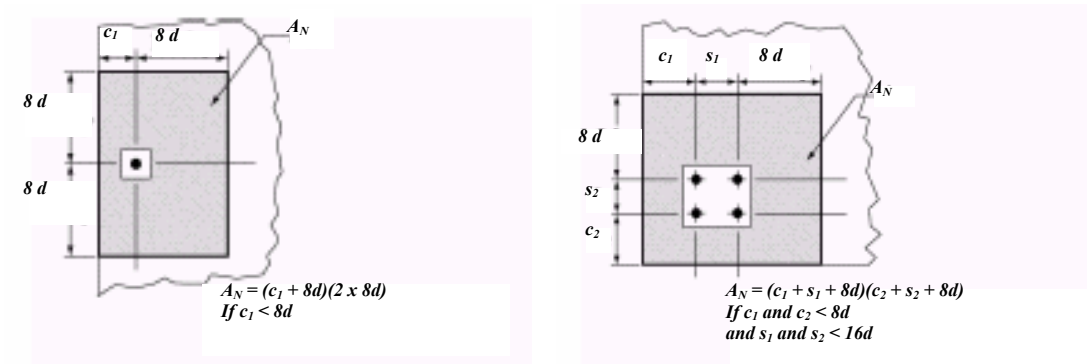
Figure 3-3 Calculation of A_{N0} for the uniform bond stress model using the anchor diameter
