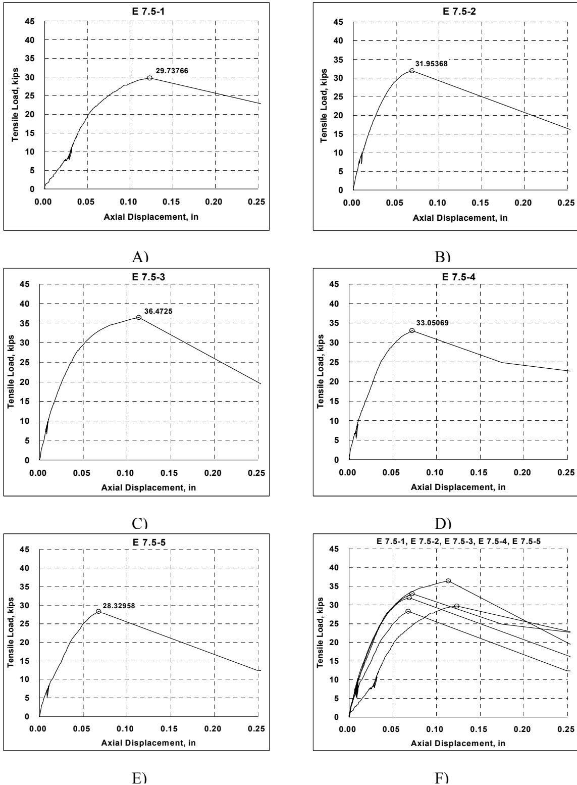
Figure C-3 Graphs of test results of core-drilled anchors installed 7.5 inches away from one edge A) First test in series; B) Second test in series; C) Third test in series; D) Fourth test in series; E) Fifth test in series; F) Comparison of all test in series
