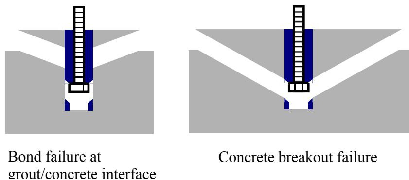
Figure 2-4 Typical bond failure at the grout/concrete interface and concrete cone breakout failure of headed grouted anchors
