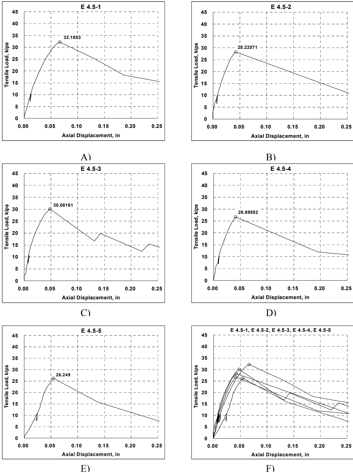
Figure C-1 Graphs of test results of core-drilled anchors installed 4.5 inches away from one edge A) First test in series; B) Second test in series; C) Third test in series; D) Fourth test in series; E) Fifth test in series; F) Comparison of all test in series
