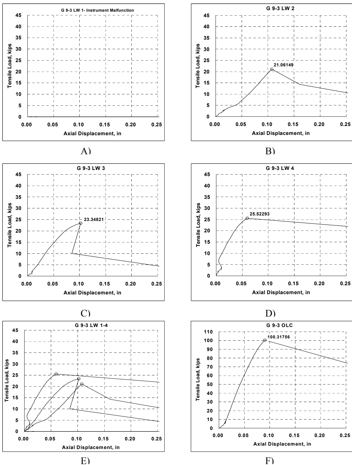
Figure D-6 Graphs of results of third core-drilled anchor group installed with anchor spacing of 9.0 inches A) Load on first anchor; B) Load on second anchor; C) Load on third anchor; D) Load on fourth anchor; E) Comparison of all anchor loads in test; F) Load on entire anchor group
