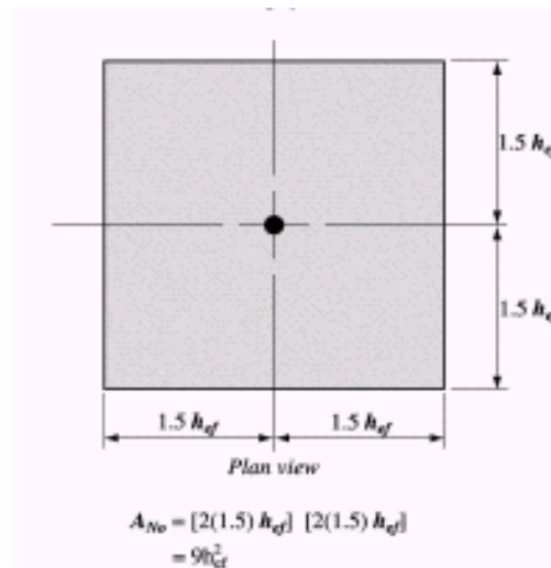
Figure 3-1 Calculation of A_{N0} for the CCD method
