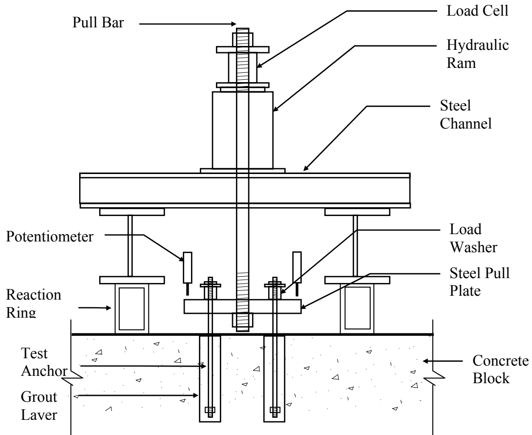
Figure 5-2 Group anchor test apparatus
