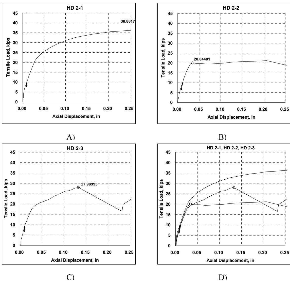
Figure B-5 Graphs of test results of second installation of hammer-drilled anchors A) First test in series; B) Second test in series; C) Third test in series; D) Comparison of all test in series
