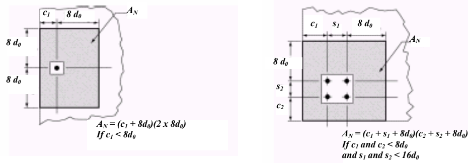
Figure 3-6 Projected areas for single anchors and anchor groups for the uniform bond stress model using the hole diameter
