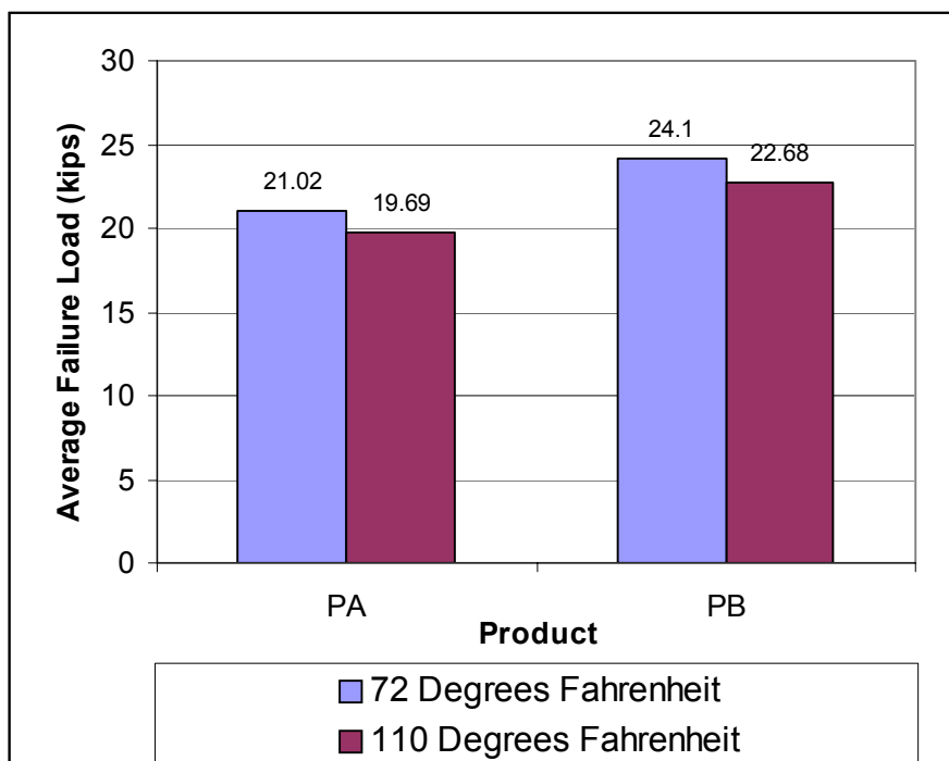
Figure F-9 Comparison of average failure loads for tests performed at ambient and elevated temperatures
