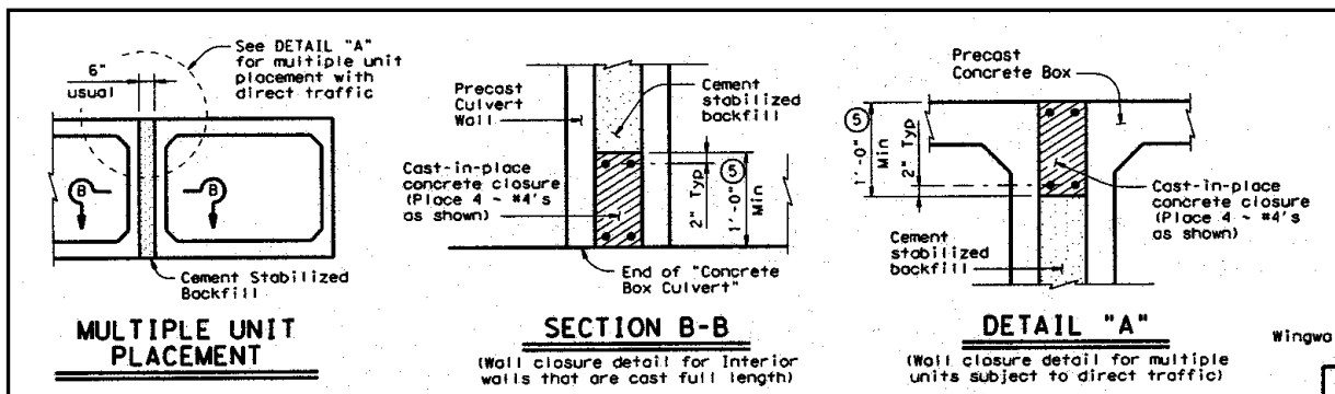
Figure 5.14: Multiple Unit Placement Details
