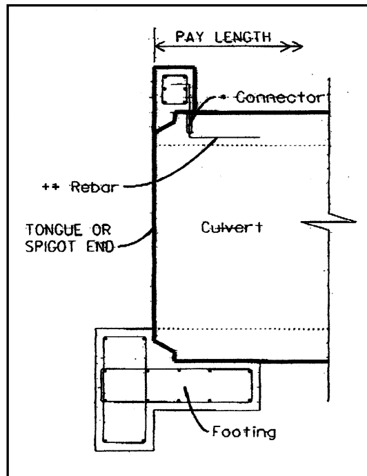
Figure 5.9: Outlet End Detail
