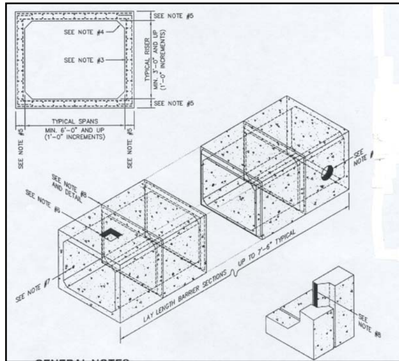
Figure 1.3: Single Cell Square/Rectangular Culvert
