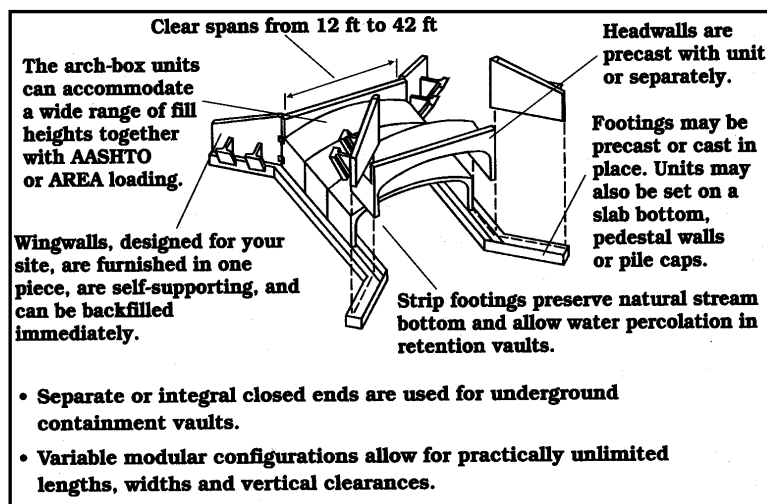
Figure 1.10: CON/SPAN Arch Culvert System Components
