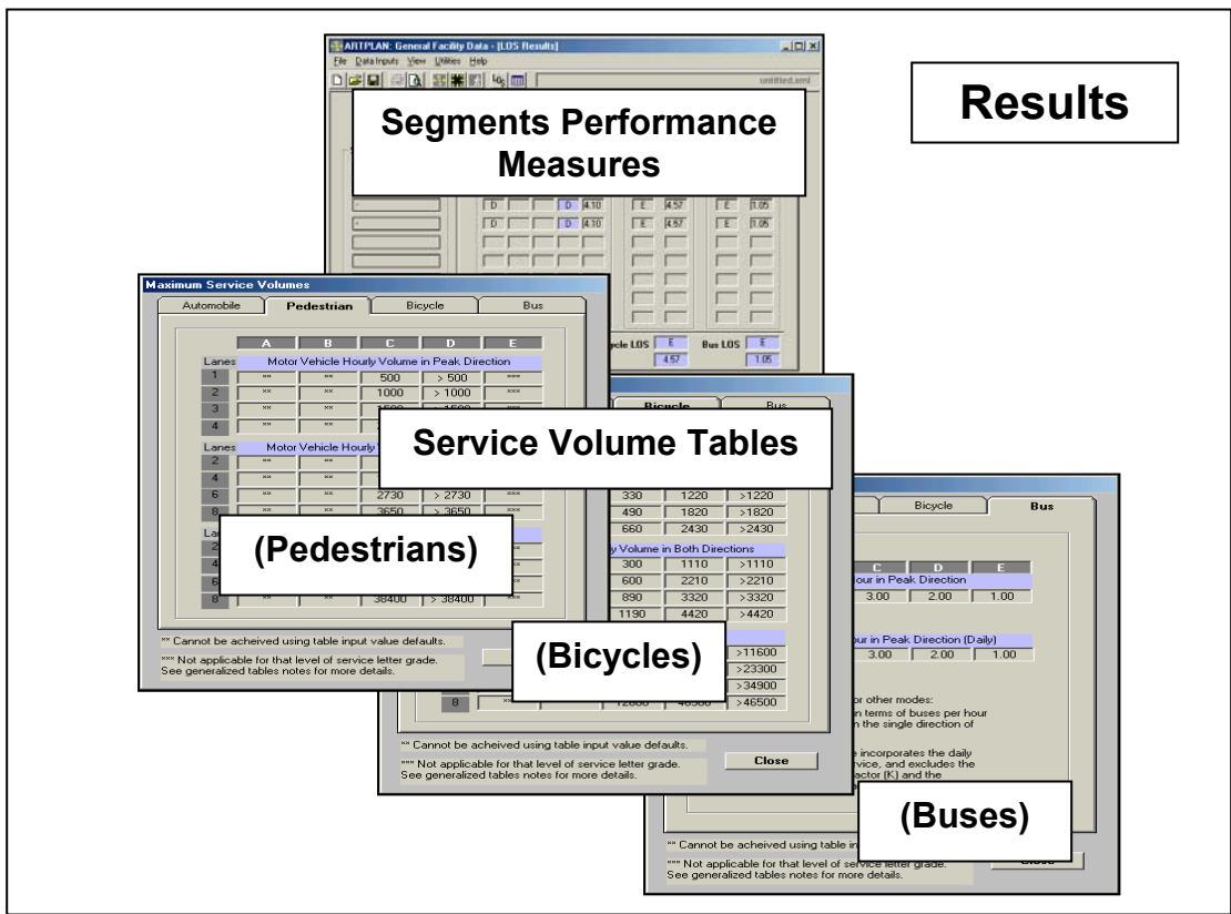
Figure 2. Screen Display Organization for ARTPLAN (Multimodal)
