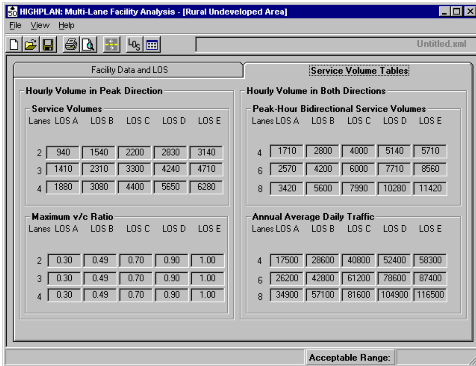
Figure A-16. HIGHPLAN: Service Volume Tables
