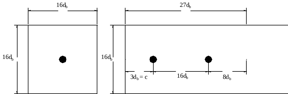
Figure 2.4: Projected area of single anchor ( A_{n0} ) and group of anchors ( A_n )
