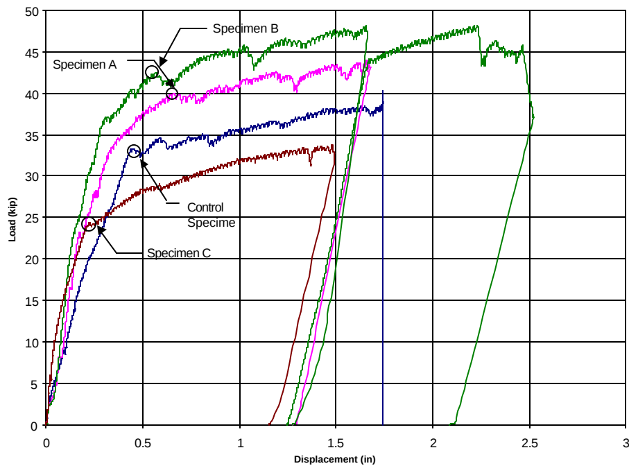
Figure 4.2 – Results for Test Series 2 moment tests
