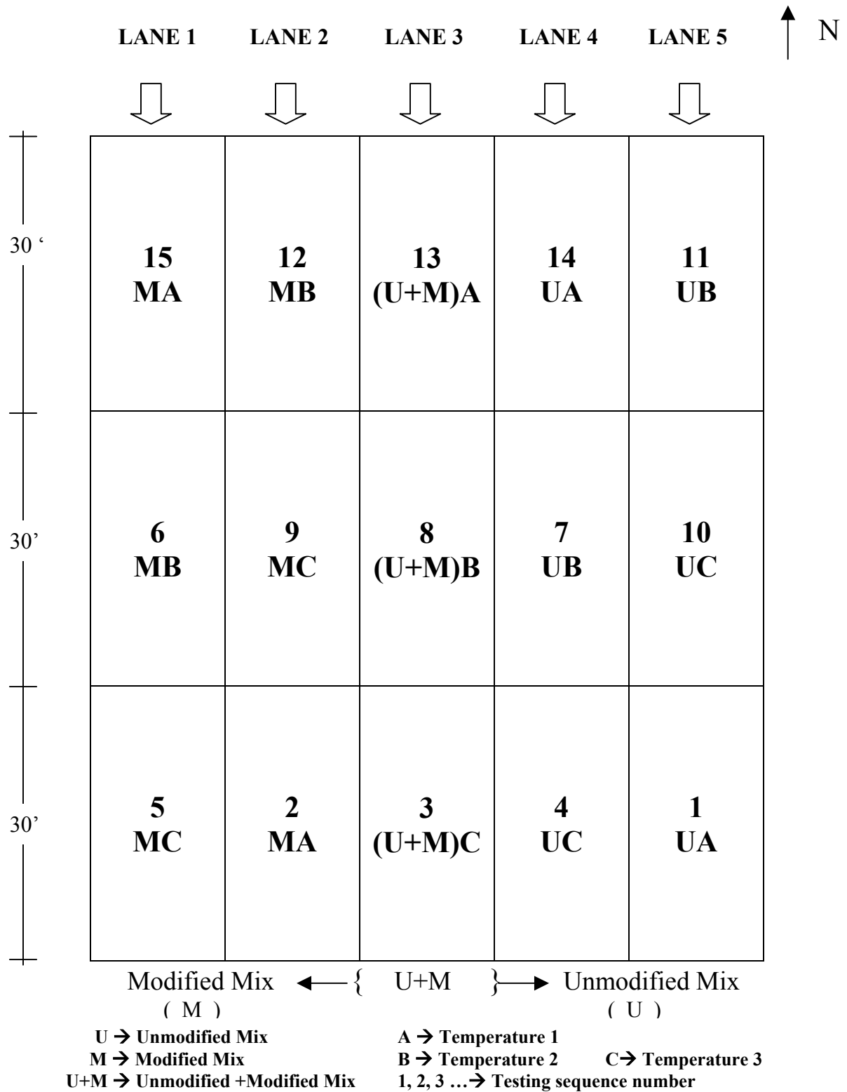
Figure 3.2 Testing Sequence (Plan View)
