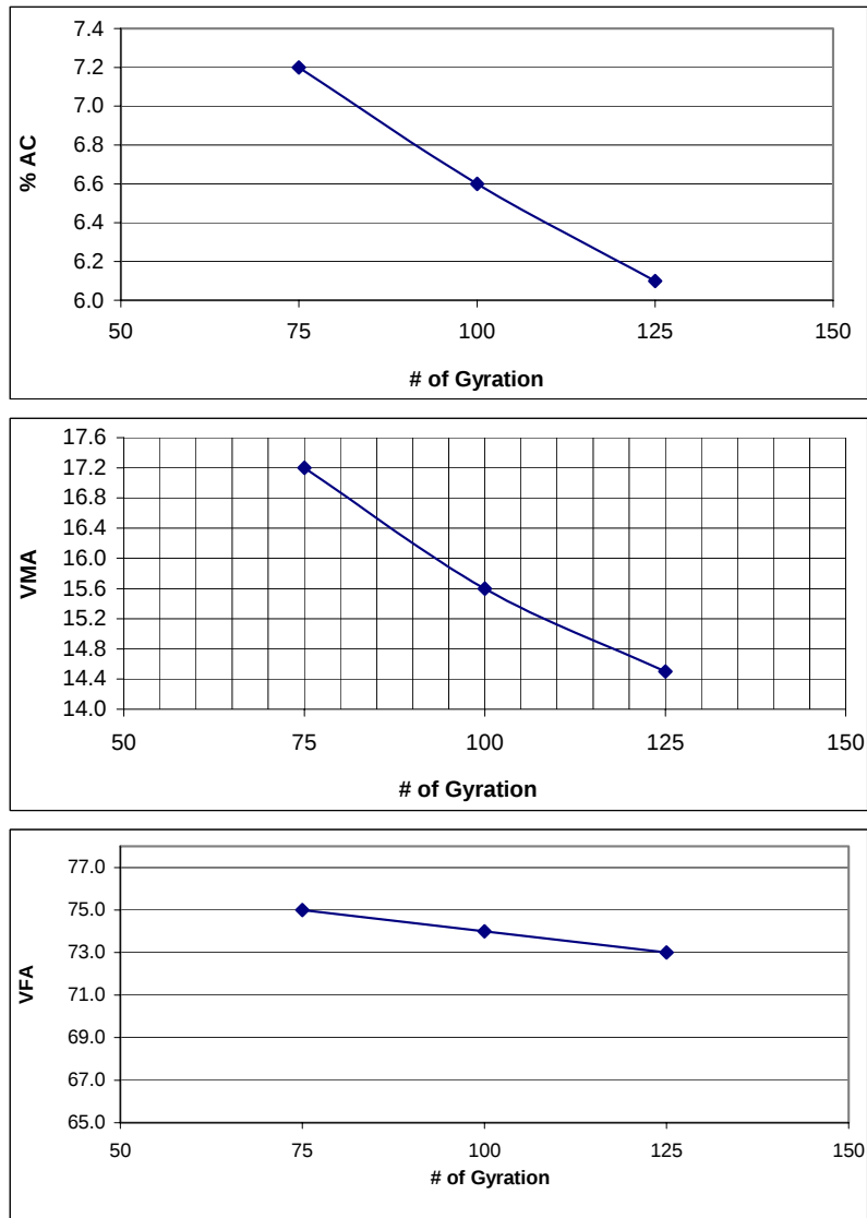
Figure B.1 Volumetric properties with number of gyrations at 4% air voids (Coarse 1).
