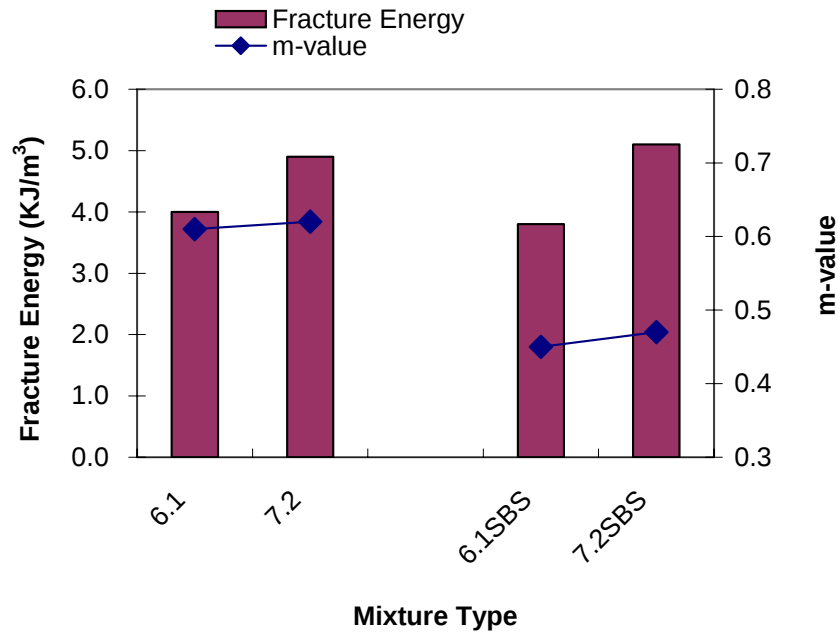
Figure 4.1 Fracture energy and m-value from Superpave IDT.
