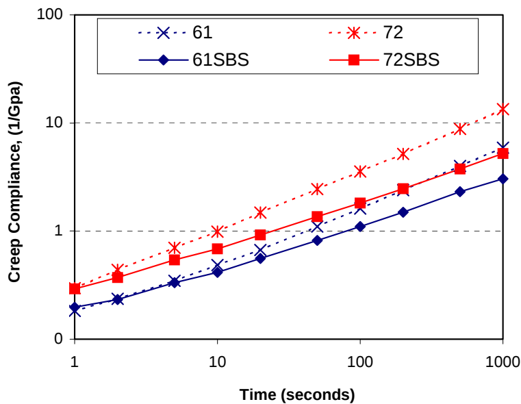
Figure 4.11 Creep compliance of coarse-graded mixtures (10°C, STOA).
