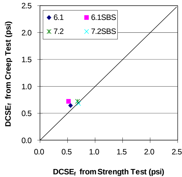
Figure 4.17 Comparison of DCSE_f between creep and strength test.
