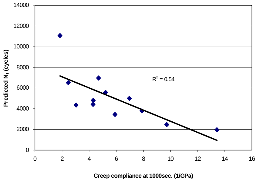
Figure 4.25 Relationship between predicted N_f and creep compliance.
