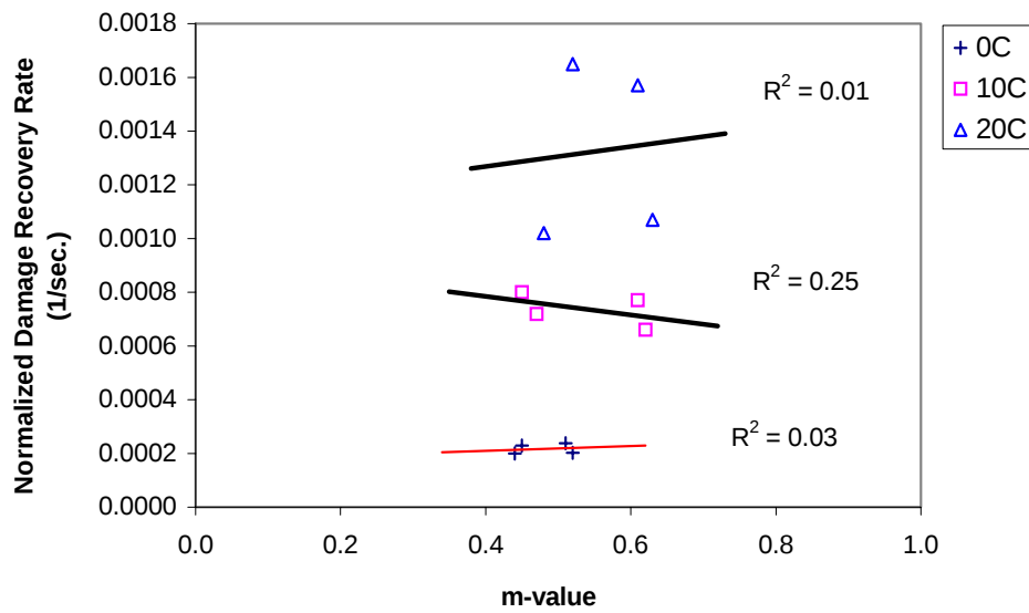
Figure 5.16 Relationship between normalized damage recovery rate and m-value.
