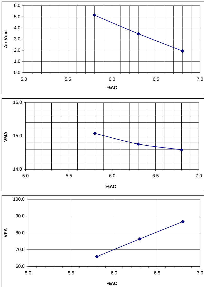
Figure B.9 Volumetric properties with asphalt contents at N_d = 125 (Fine 1).
