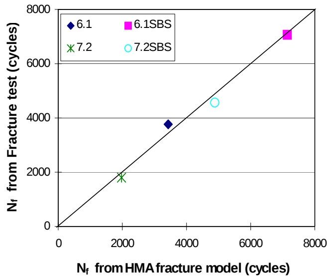
Figure 4.18 Comparison of measured and predicted N_f .
