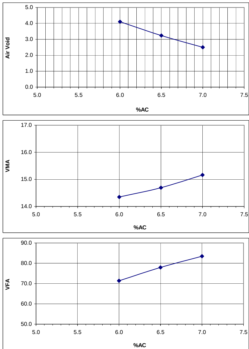
Figure B.4 Volumetric properties with asphalt contents at N_d = 125 (Coarse 1).
