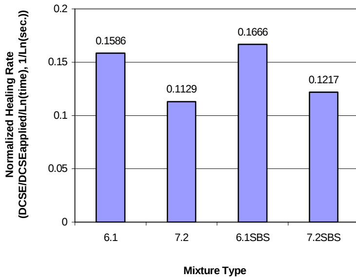
Figure 5.8 Comparison of normalized healing rates at 15° C.
