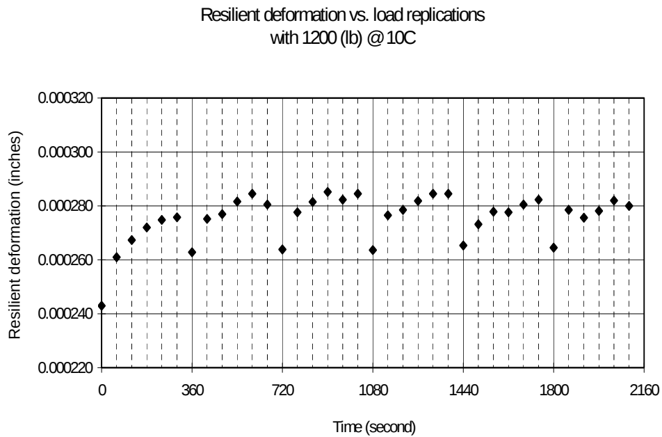
Figure D.6 Healing test (6.1% modified asphalt, Coarse 1, 1200 (lb) cyclic load at 10° C).
