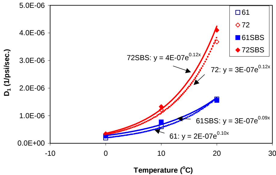
Figure 4.8 Temperature sensitivity of D_1 .
