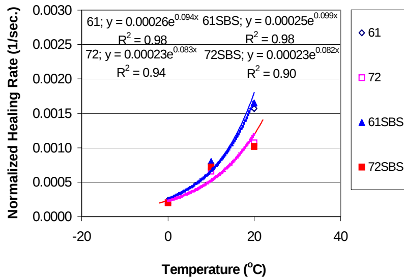
Figure 5.14 Temperature sensitivity of normalized damage recovery rate.
