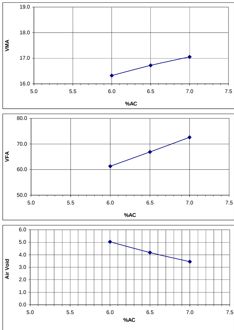
Figure B.2 Volumetric properties with asphalt contents at N_d = 75 (Coarse 1).
