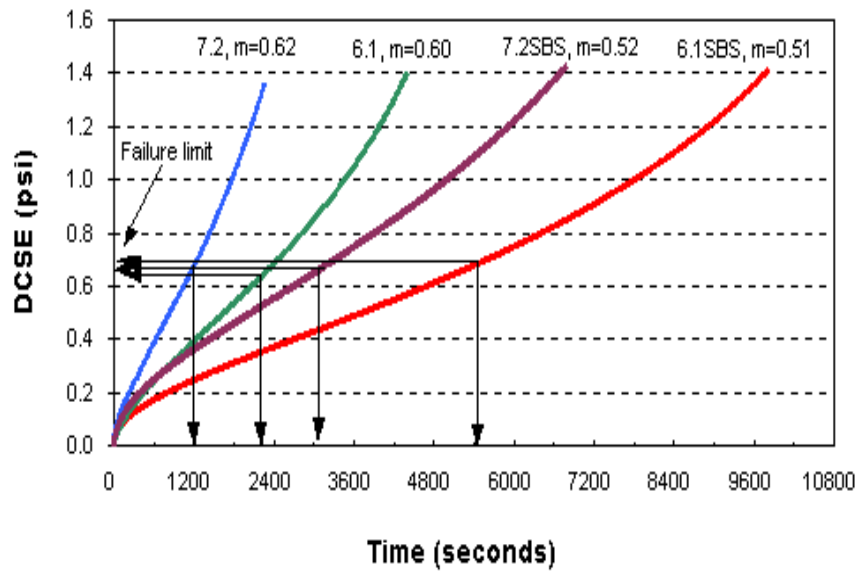
Figure 4.16 Creep test results (DCSE vs. time).
