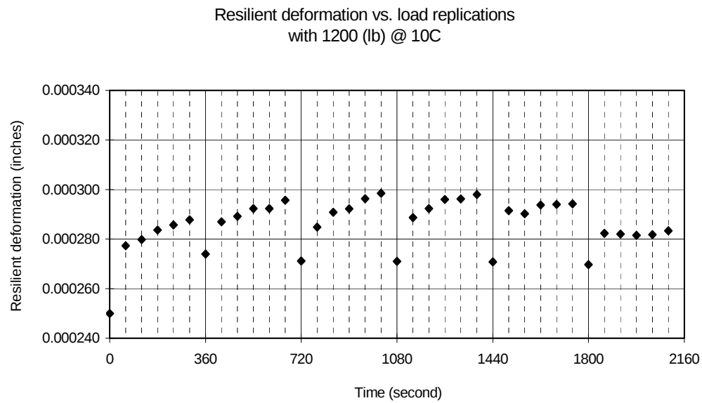
Figure D.7 Healing test (7.2% modified asphalt, Coarse 1, 1200 (lb) cyclic load at 10° C).
