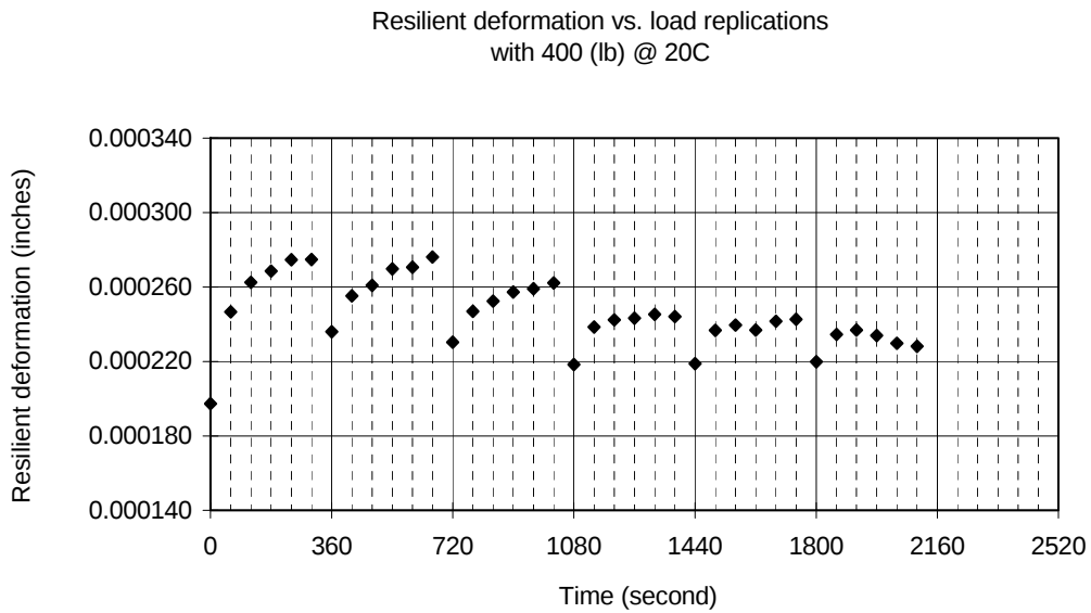
Figure D.10 Healing test (6.1% modified asphalt, Coarse 1, 400 (lb) cyclic load at 20° C).
