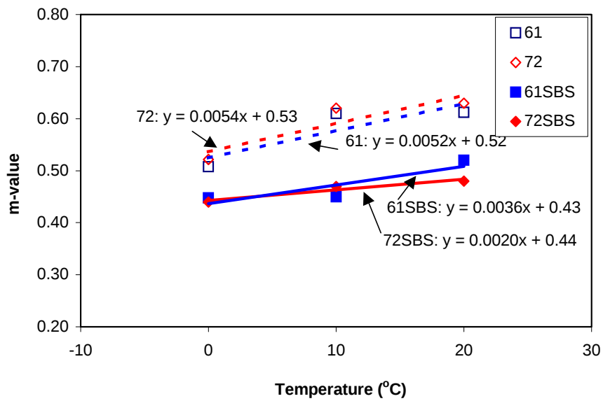
Figure 4.7 Temperature sensitivity of m-value.
