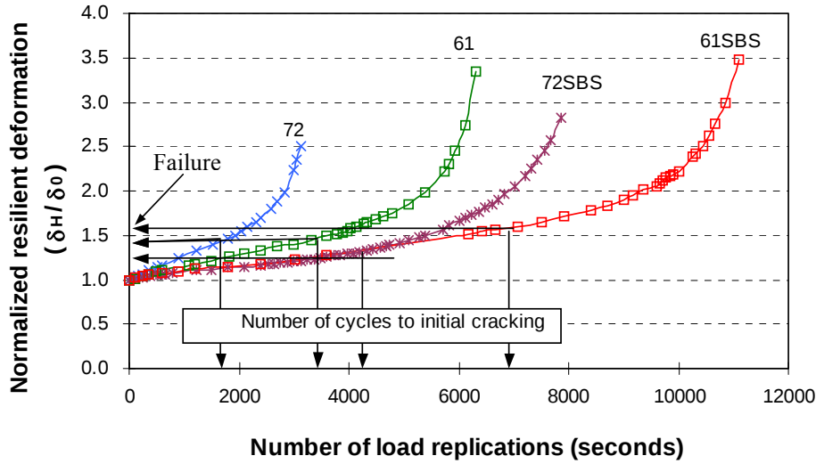
Figure 4.10 Fracture test results (STOA, Coarse 1, and 10° C).
