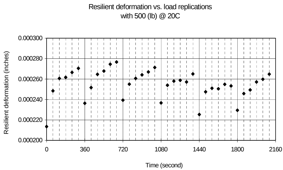
Figure D.8 Healing test (6.1% unmodified asphalt, Coarse 1, 500 (lb) cyclic load at 20° C).
