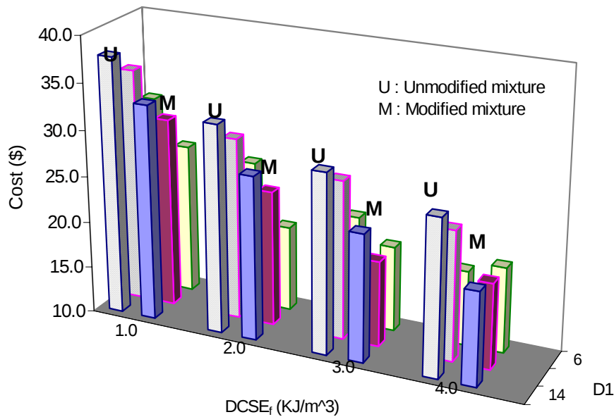
Figure 6.1 Comparison of construction cost of AC layer depending on mixture properties for conventional pavement and low traffic level.
