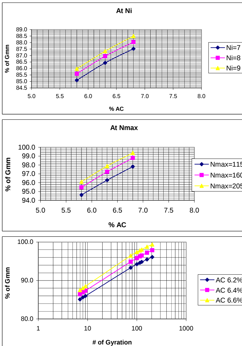
Figure B.10 Percentage of Gmm (Fine 1).
