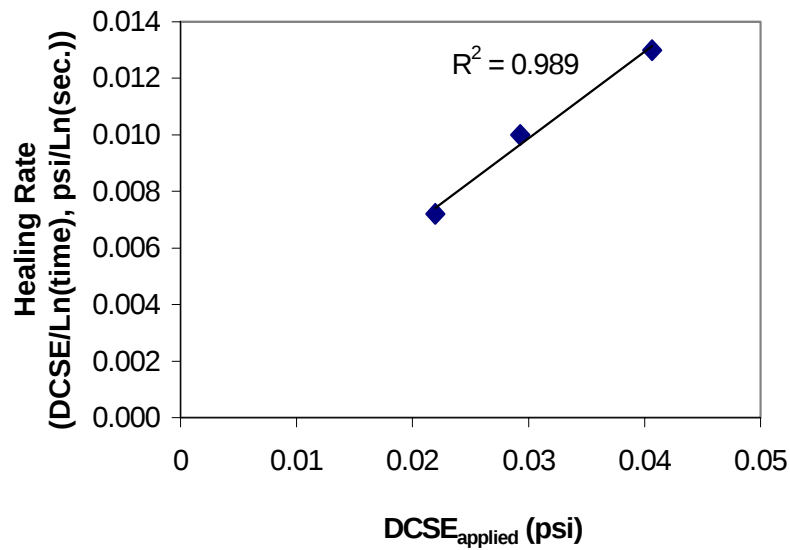
Figure 5.5 Healing rates in terms of DCSE with different DCSE applied on same mixtures (6.1SBS, loading with 55 psi and healing at 20° C).
