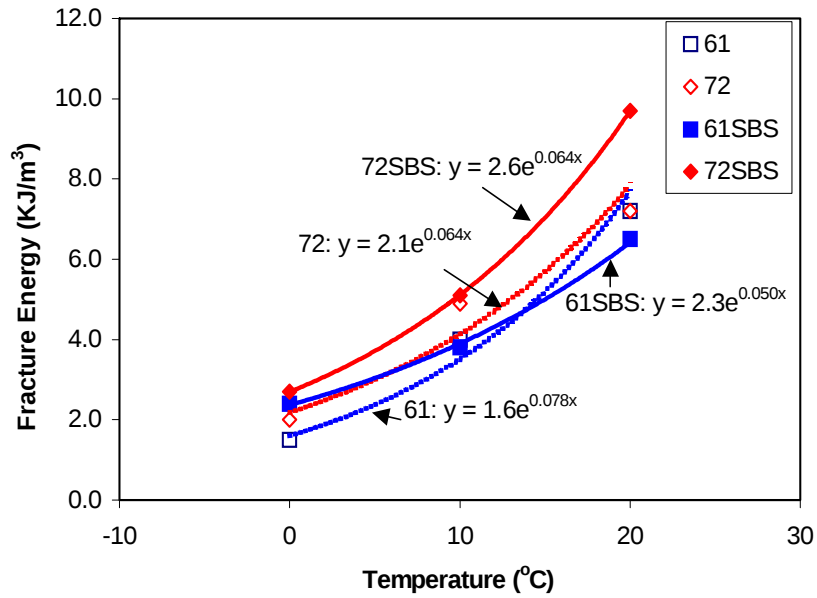
Figure 4.5 Temperature sensitivity of fracture energy.
