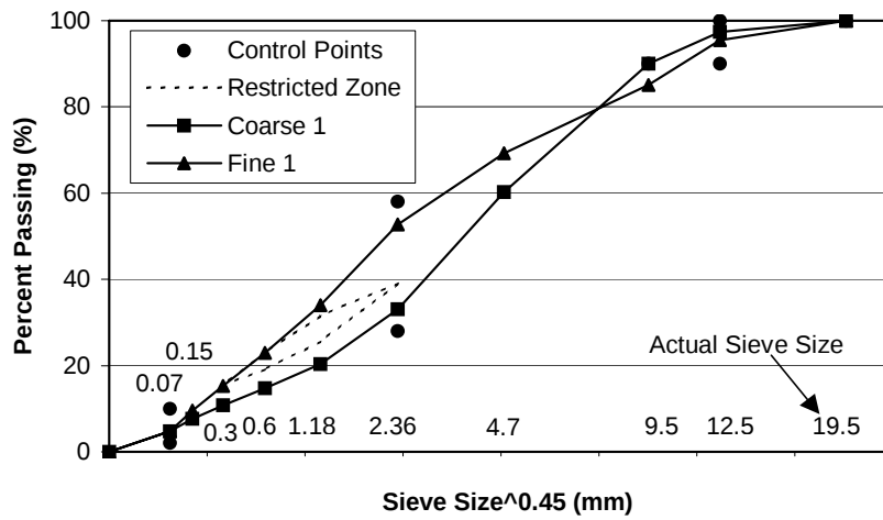
Figure 3.1 Aggregate gradations (Coarse 1 and Fine 1).
