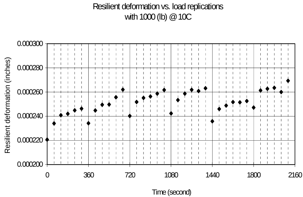
Figure D.5 Healing test (7.2% unmodified asphalt, Coarse 1, 1000 (lb) cyclic load at 10° C).
