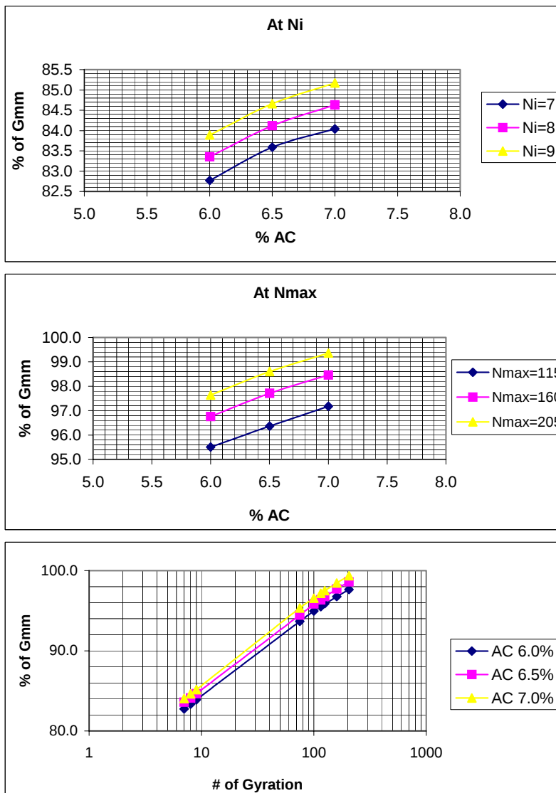
Figure B.5 Percentage of Gmm (Coarse 1).
