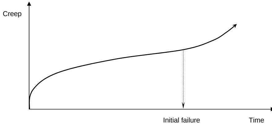
Figure 3.10 Typical behavior and initial failure in creep.
