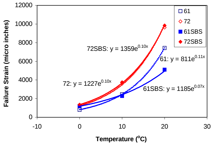
Figure 4.4 Temperature sensitivity of failure strain.
