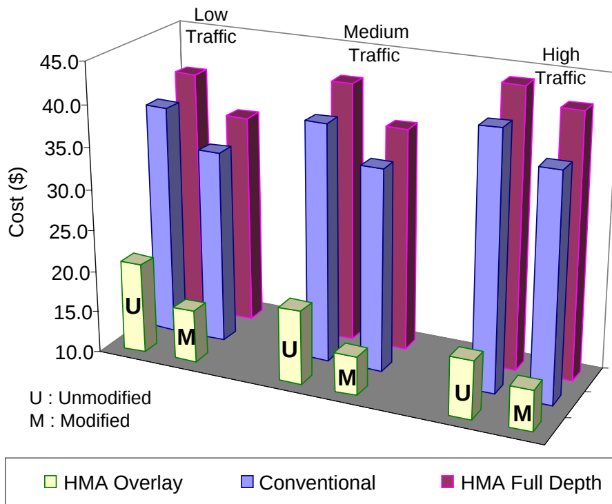
Figure 6.2 Comparison of construction cost of AC layer depending on pavement structure and traffic level for the mixtures with DCSE_f = 1.0 ( \text{KJ/m}^3 ) and D_1 = 14 \times 10^{-7} (1/psi).
