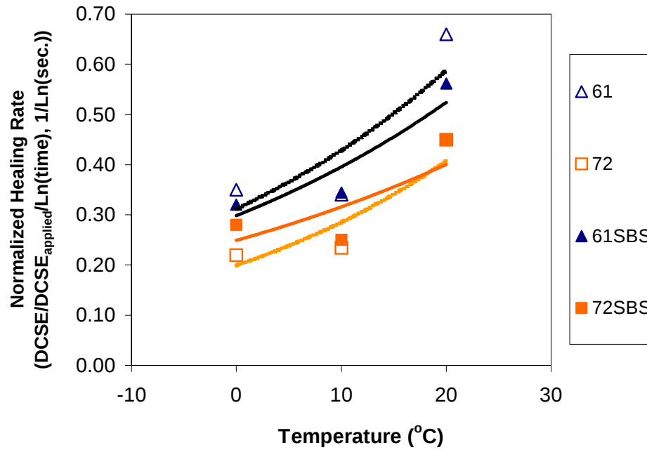
Figure 5.9 Temperature sensitivity of normalized healing rate.
