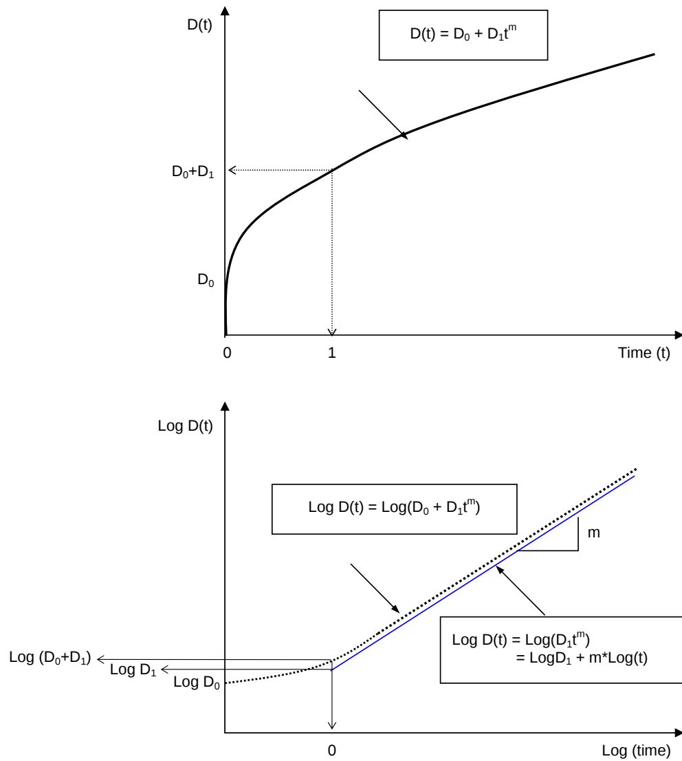
Figure 3.8 Power model of the creep compliance.
