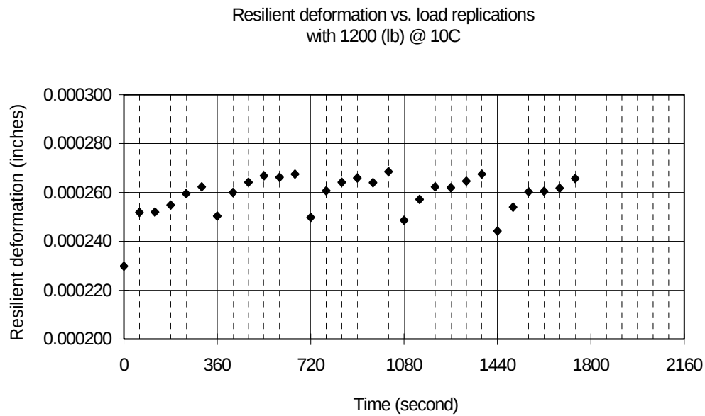
Figure D.4 Healing test (6.1% unmodified asphalt, Coarse 1, 1200 (lb) cyclic load at 10° C).
