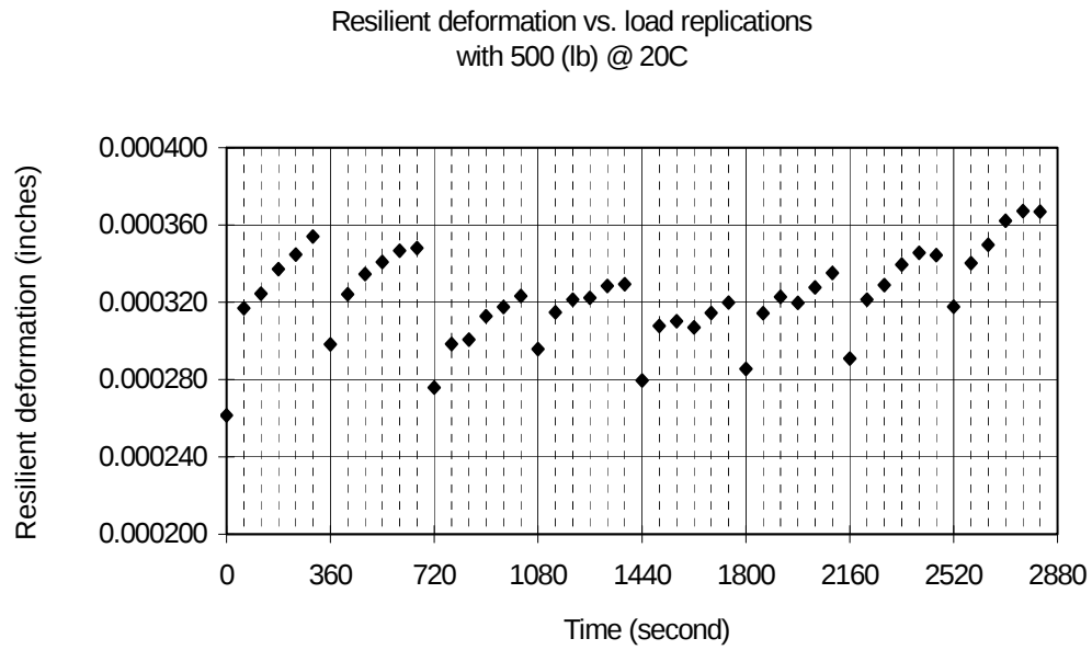
Figure D.9 Healing test (7.2% unmodified asphalt, Coarse 1, 500 (lb) cyclic load at 20° C).
