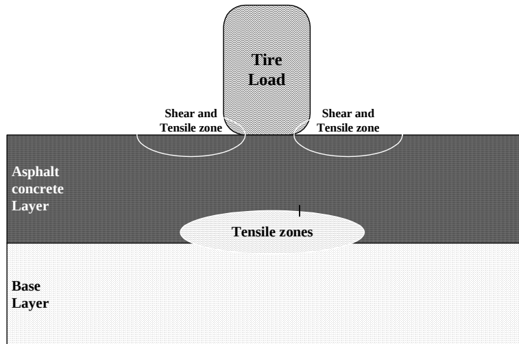
Figure 2.1 Schematic locations of shear and tensile stress zones in the asphalt concrete pavement (after Lytton et al. 2001)
