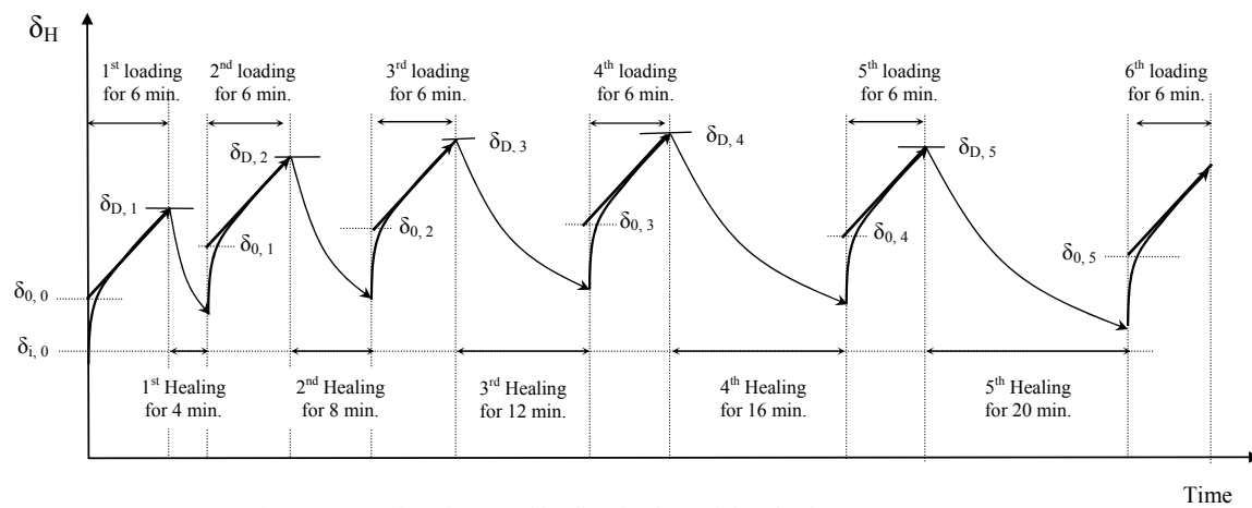
Figure 5.11 Series of repeated loading for determining the damage recovery rate.
