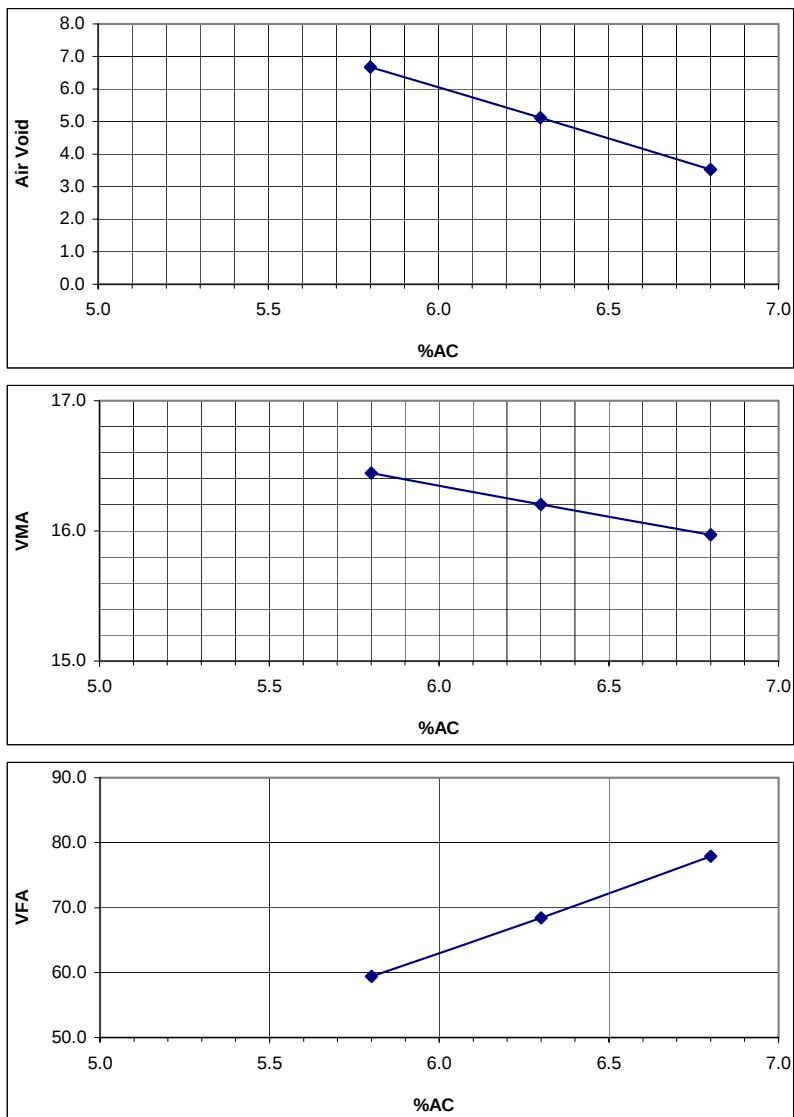
Figure B.7 Volumetric Properties with Asphalt Contents at N_d = 75 (Fine 1).
