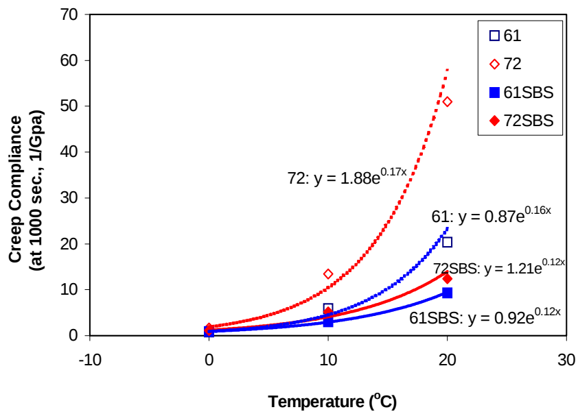
Figure 4.6 Temperature sensitivity of creep compliance.
