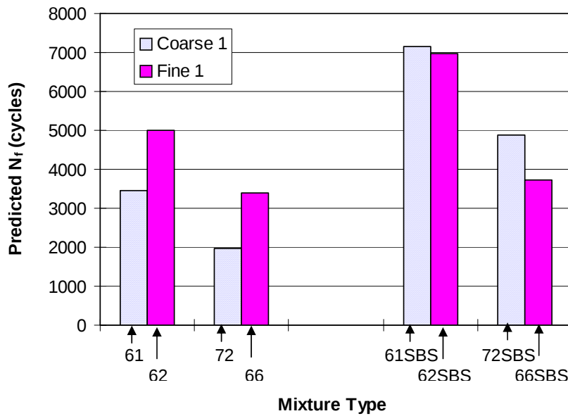
Figure 4.24 Comparison of predicted N_f of coarse and fine graded mixtures.
