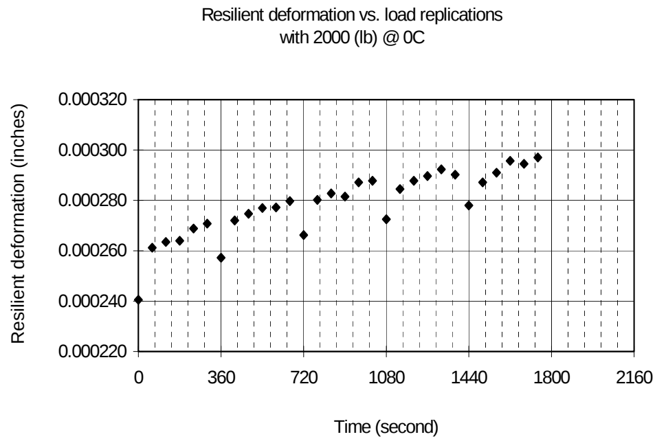
Figure D.3 Healing test (7.2% modified asphalt, Coarse 1, 2000 (lb) cyclic load at 0° C).
