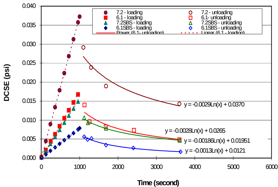
Figure 5.1 Healing test results, loading (1000 cycles with 75psi) and healing at 15° C.
