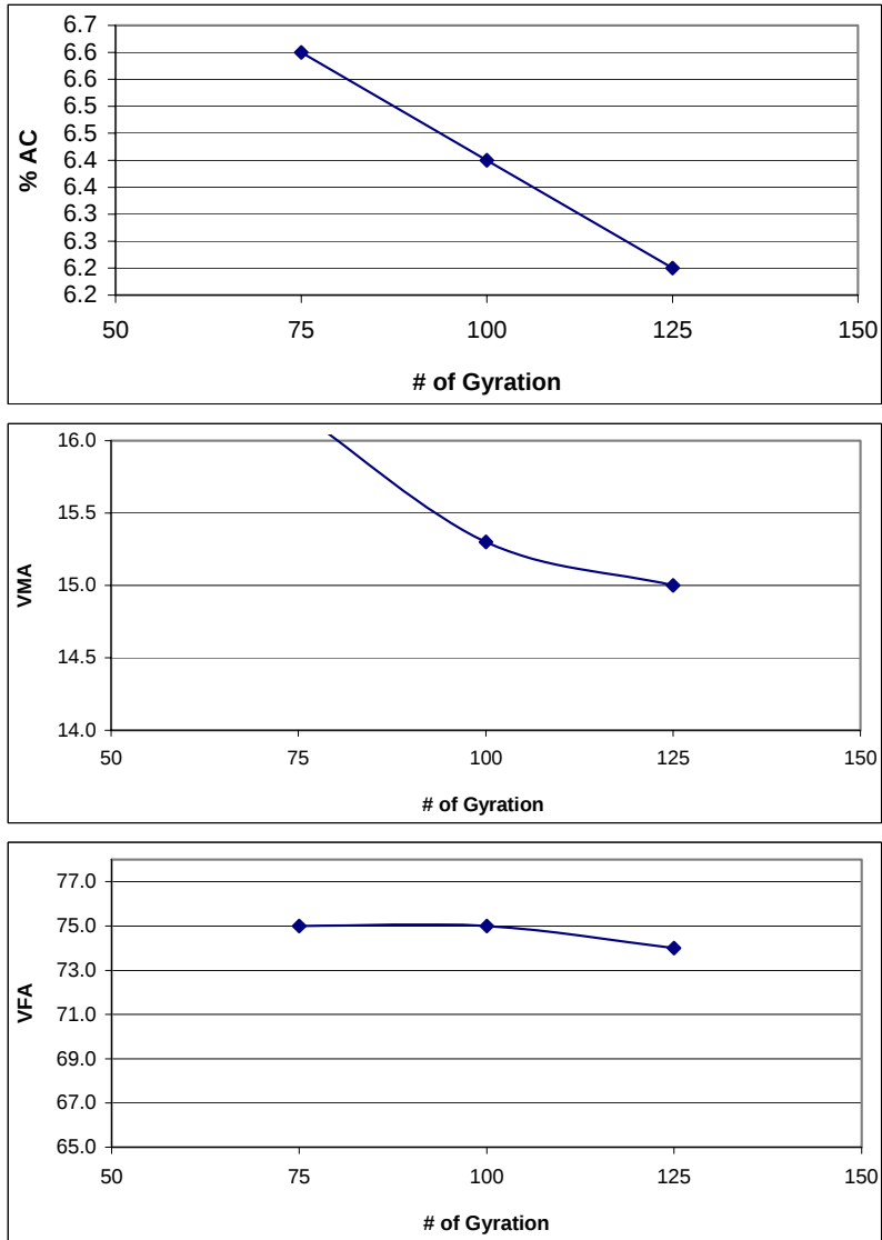
Figure B.6 Volumetric Properties with Number of Gyration (Fine 1).
