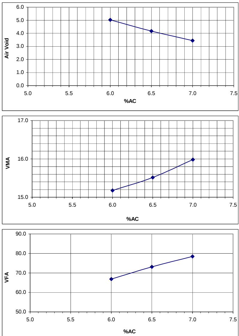
Figure B.3 Volumetric properties with asphalt contents at N_d = 100 (Coarse 1).
