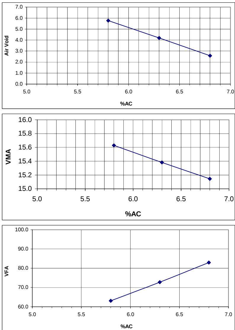
Figure B.8 Volumetric properties with asphalt contents at N_d = 100 (Fine 1).
