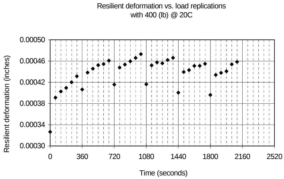
Figure D.11 Healing test (7.2% modified asphalt, Coarse 1, 400 (lb) cyclic load at 20° C).
