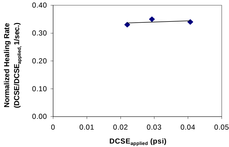
Figure 5.6 Healing rates in terms of DCSE/DCSE_{\text{applied}} with different DCSE_{\text{applied}} on same mixtures (6.1SBS, loading with 55 psi and healing at 20° C).
