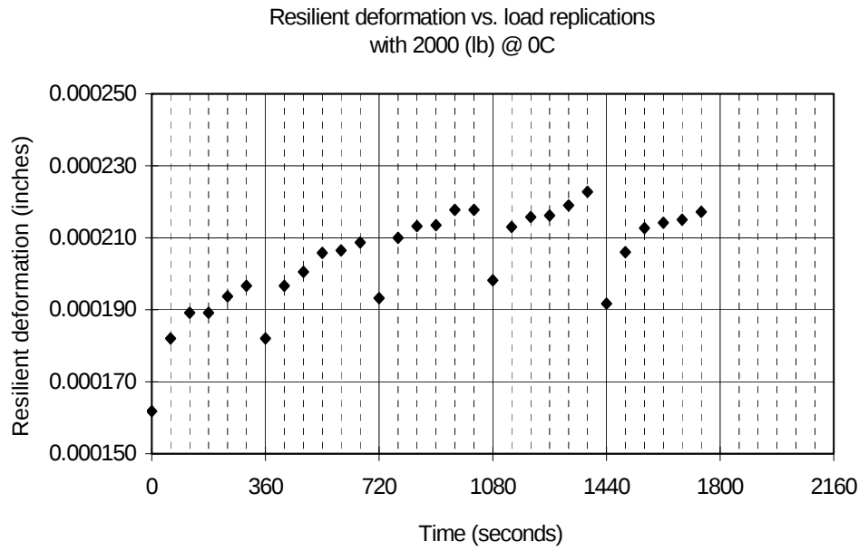
Figure D.1 Healing test (6.1% unmodified asphalt, Coarse 1, 2000 (lb) cyclic load at 0° C).
