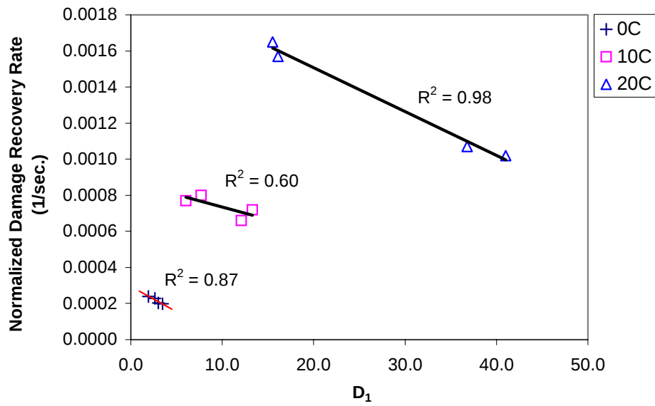
Figure 5.15 Relationship between normalized damage recovery rate and D_1 .
