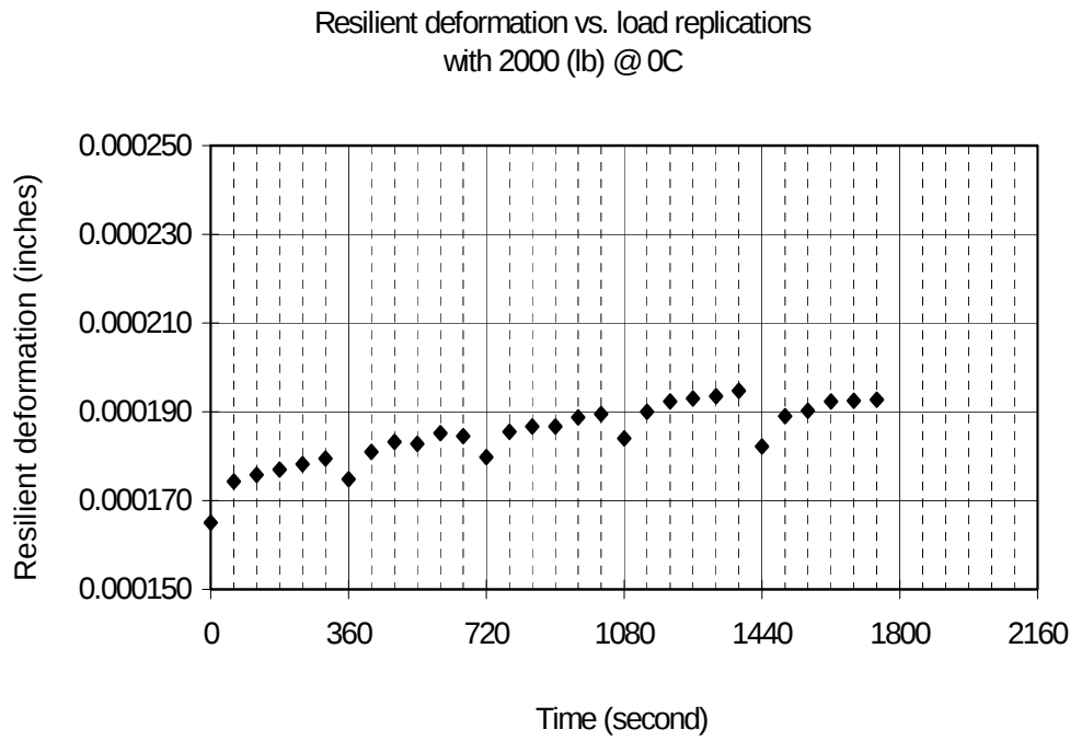
Figure D.2 Healing test (6.1% modified asphalt, Coarse 1, 2000 (lb) cyclic load at 0° C).
