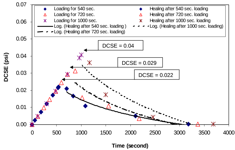
Figure 5.4 Healing test at different DCSE for modified mixtures with 6.1% AC (loading with 55 psi and healing at 20° C).
