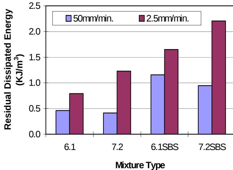
Figure 4.15 Comparison of residual dissipated energy.
