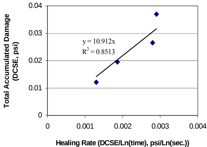
Figure 5.3 Relationship between total accumulated damage and healing rate (1000 cycles loading with 75 psi and healing at 15° C).
