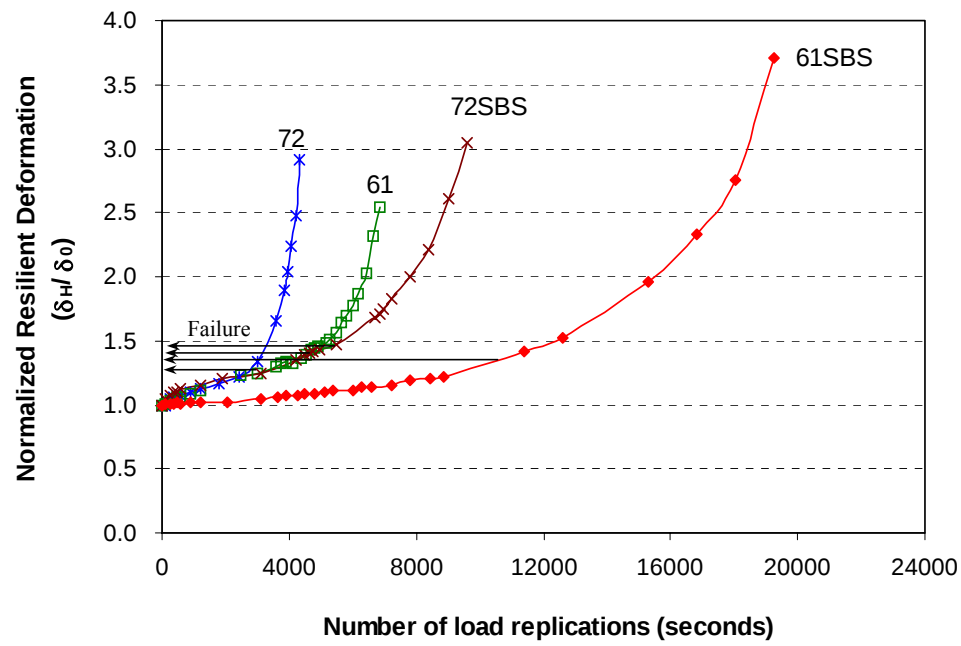
Figure 4.20 Fracture test results (LTOA, Coarse 1, and 10° C).
