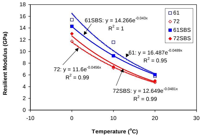
Figure 4.2 Temperature sensitivity of resilient modulus.
