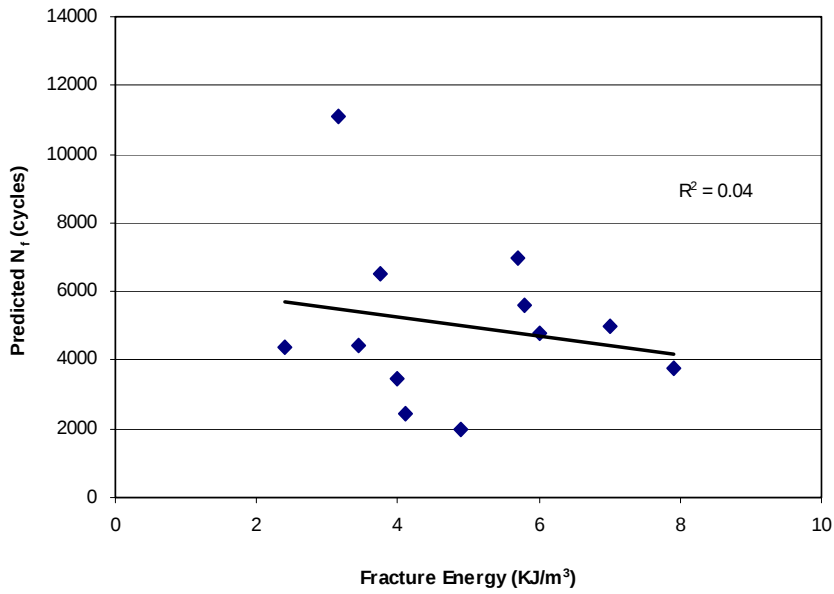
Figure 4.26 Relationship between predicted N_f and fracture energy.
