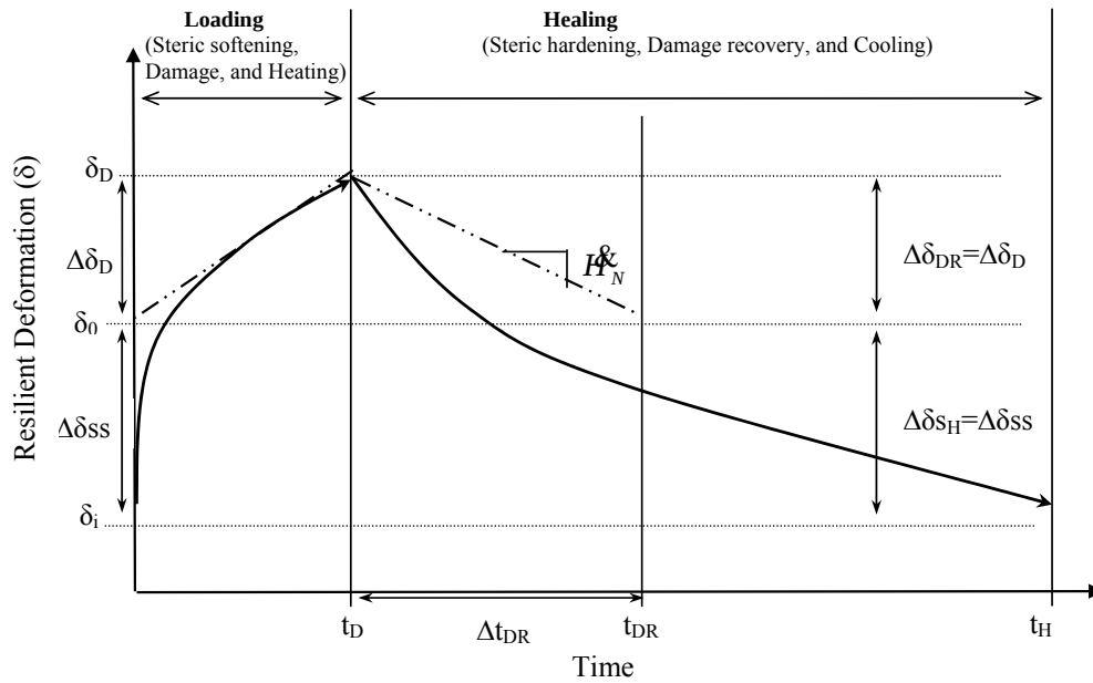
Figure 5.10 Resilient deformations during loading and healing.
