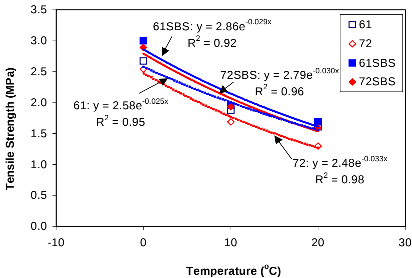
Figure 4.3 Temperature sensitivity of tensile strength.
