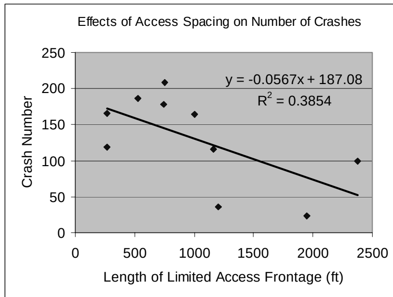
Figure 8: Effect of Length of Limited Access Frontage on the Number of Crashes
