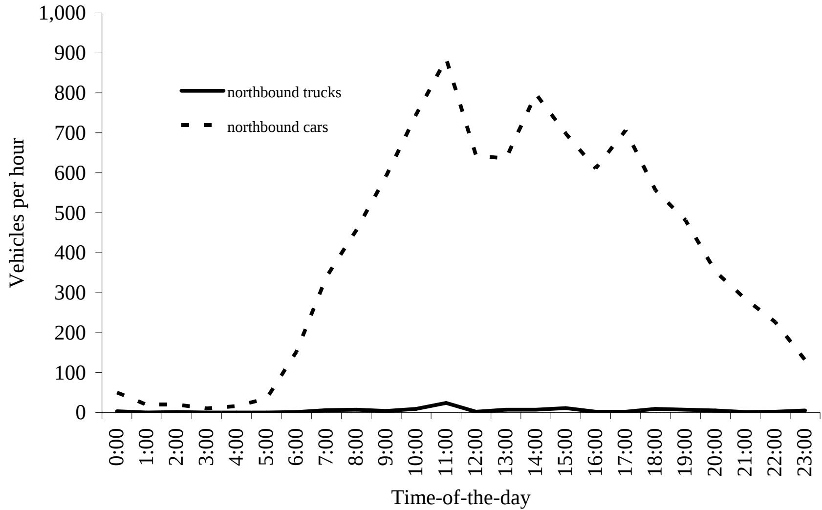
FIGURE B.4: Hourly Variation of Traffic on the Northbound Inside Lane at Milepost 374
