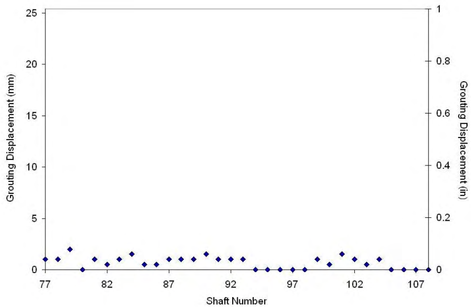
Figure 4-40 PGA Blvd: Phase II production QA data showing uplift for every shaft.
