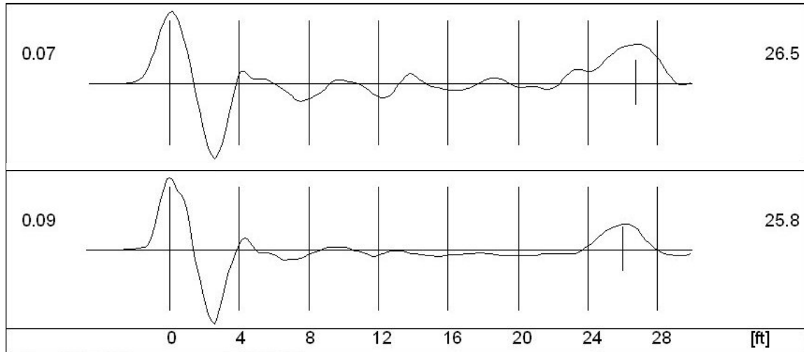
Figure 4-167 Auburn: SIT data for TS-5 before grouting (top) and after load testing (bottom).
