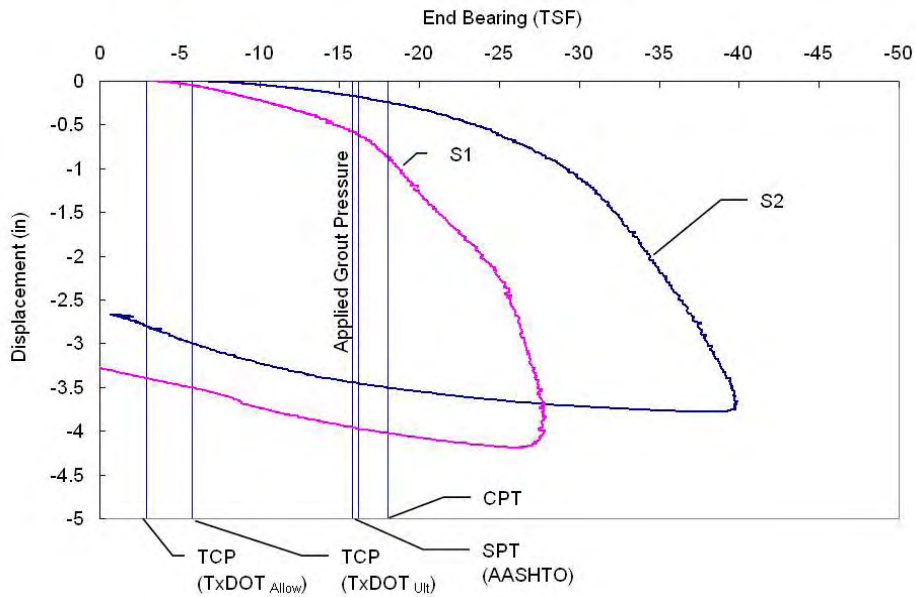
Figure 4-108 TexDOT Demo: End Bearing Stress Plots for Shafts S-1 and S-2.
