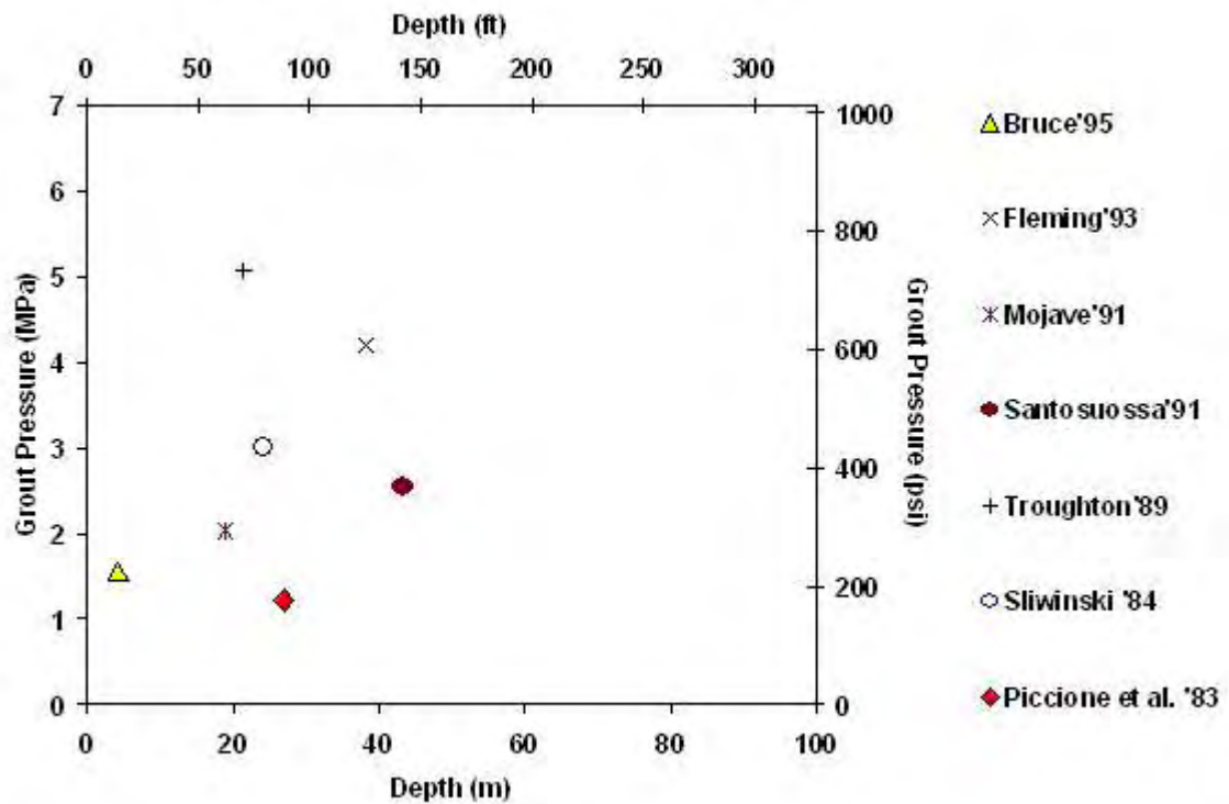
Figure 5-1 Published grout pressure versus depth prior to this research program.
