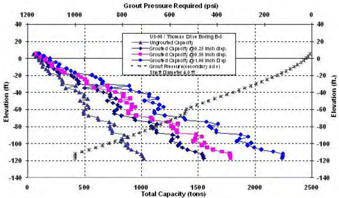
Figure C-222 US 98: B-5, 4ft Diameter
