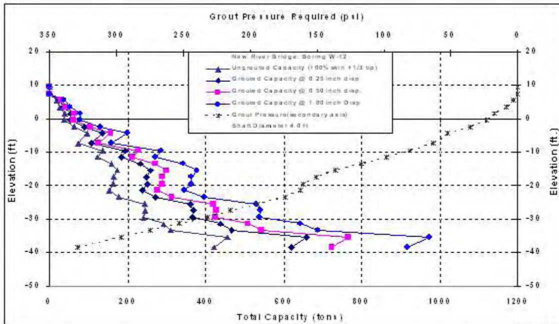
Figure C-160 New River Bridge: W-12, 4ft Diameter
