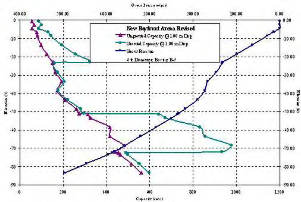
Figure C-90 New Bayfront Arena: B-5, 4ft Diameter
