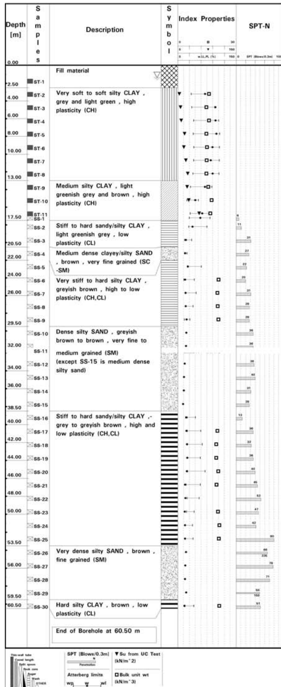
Figure B-6 Bangkok: BH 3
