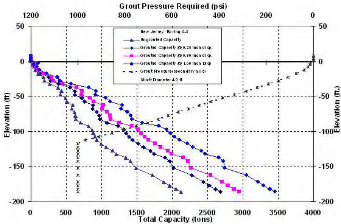
Figure C-164 Newark Legal Center: A-3, 4ft Diameter
