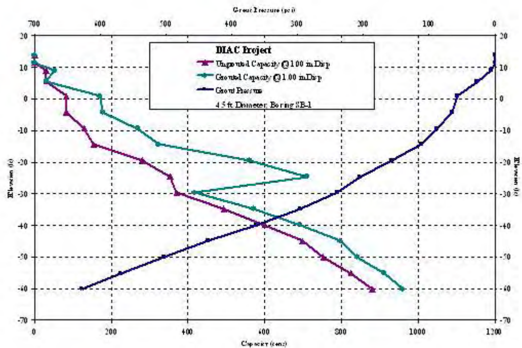
Figure C-12 Bolling Airforce Base: SB-1, 4.5ft Diameter
