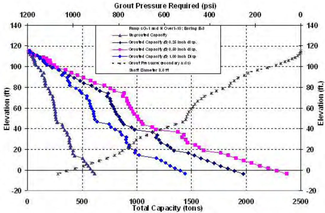
Figure C-36 I-10 / I-110: B-3, 3ft Diameter
