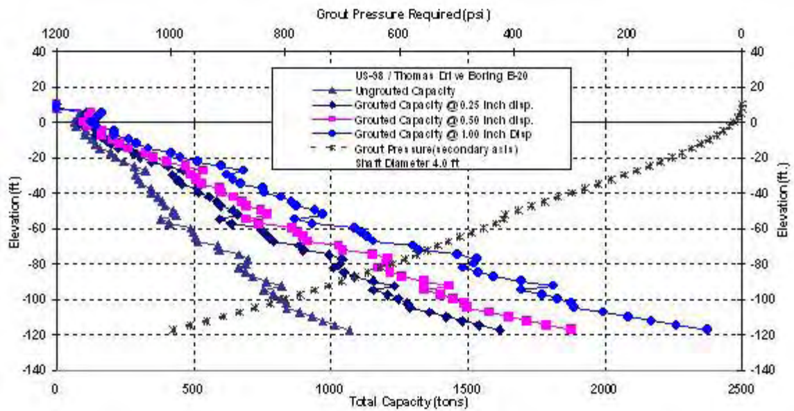
Figure C-206 US 98: B-20, 4ft Diameter
