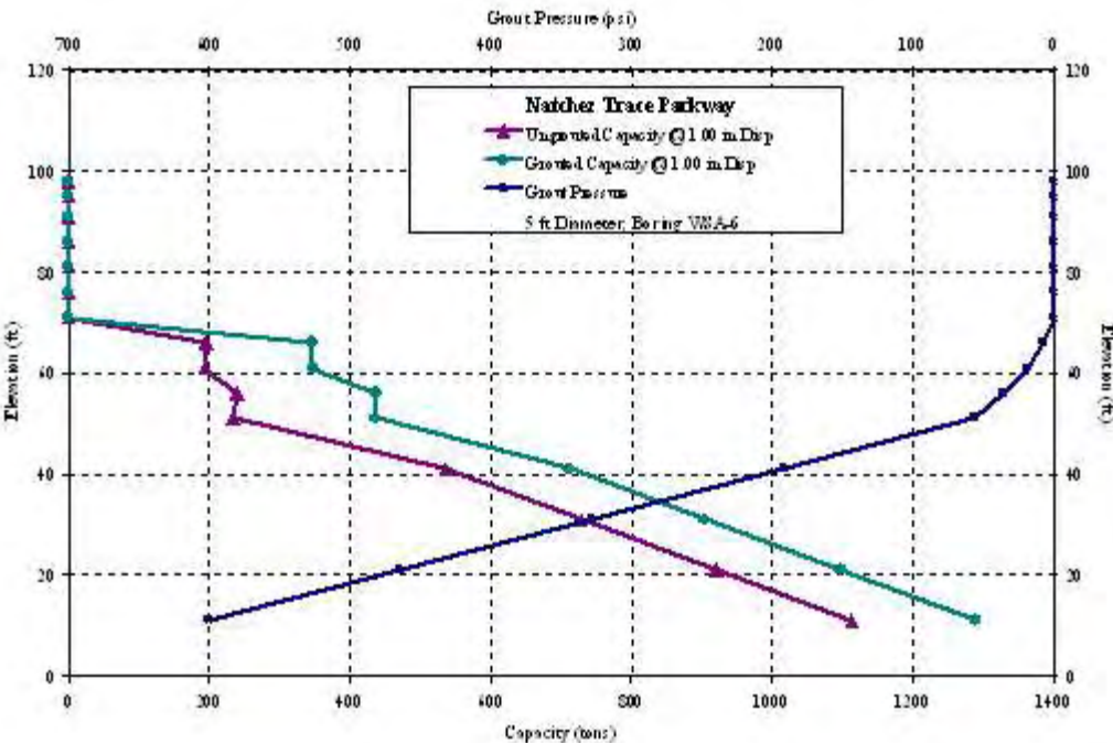
Figure C-64 Natchez Trace Pkwy: WSA-6, 5ft Diameter
