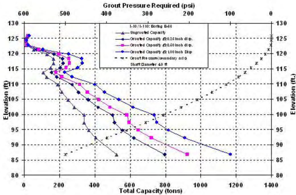
Figure C-56 I-10 / I-110: B-66, 4ft Diameter
