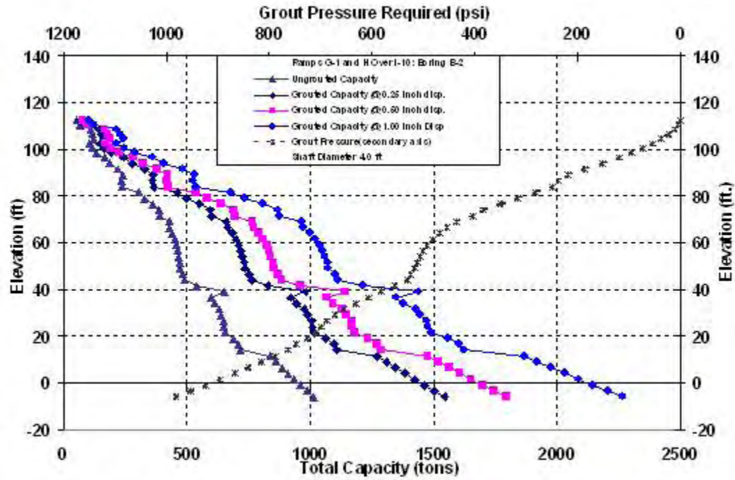
Figure C-35 I-10 / I-110: B-2, 4ft Diameter
