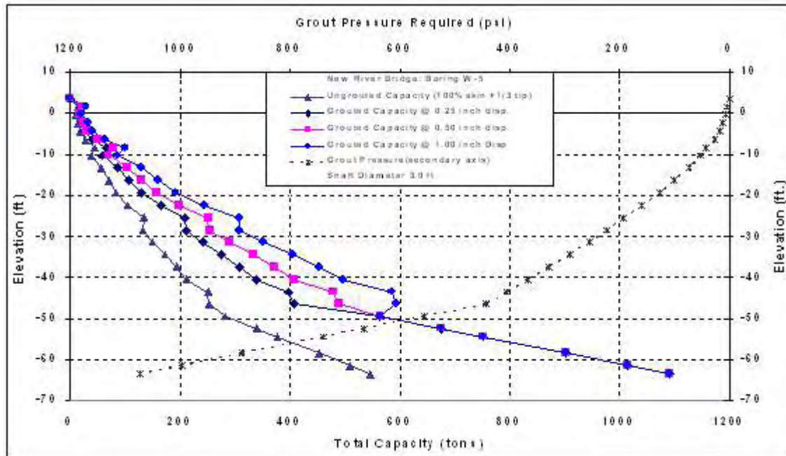
Figure C-131 New River Bridge: W-5, 3ft Diameter
