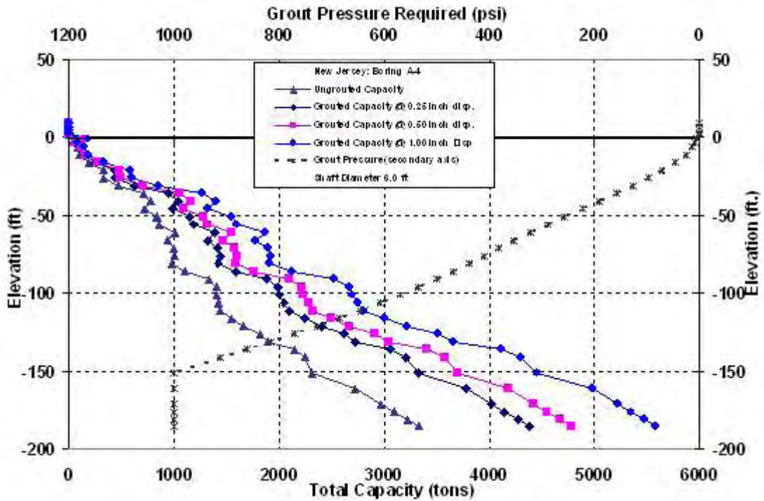
Figure C-170 Newark Legal Center: A-4, 6ft Diameter
