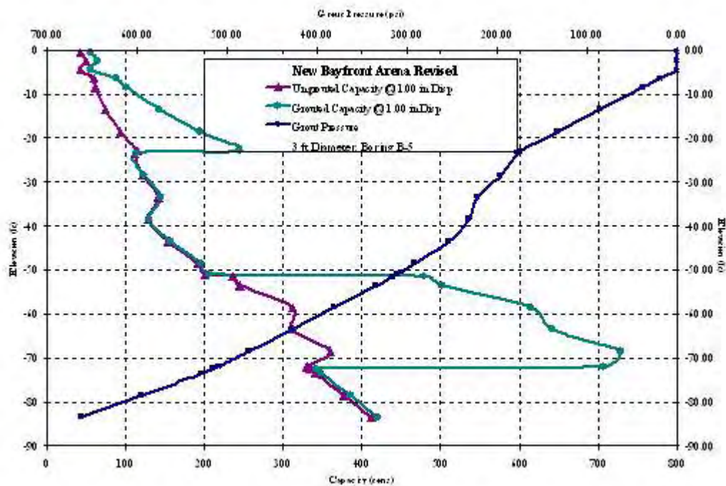
Figure C-88 New Bayfront Arena: B-5, 3ft Diameter
