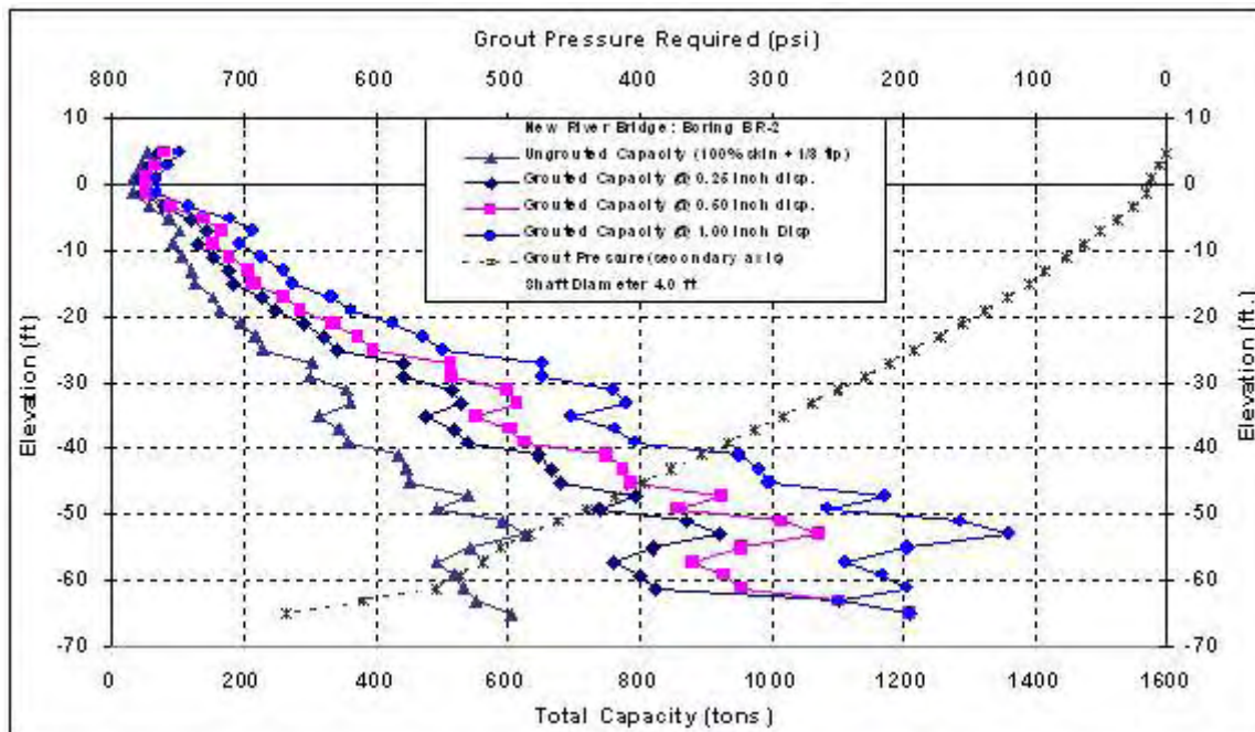
Figure C-112 New River Bridge: BR-2, 4ft Diameter
