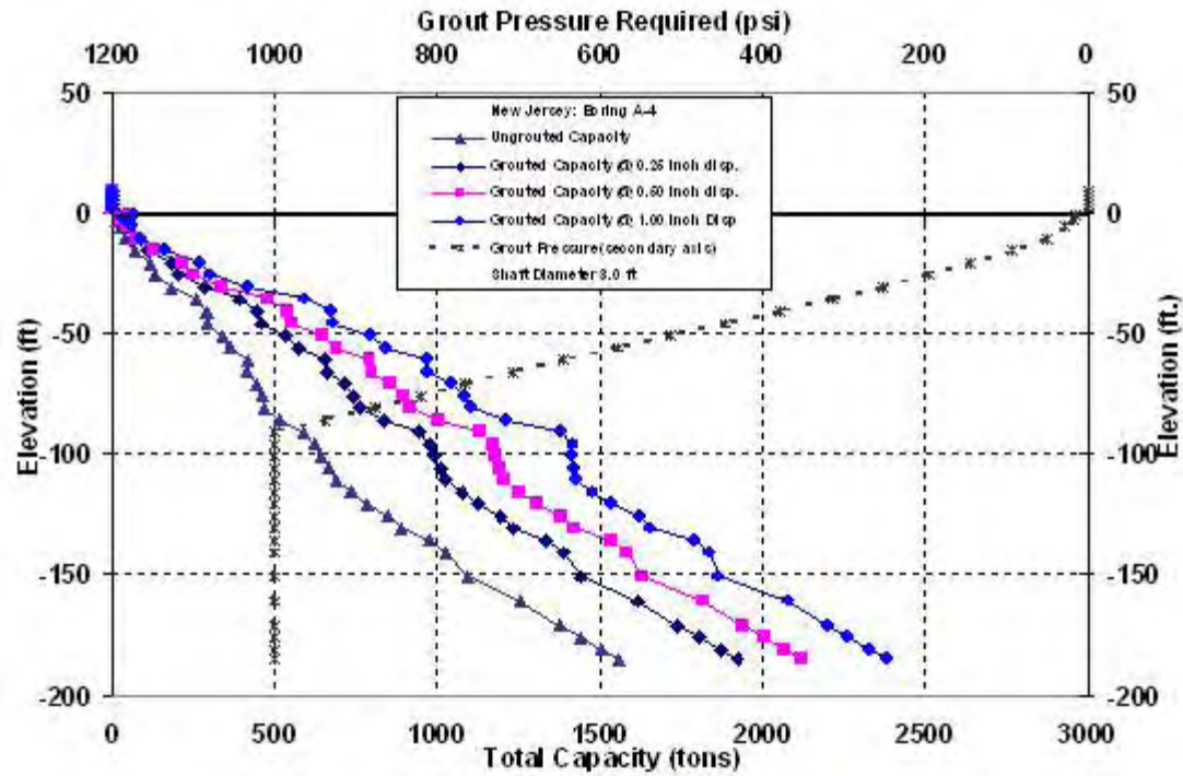
Figure C-167 Newark Legal Center: A-4, 3ft Diameter
