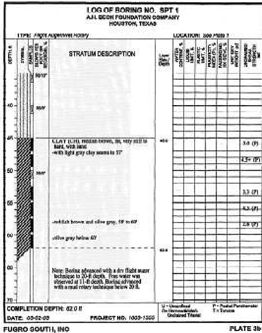
Figure B-44 TexDOT Demo: SPT 1 (page 2).
