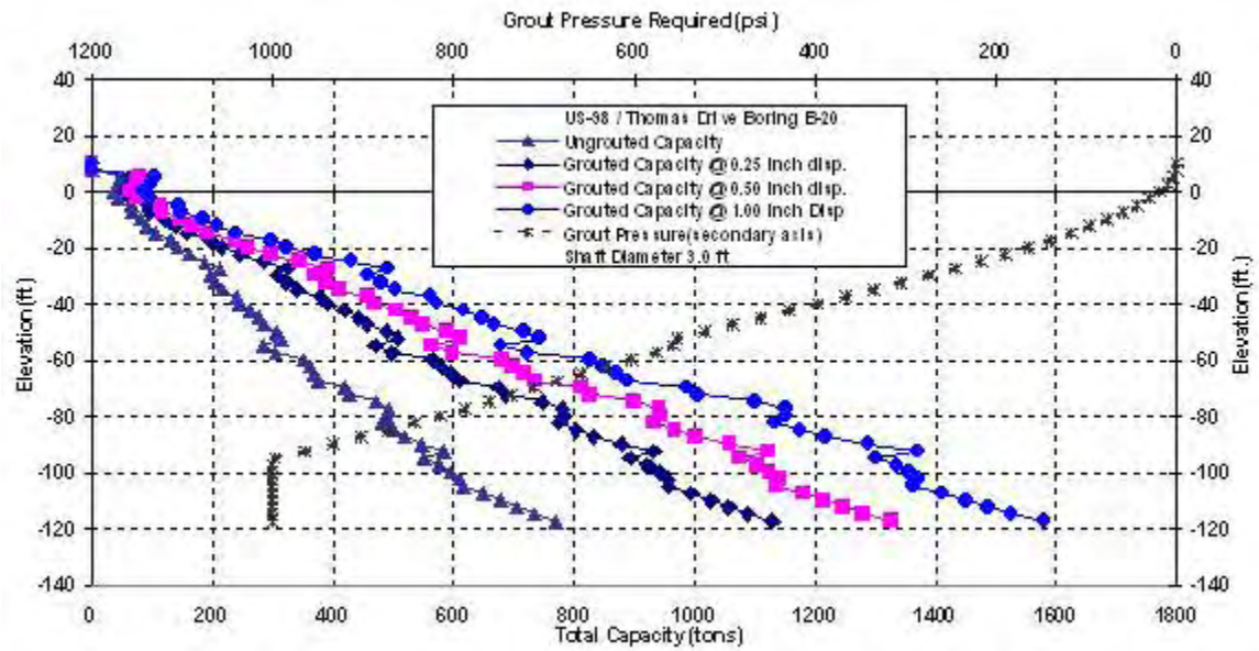
Figure C-205 US 98: B-20, 3ft Diameter
