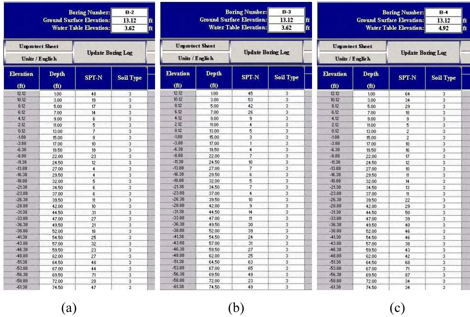
Figure B-51 PGA Blvd: (a) B-2, (b) B-3, and (c) B-4.
