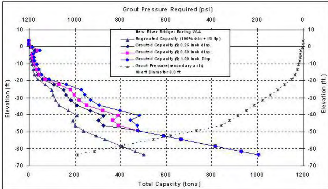
Figure C-127 New River Bridge: W-4, 3ft Diameter
