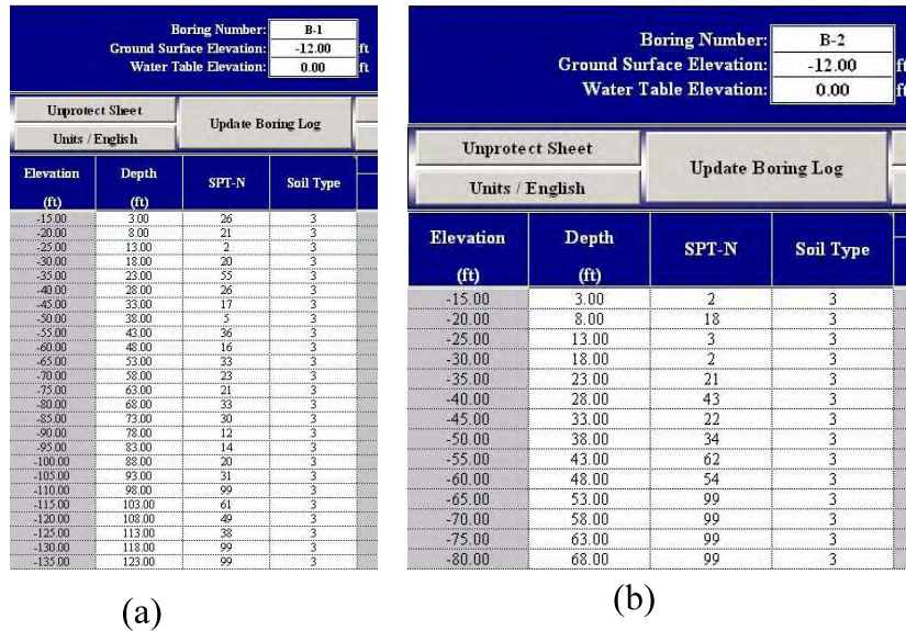
Figure B-52 Bayway Bridge: (a) B-1 and (b) B-2.
