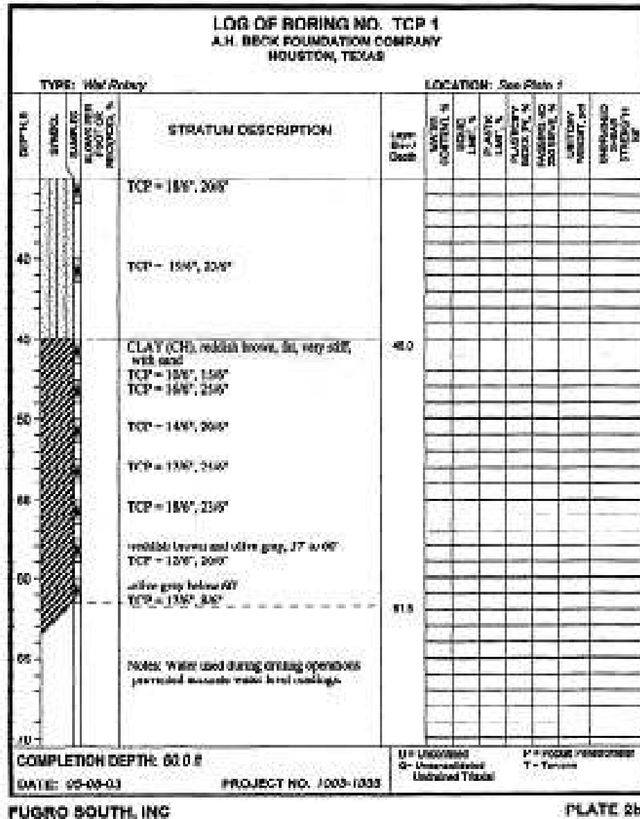
Figure B-46 TexDOT Demo: TCP 1 (page 2).
