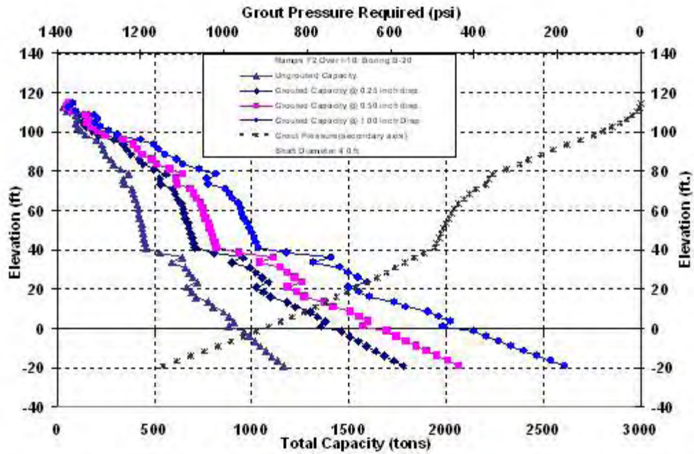
Figure C-47 I-10 / I-110: B-20, 4ft Diameter
