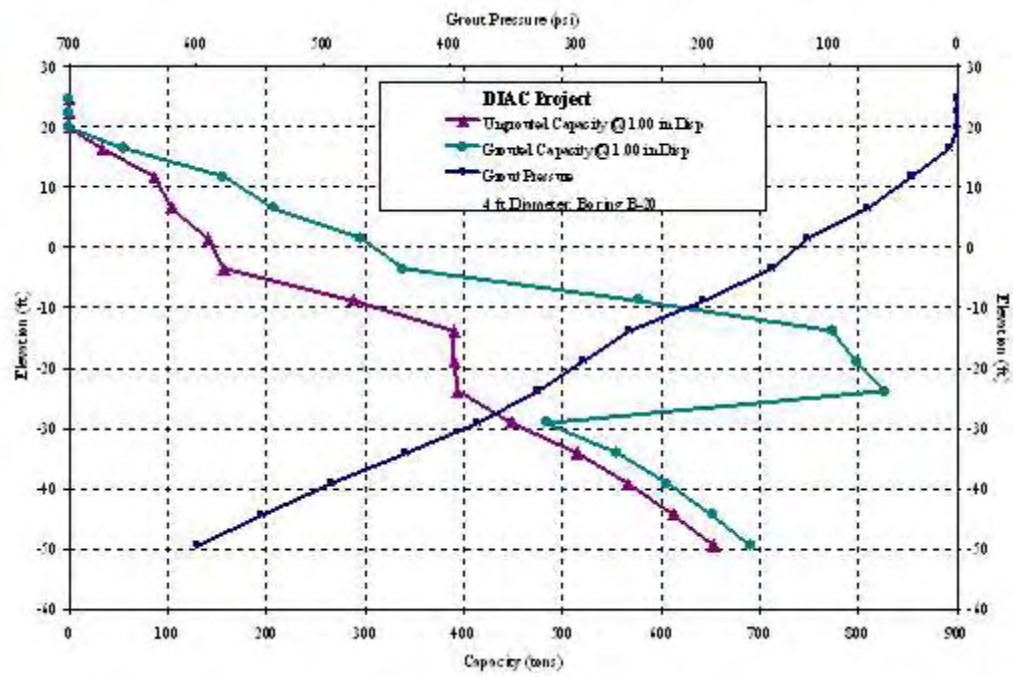
Figure C-19 Bolling Airforce Base: B-20, 4ft Diameter
