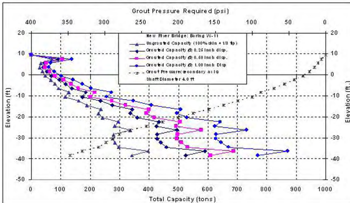
Figure C-156 New River Bridge: W-11, 4ft Diameter
