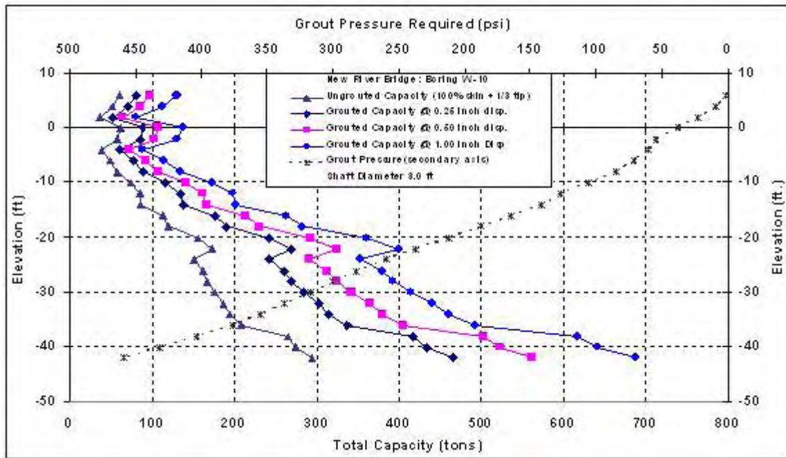
Figure C-151 New River Bridge: W-10, 3ft Diameter
