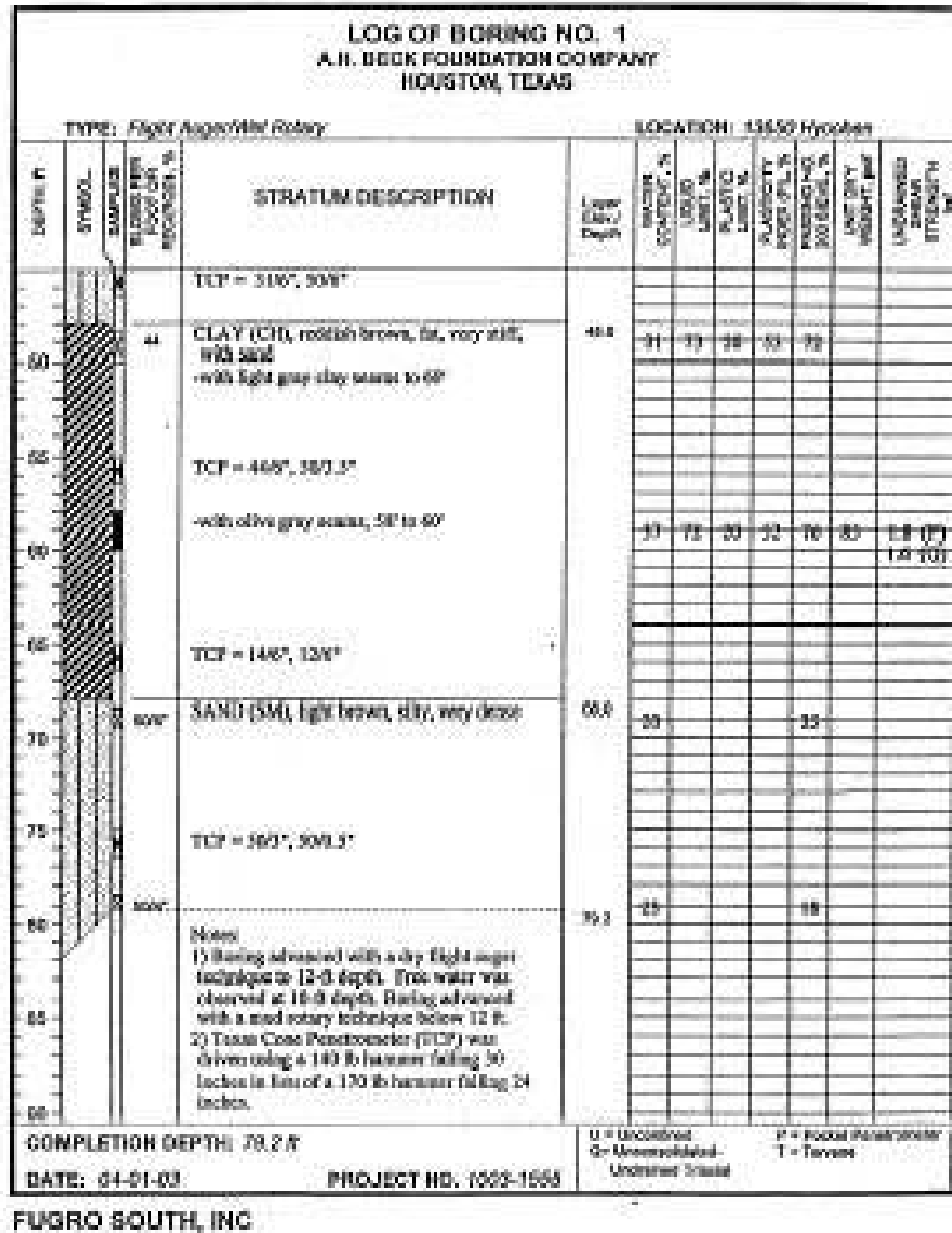
Figure B-42 TexDOT Demo: Boring No. 1 (page 2).
