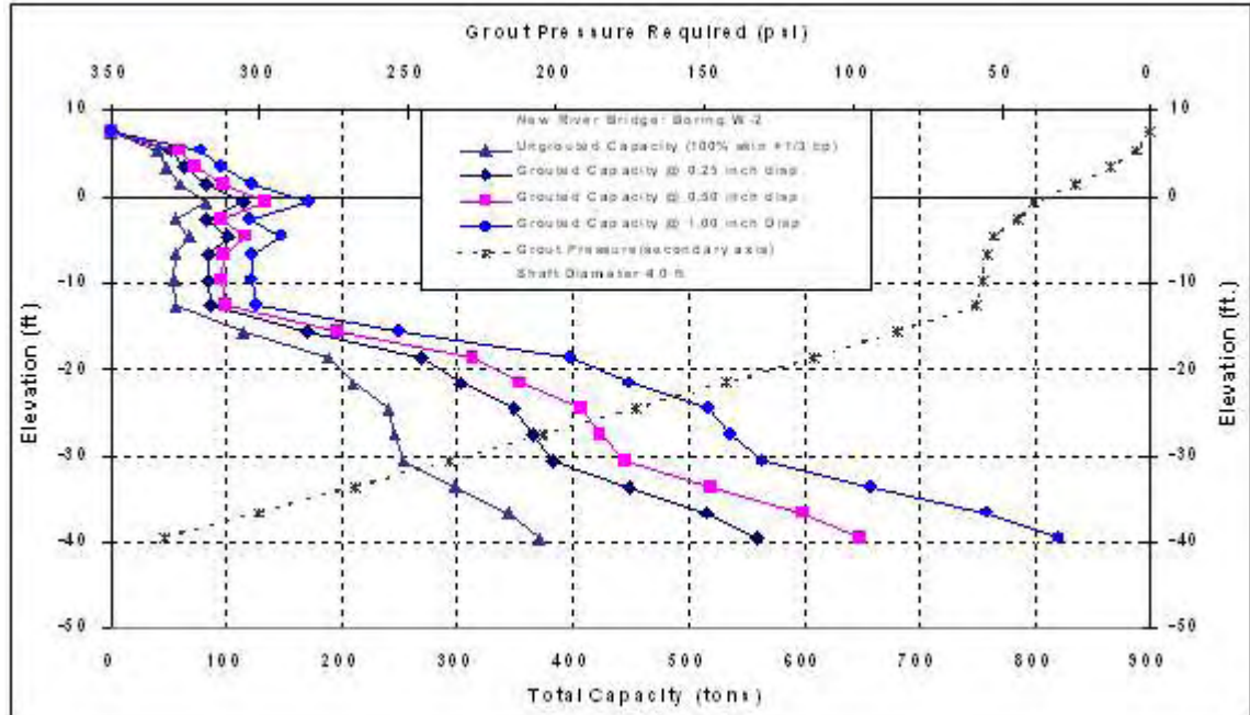
Figure C-120 New River Bridge: W-2, 4ft Diameter
