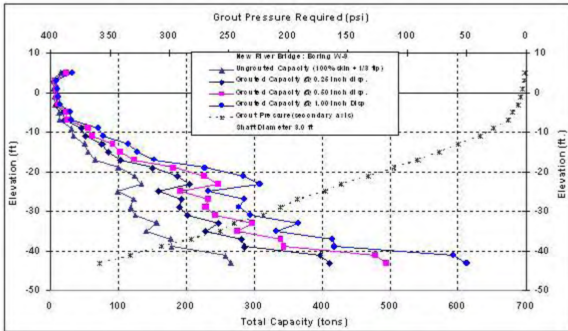
Figure C-147 New River Bridge: W-9, 3ft Diameter
