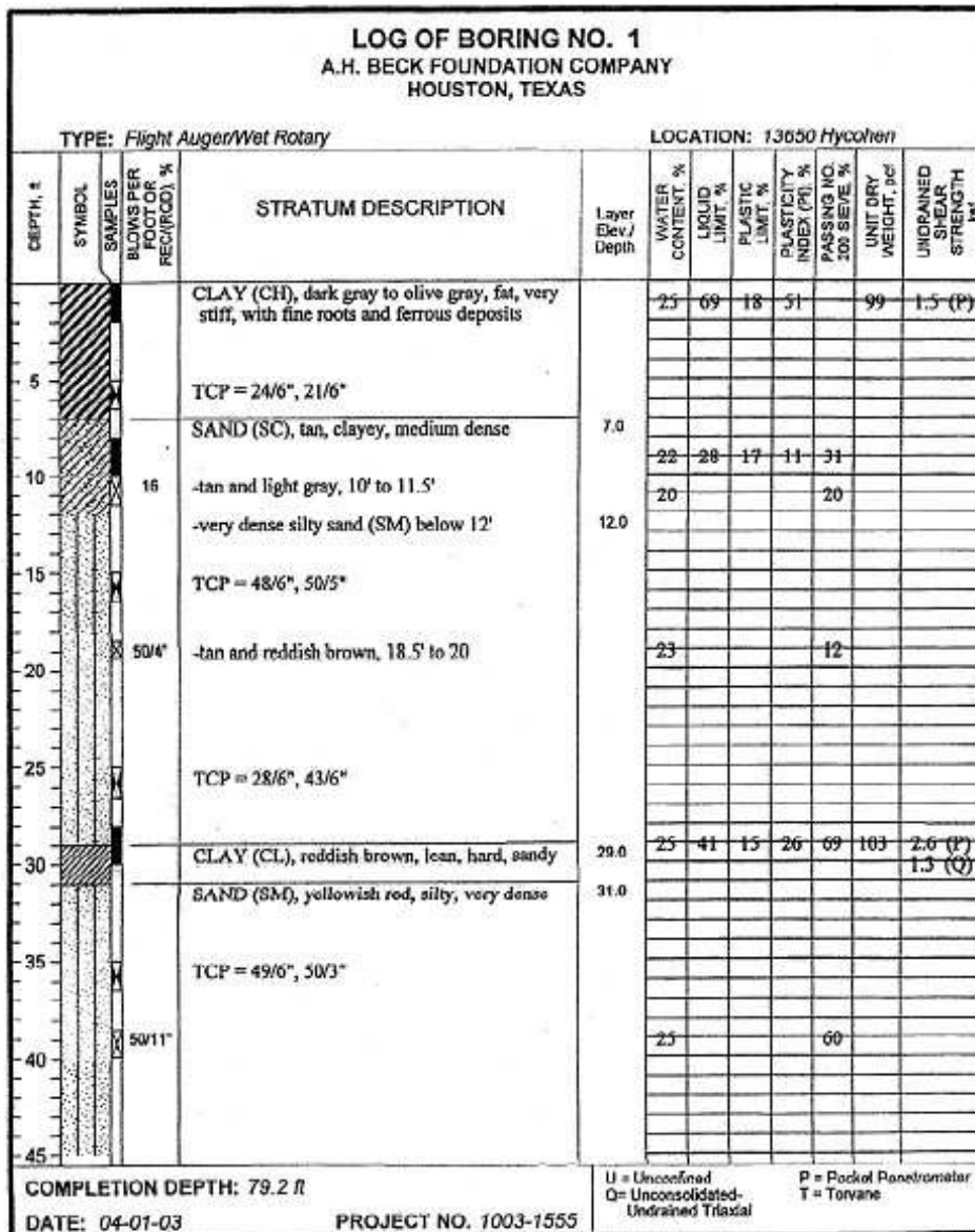
Figure B-41 TexDOT Demo: Boring No. 1 (page 1).
