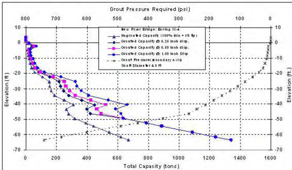
Figure C-128 New River Bridge: W-4, 4ft Diameter
