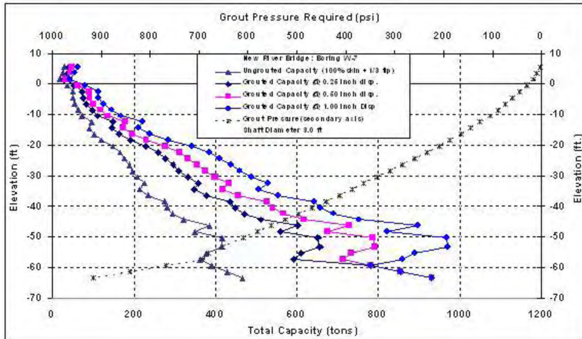
Figure C-139 New River Bridge: W-7, 3ft Diameter
