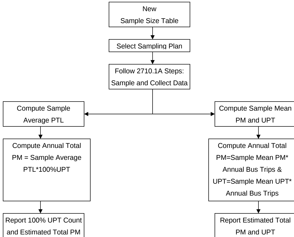
Figure 2. Flow Chart on Steps Following a New Sample Size Table
