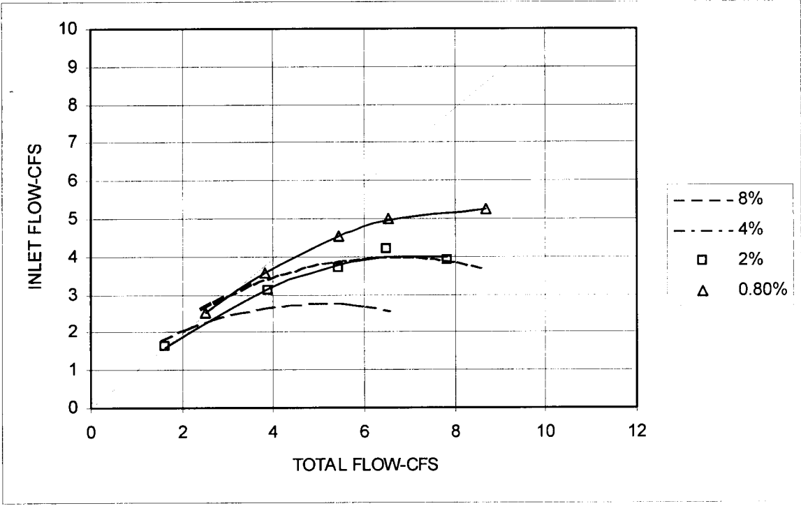
Figure 11: Full size performance curves for inlet Prototype inlet at 6% cross slope. Parameter is longitudinal slope.
