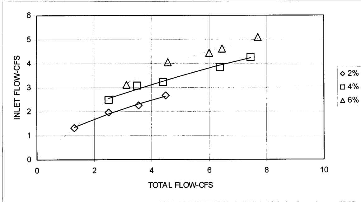
Figure 12 : Results of investigation for Type 5 inlet at 1% longitudinal slope, solid symbols represent data, solid lines represent empirical fits. Parameter is cross slope.
