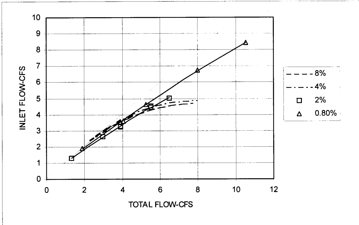
Figure 3: Full size performance curves for inlet Index 219 at 2% cross slope. Parameter is longitudinal slope.
