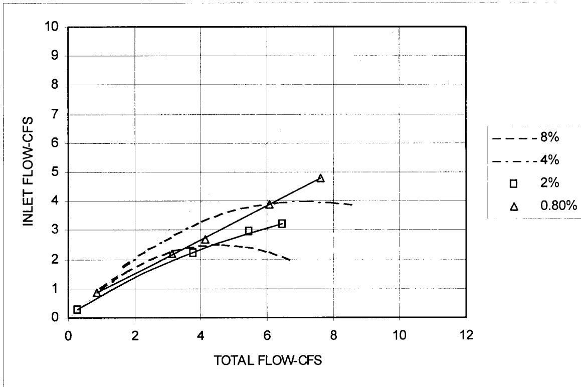
Figure 9: Full size performance curves for inlet Prototype inlet at 2% cross slope. Parameter is longitudinal slope.
