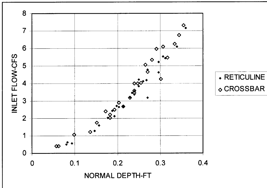
Figure 29: Correlation between normal depth upstream and inlet flow for both grating types. Measurement point upstream of bed transition.
