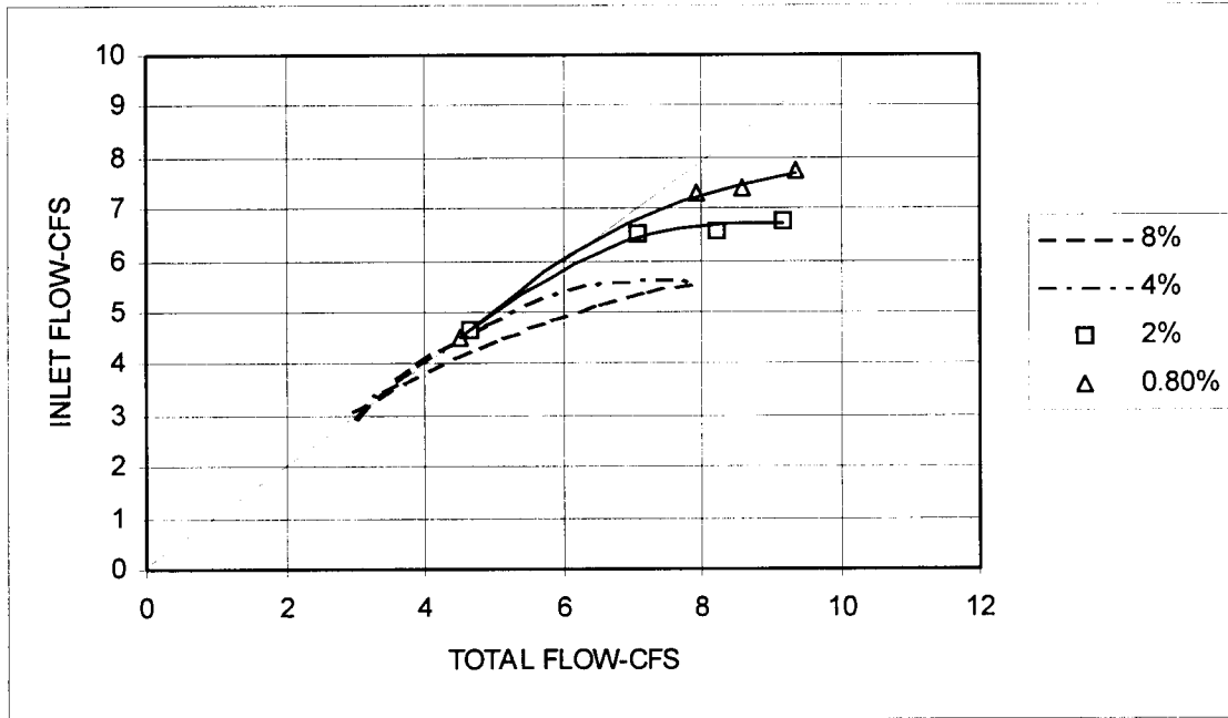
Figure 5: Full size performance curves for inlet Index 219 at 6% cross slope. Parameter is longitudinal slope.
