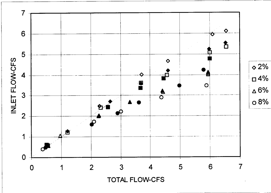
Figure 23: Collected data for model grated gutter inlet (Type S, Index 220). Longitudinal slope indicated at side bar, solid symbols denote data for reticuline grates, open symbols denote crossbar grates. Not to be used for design purposes.
