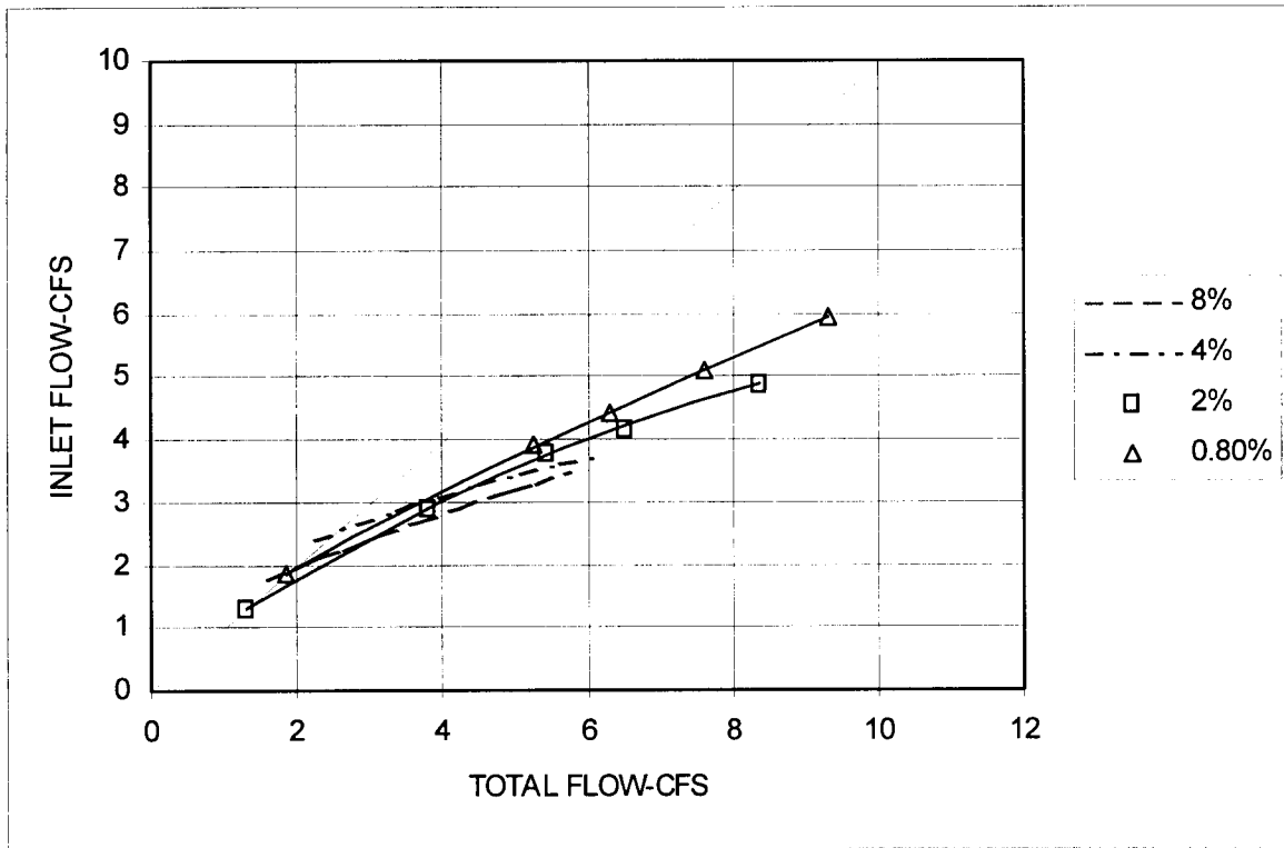
Figure 7: Full size performance curves for inlet Index 213 at 4% cross slope. Parameter is longitudinal slope.
