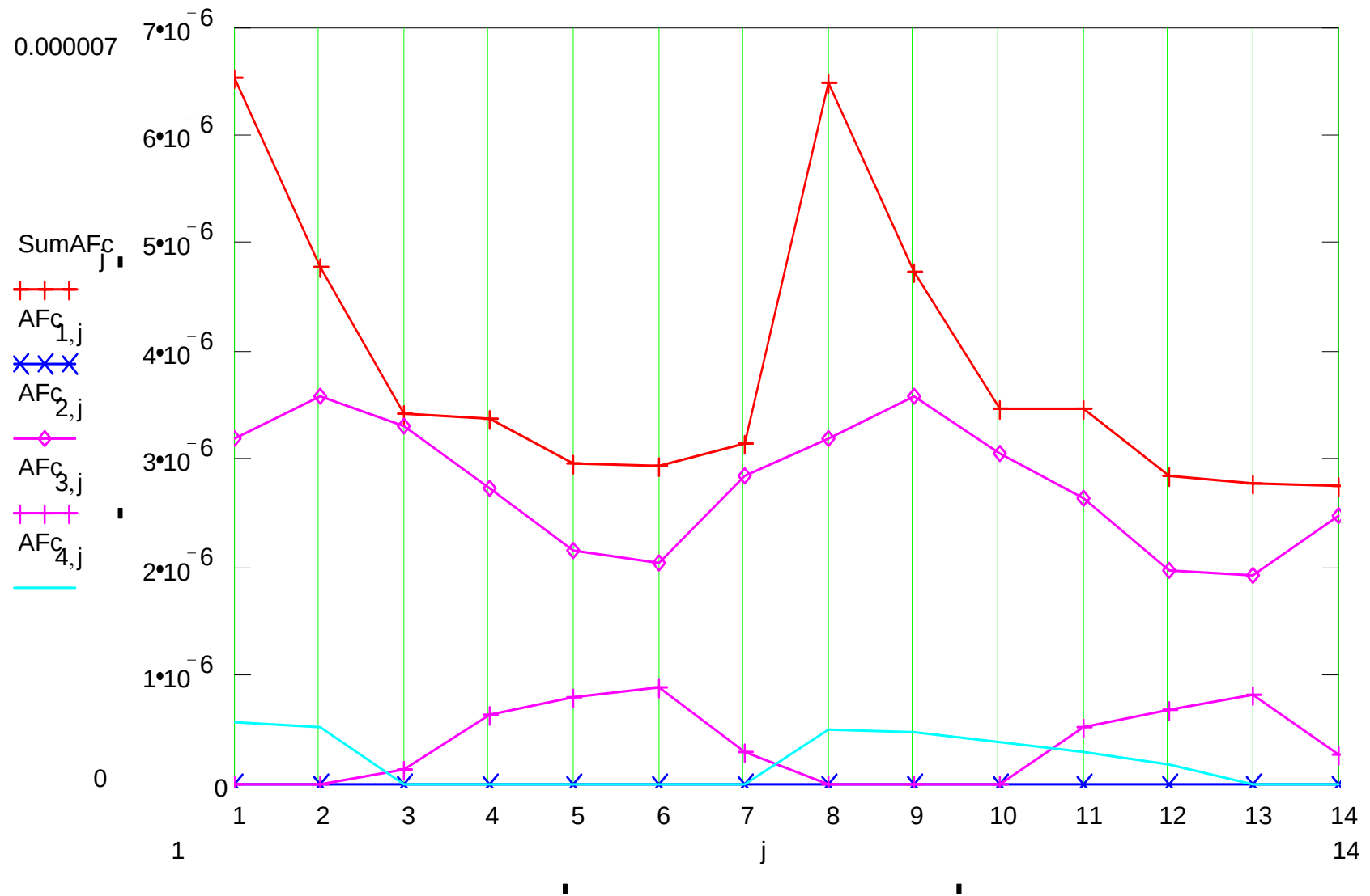
Figure 6. Annual Frequency of Collapse due to Downbound Vessel Group # 1, 2, 3, and 4
