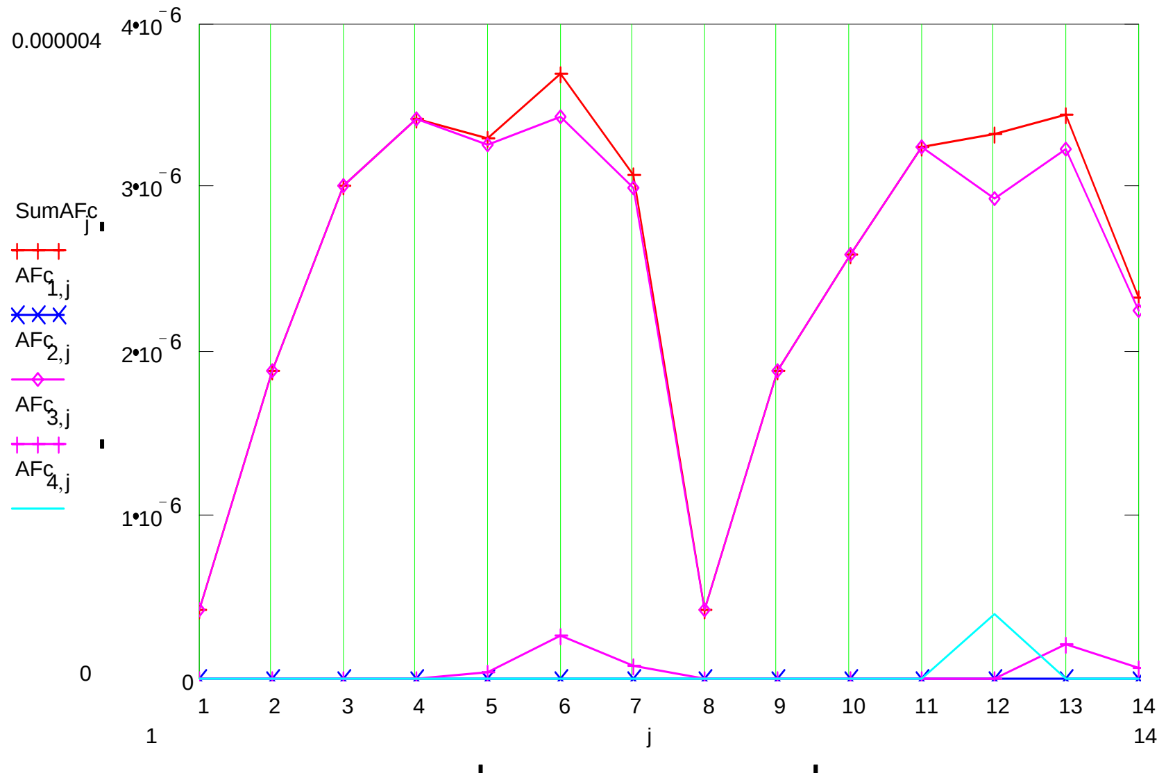
Figure 5. Annual Frequency of Collapse due to Upbound Vessel Group # 1, 2, 3, and 4
