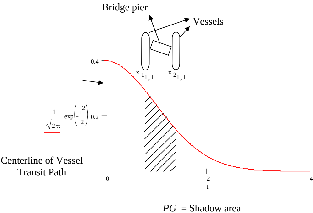
Figure 2. Geometric Probability of Pier Collision
