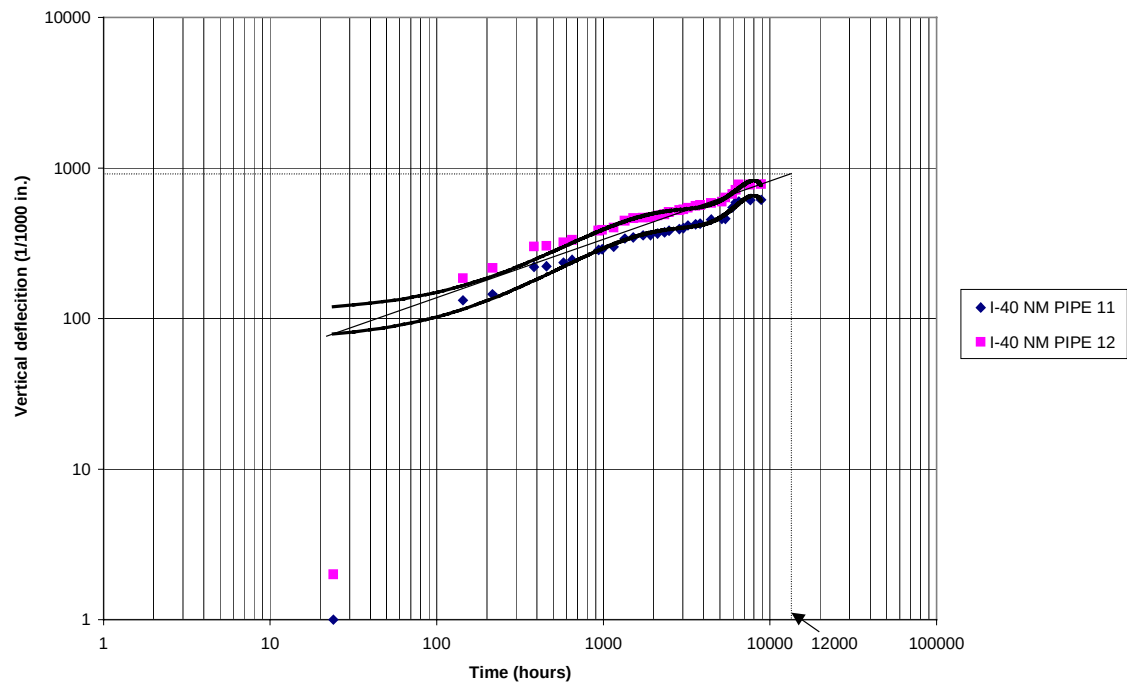
Fig. 4.15. Vertical change of diameter of Pipes 11 and 12
