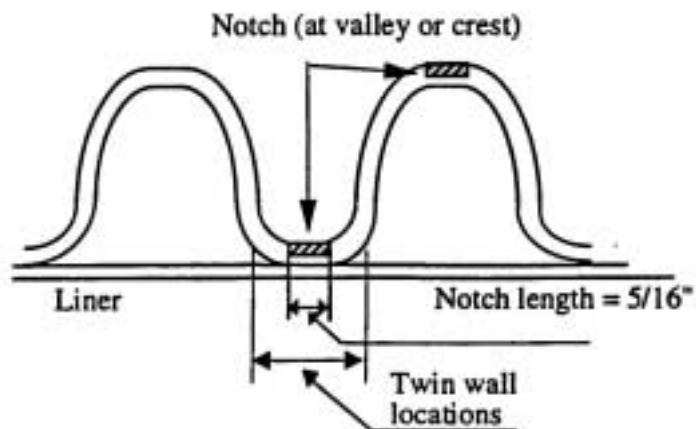
Fig. 3.2 (a) Cross-section of the notch
