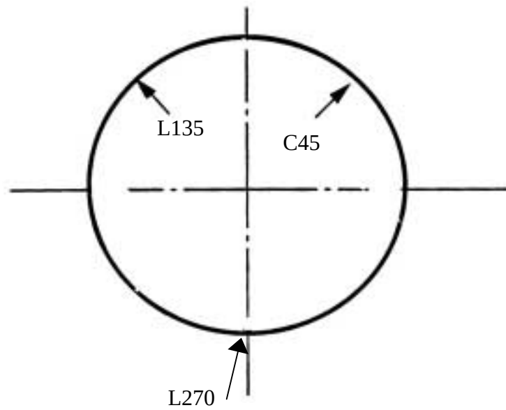
Fig. 3.8 Locations of strain gages
