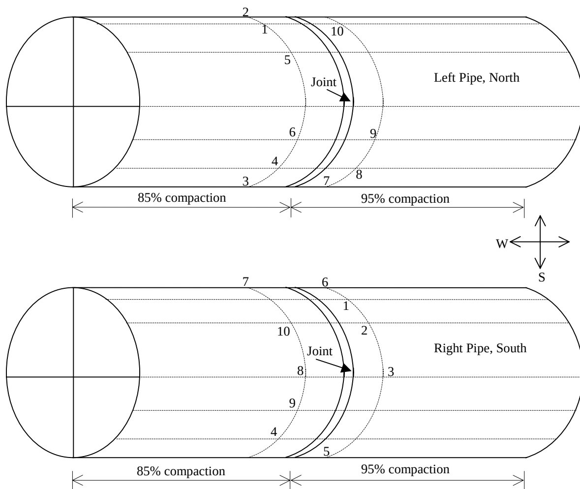
Figure 6.3 Position of the strain gages on the pipe
