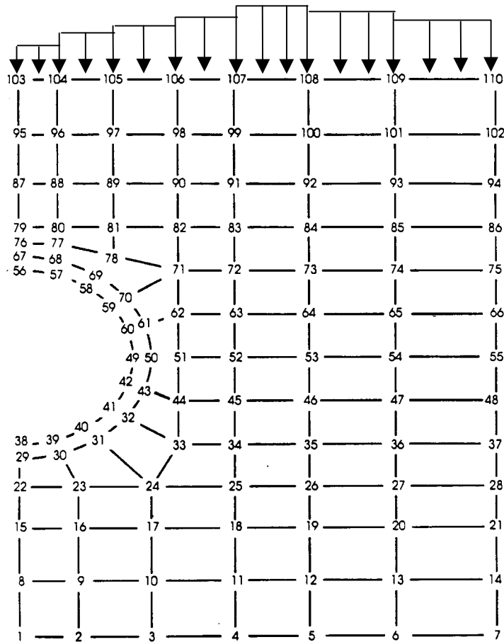
Figure 5.16 The distribution loading
