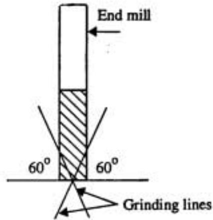
Fig. 3.2 (b) Preparation of ground tip end mill for notch
