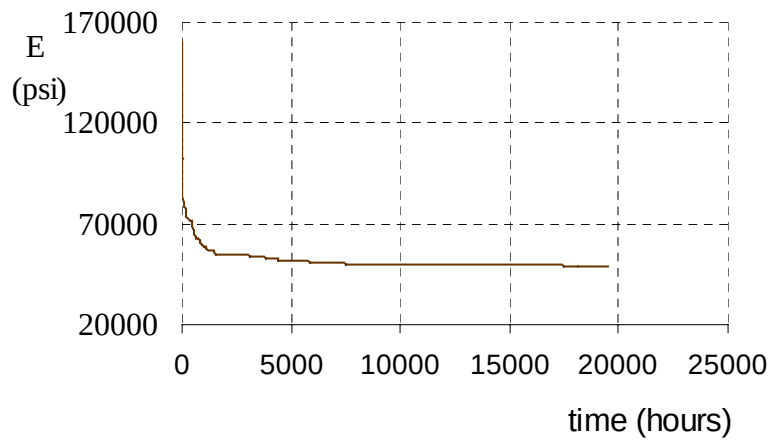
Figure 8.9 Master curve for type I (30 0 C)
