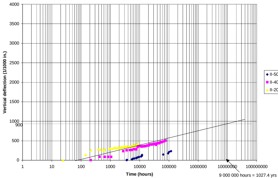
Fig. 5.12 Master curve, based on the Bi-directional method for Type II- Unnotched- M=1,900lb.
