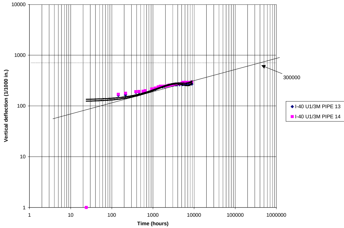
Fig. 4.5. Vertical change of diameter of Pipes 13 and 14
