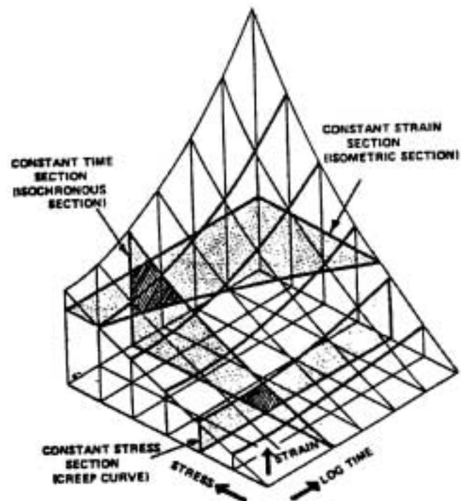
Fig. 2.3 Schematic of the viscoelastic behavior of polymers
