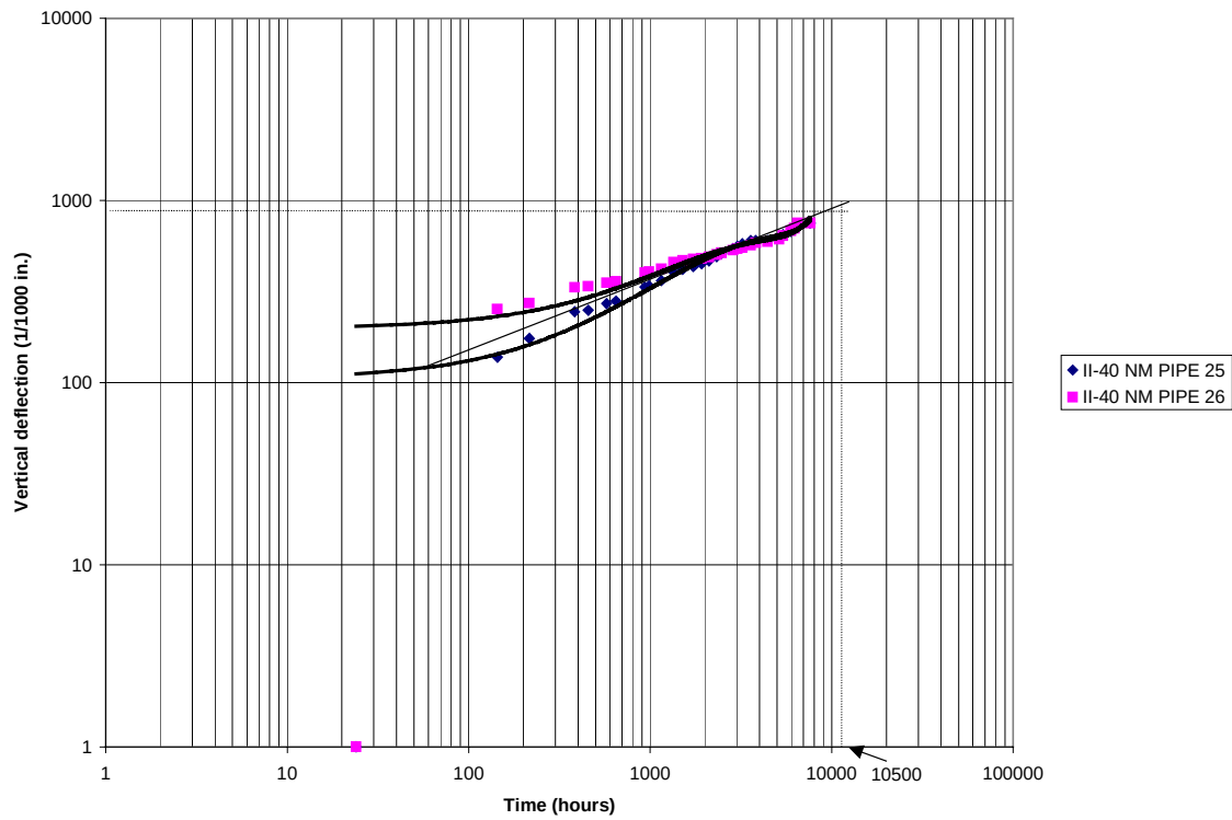
Fig. 4.18. Vertical change of diameter of Pipes 25 and 26
