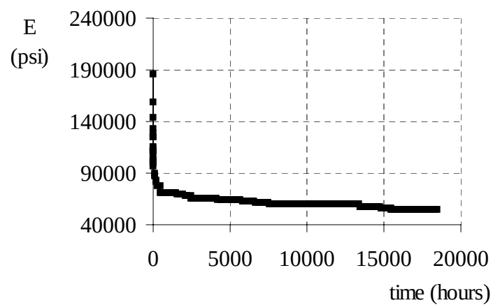
Figure 8.11 Master curve for type II (30 °C)
