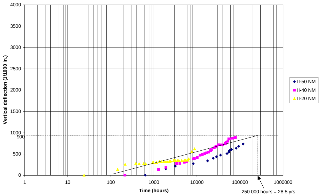
Fig. 5.10 Master curve, based on the Bi-directional method for Type II- Notched- M=5,600lb.
