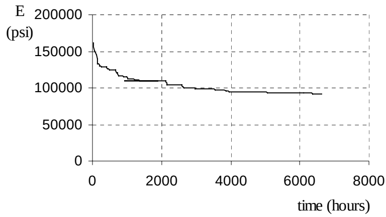
Figure 8.8 Master curve for type II (20 0 C)
