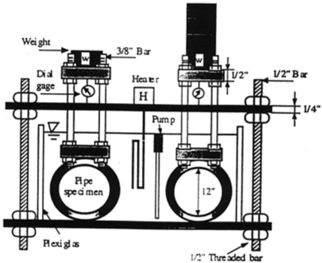
Figure 8.2 Parallel plate loading at super ambient temperature
