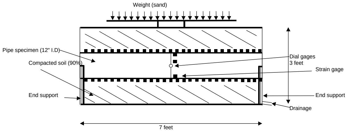
Fig. 3.10 Schematic of the test setup
