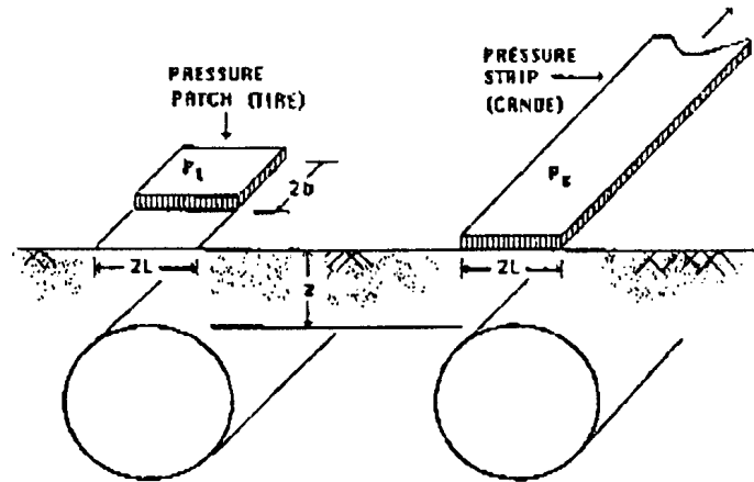
Fig. 5.13 H-truck loading and tire pressure distribution
