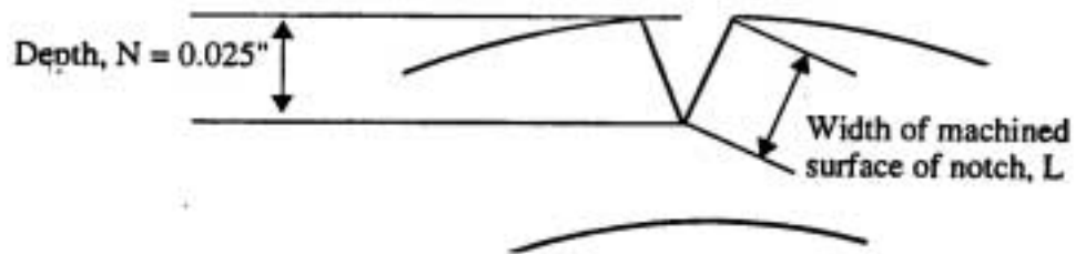
Fig. 3.2 (c) Notch Depth
