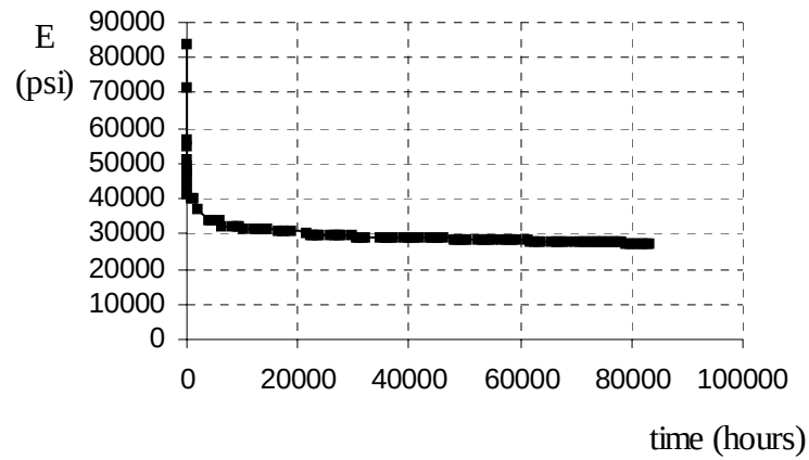
Figure 8.14 Master curve for type II (50 °C)
