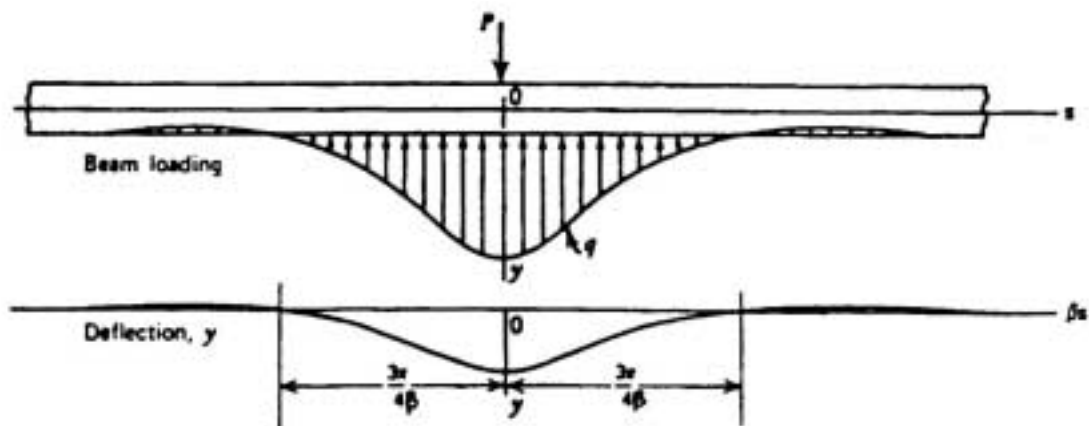
Fig. 3.3 Infinite pipe on elastic soil foundation
