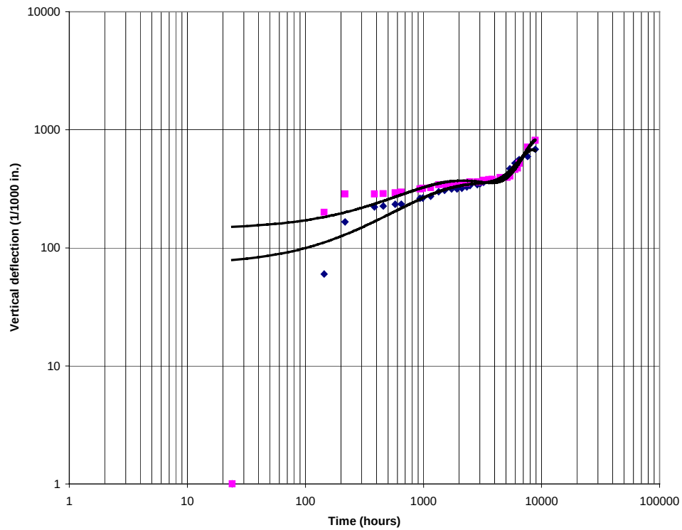
Fig. 4.10. Vertical change of diameter of Pipes 17 and 18
