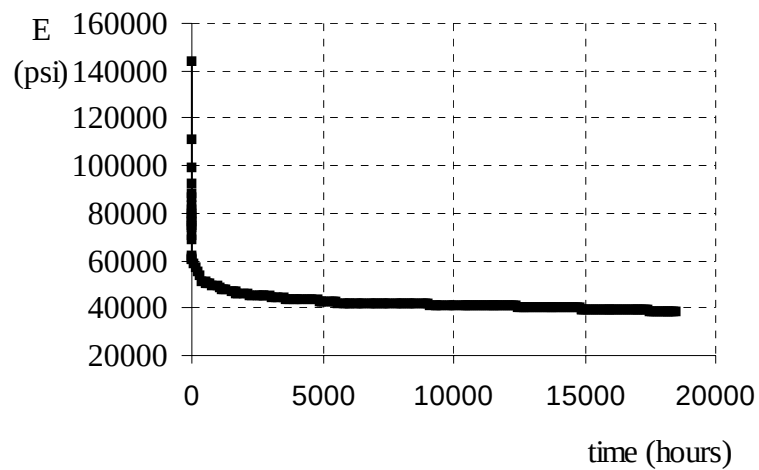
Figure 8.10 Master curve for type I (30 °C)
