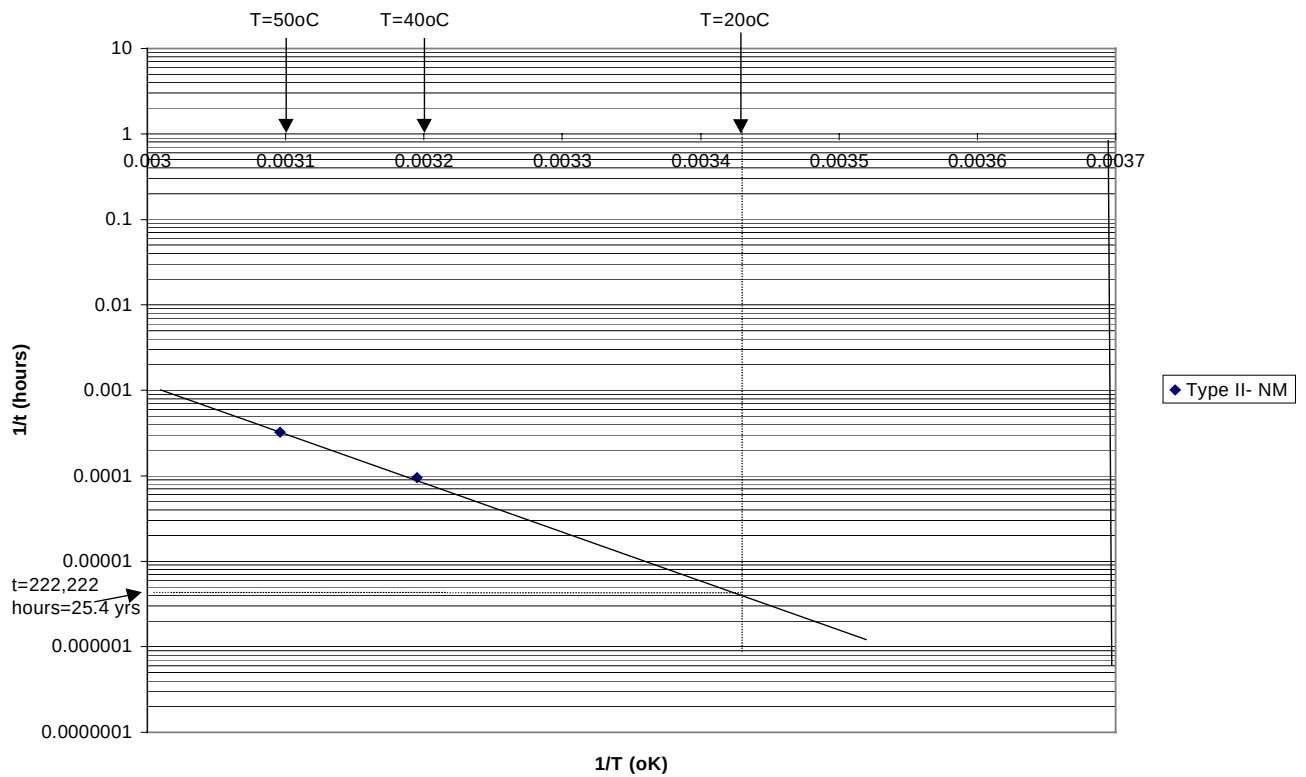
Fig. 5.4 Arrhenius plot for Type II-NM corresponding to 7.5% vertical change of diameter
