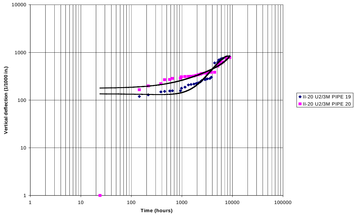
Fig. 4.9. Vertical change of diameter of Pipes 19 and 20
