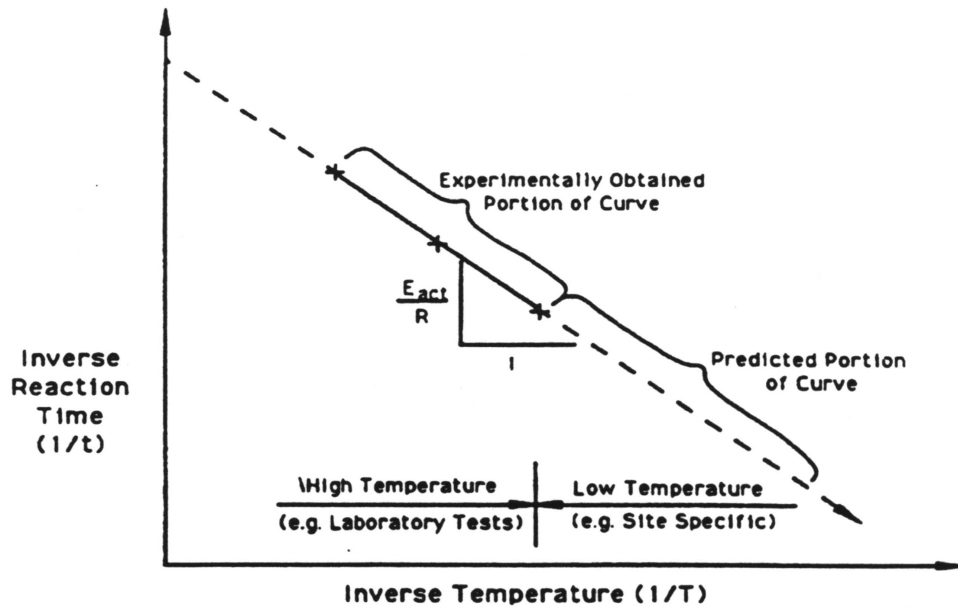
Fig. 2.8 Generalized Arrhenius plot, for a specified stress level, used for life prediction from super-ambient temperature experimental data
