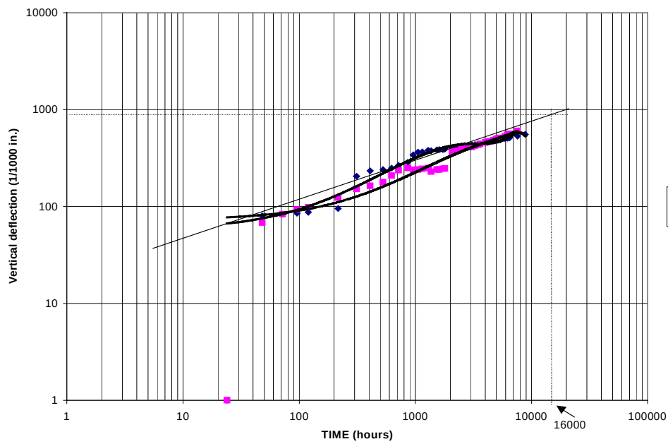
Fig. 4.12. Vertical change of diameter of Pipes 5 and 6
