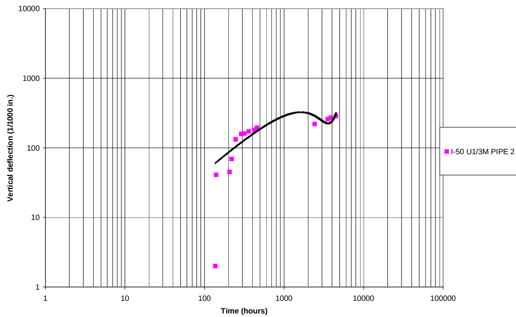
Fig. 4.6. Vertical change of diameter of Pipe 2
