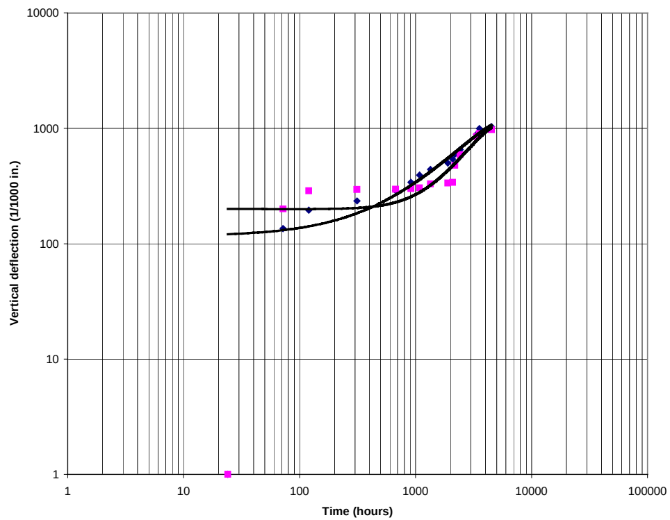
Fig. 4.16. Vertical change of diameter of Pipes 9 and 10
