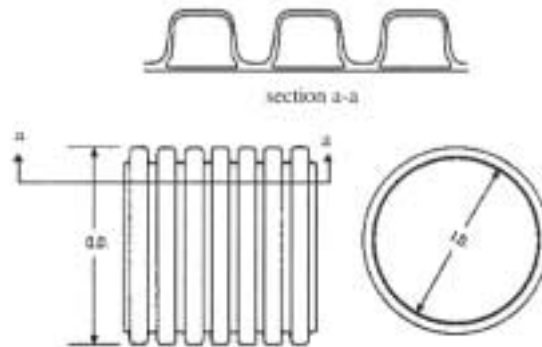
Fig. 3.1 Specimen geometry
