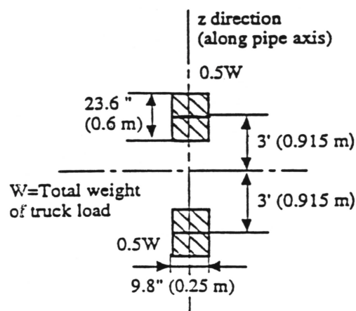
Fig. 3.4 ASHTO H20 highway loading configuration [AASHTO, 1992]
