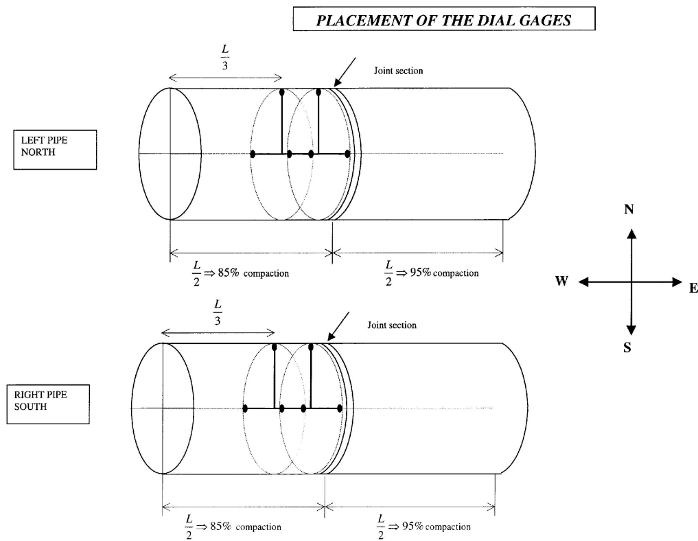
Figure 6.1 Position of dial gages
