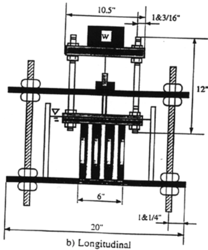
Figure 8.3 Schematic of creep test setup
