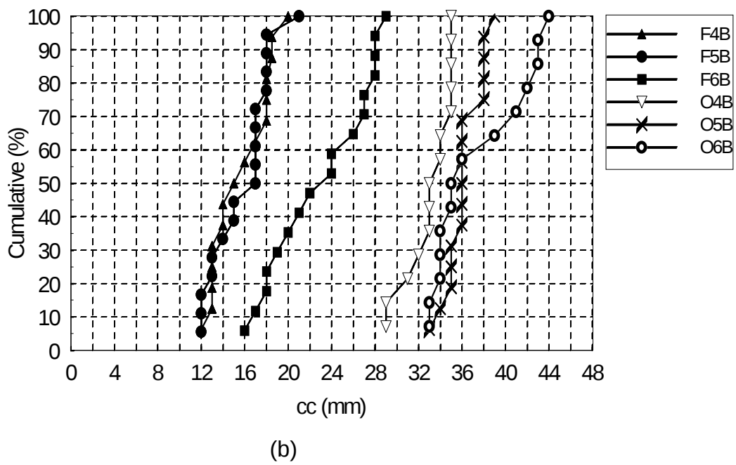
Figure 3. Cumulative percentage of steel wire cross sections examined in the cut edges vs concrete cover thickness (cc) for specimens corresponding to : a) set A and b) set B.
