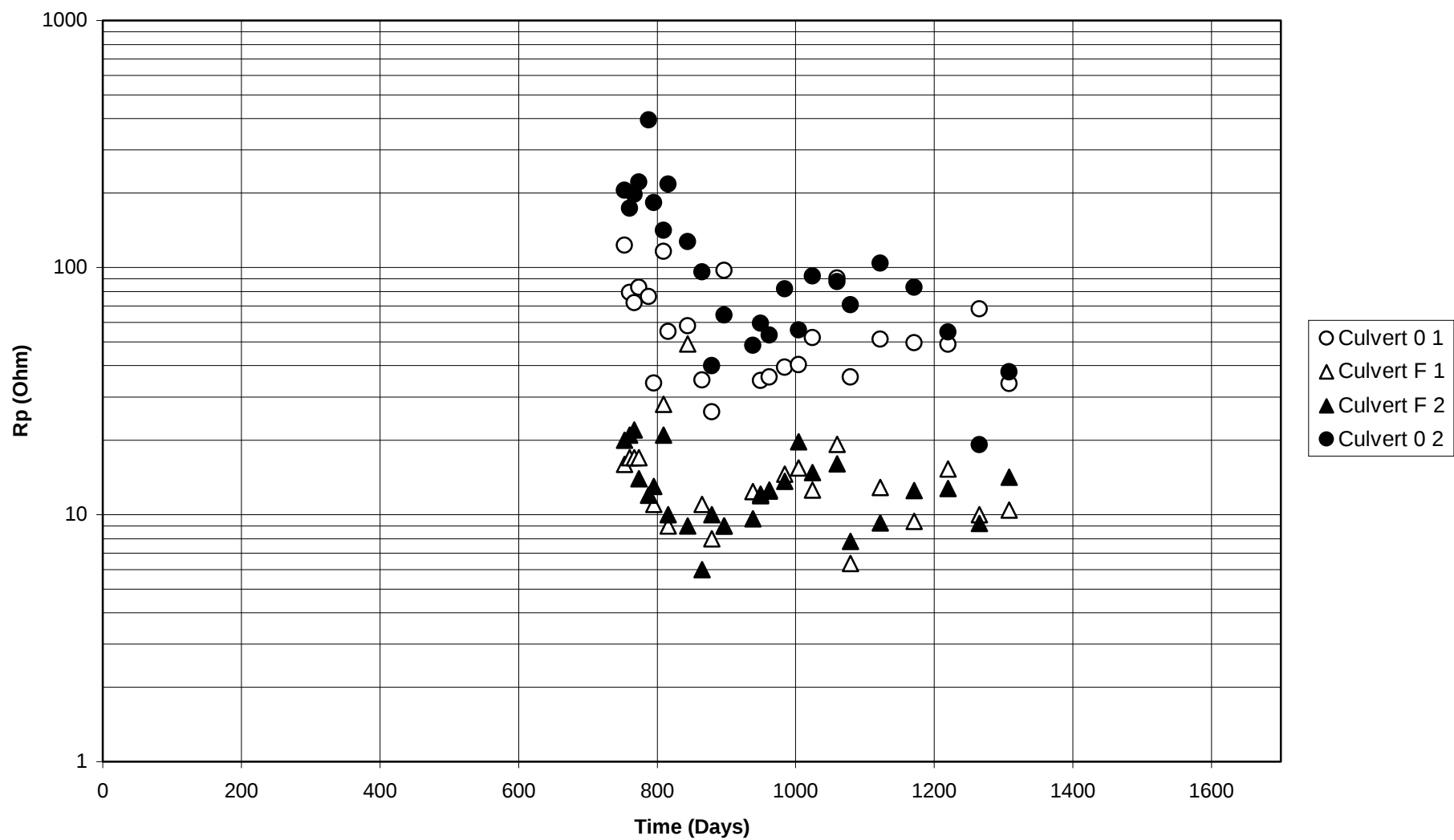
Figure 14 . Polarization resistance as a function of time for each pipe (solution resistance (solution resistance subtracted)).
