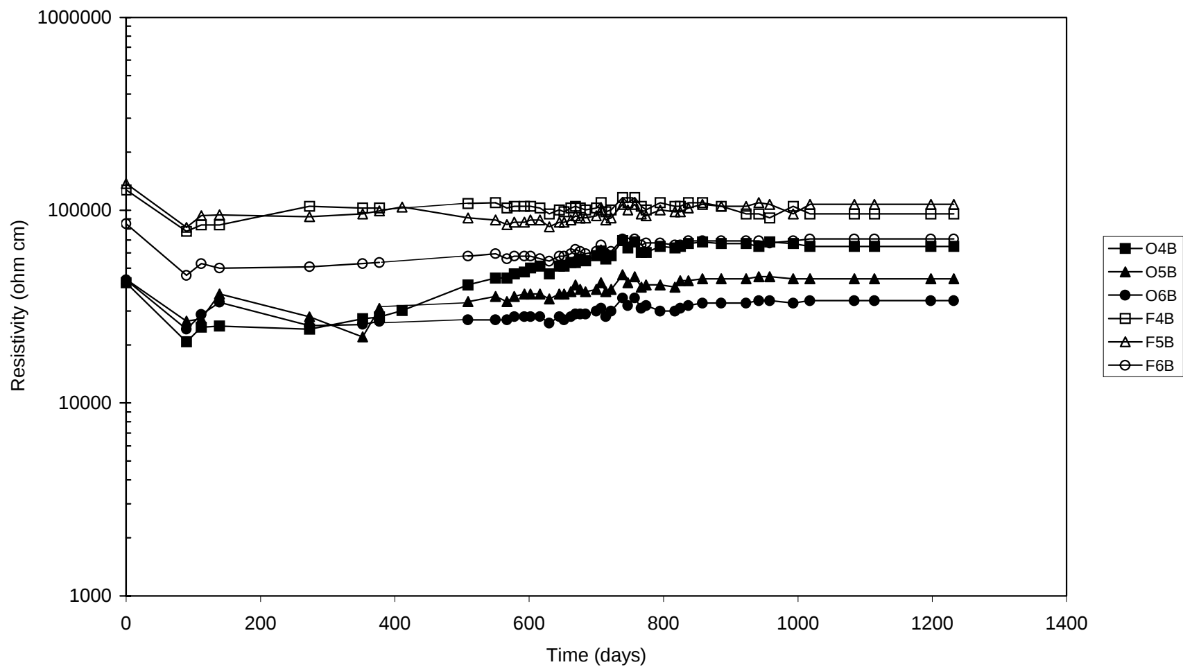
Figure 11. b. Evolution of concrete resistivity as a function of time for specimens of set B (permanently wet, with 8 months fresh water preconditioning before day 0).
