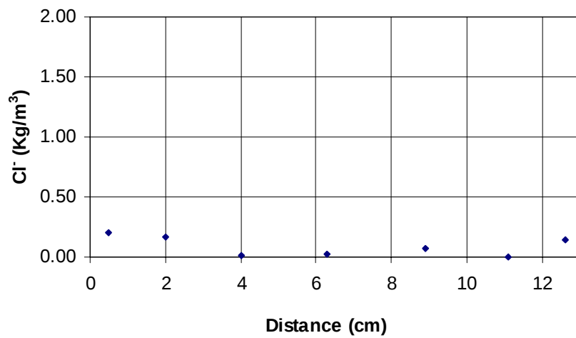
Chloride content vs distance from inside surface
