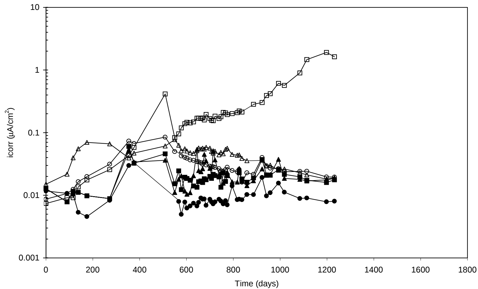
Figure 10. b. Evolution of nominal corrosion current density as a function of exposure time for specimens of set B.
