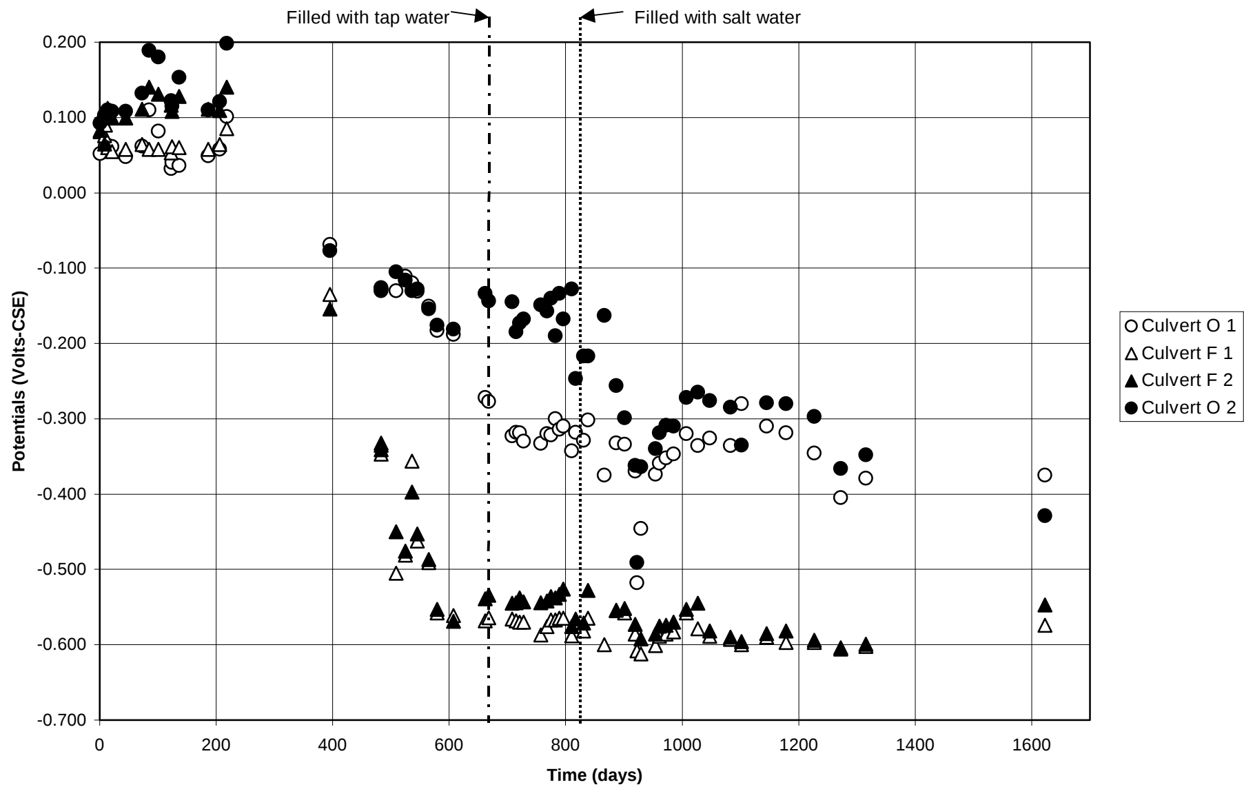
Figure 13. Potential as a function of time for reinforcement in each pipe.
