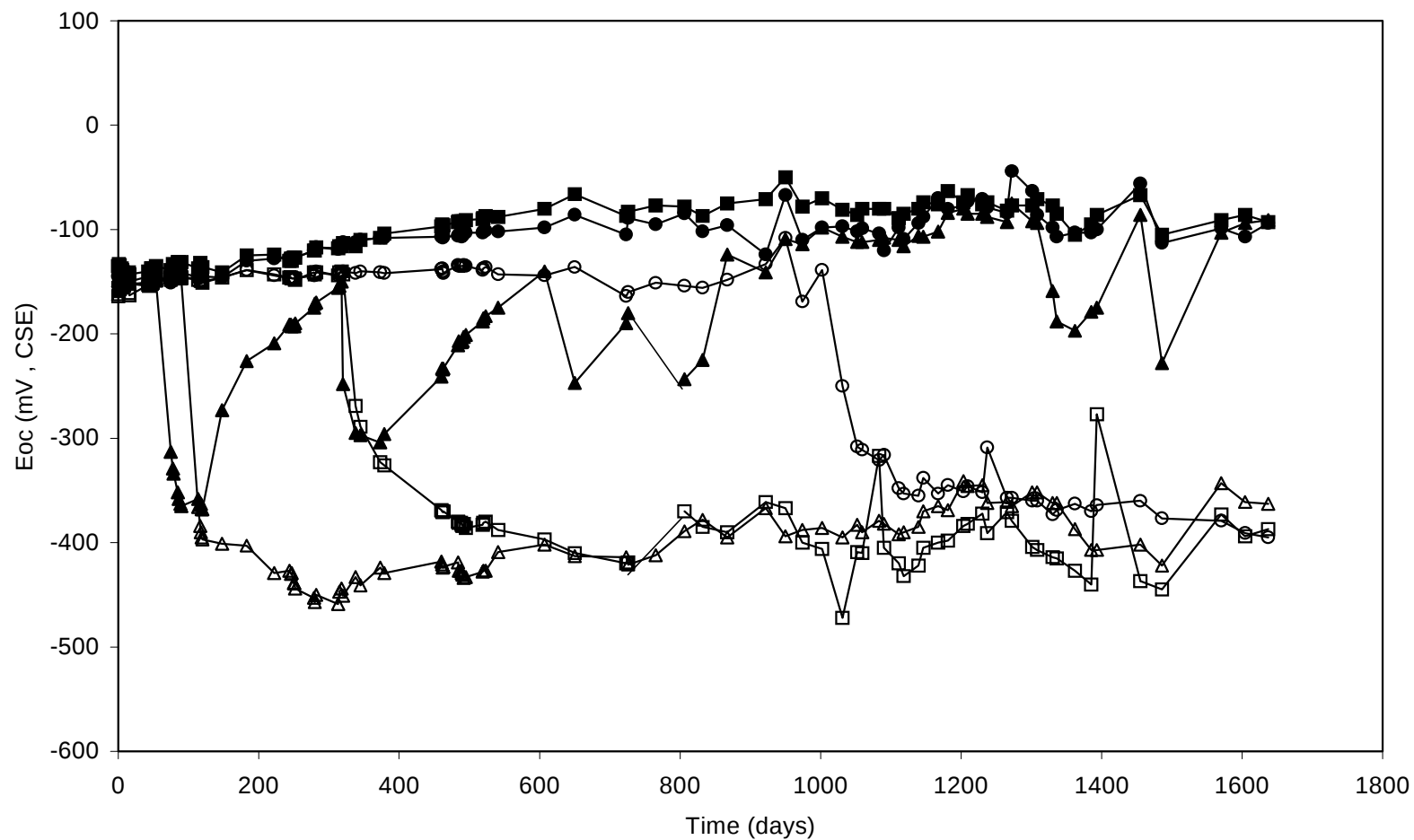
Figure 8. a. Open circuit potentials as a function of exposure time for specimens of set A (near the end of the wet cycle).
