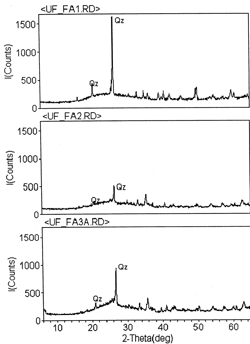
Figure 10: XRD Patterns for As-Received Ashes
