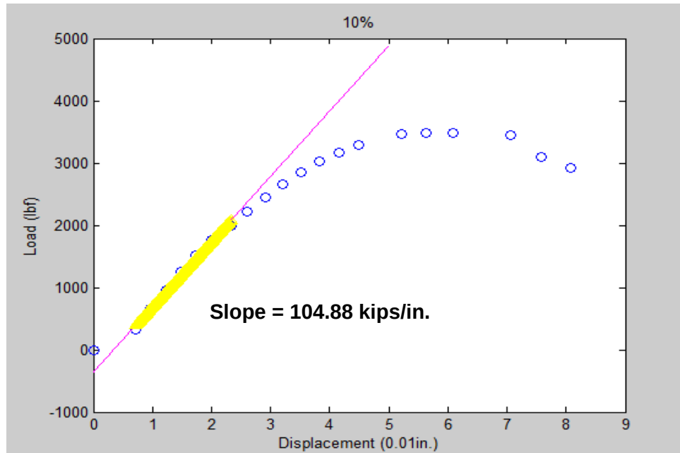
Figure A.2: IDT 'stiffness' for the mixture with 10% BA
