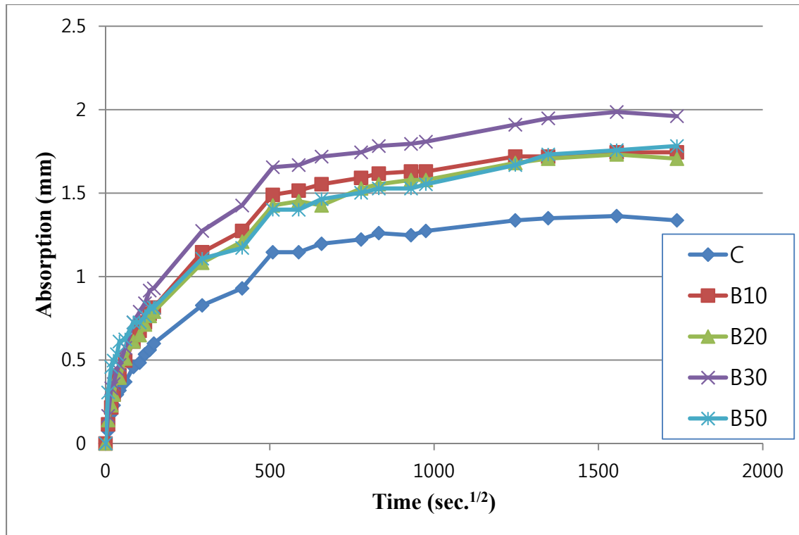
Figure 5.7: Absorption capacity for concrete specimens with time
