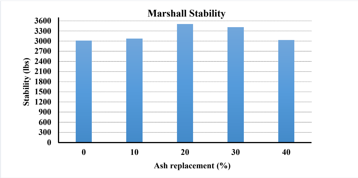
Figure 6.5: Marshall stability result
