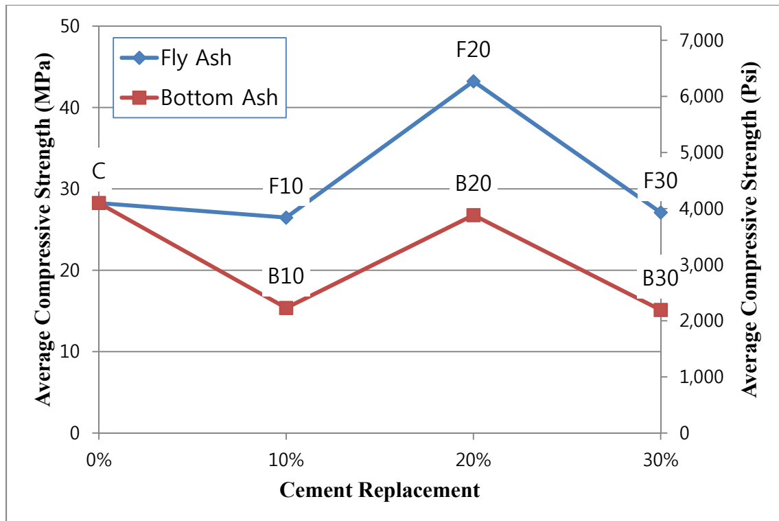
Figure 4.7: Average compressive strength measured at 28 days for all cement paste cylinders
