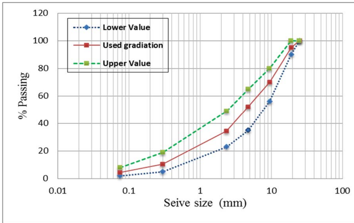
Figure 6.2: Gradation curve of used aggregate and limits
