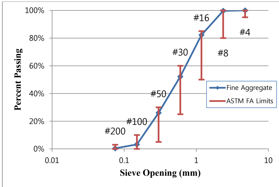
Figure 5.1: Gradation curve for fine aggregate (ASTM C33)
