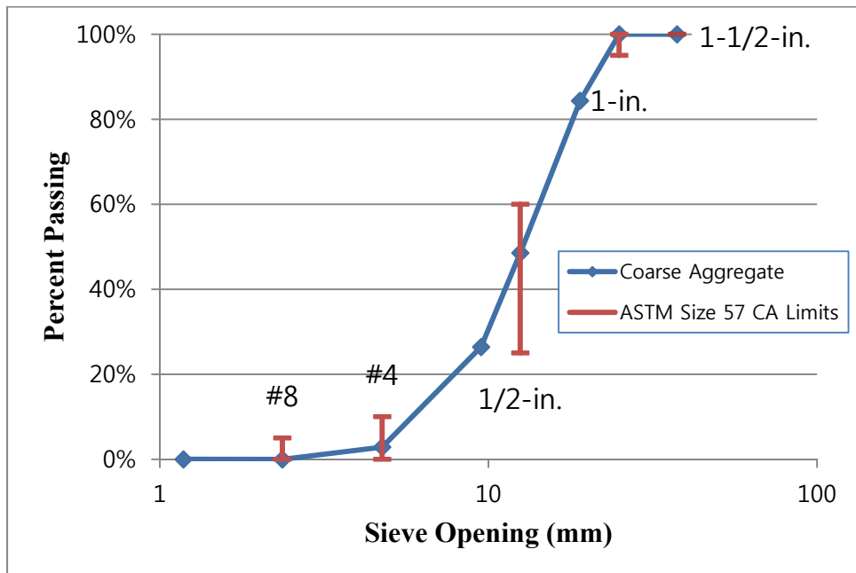
Figure 5.2: Gradation curve for coarse aggregate (ASTM C 136)
