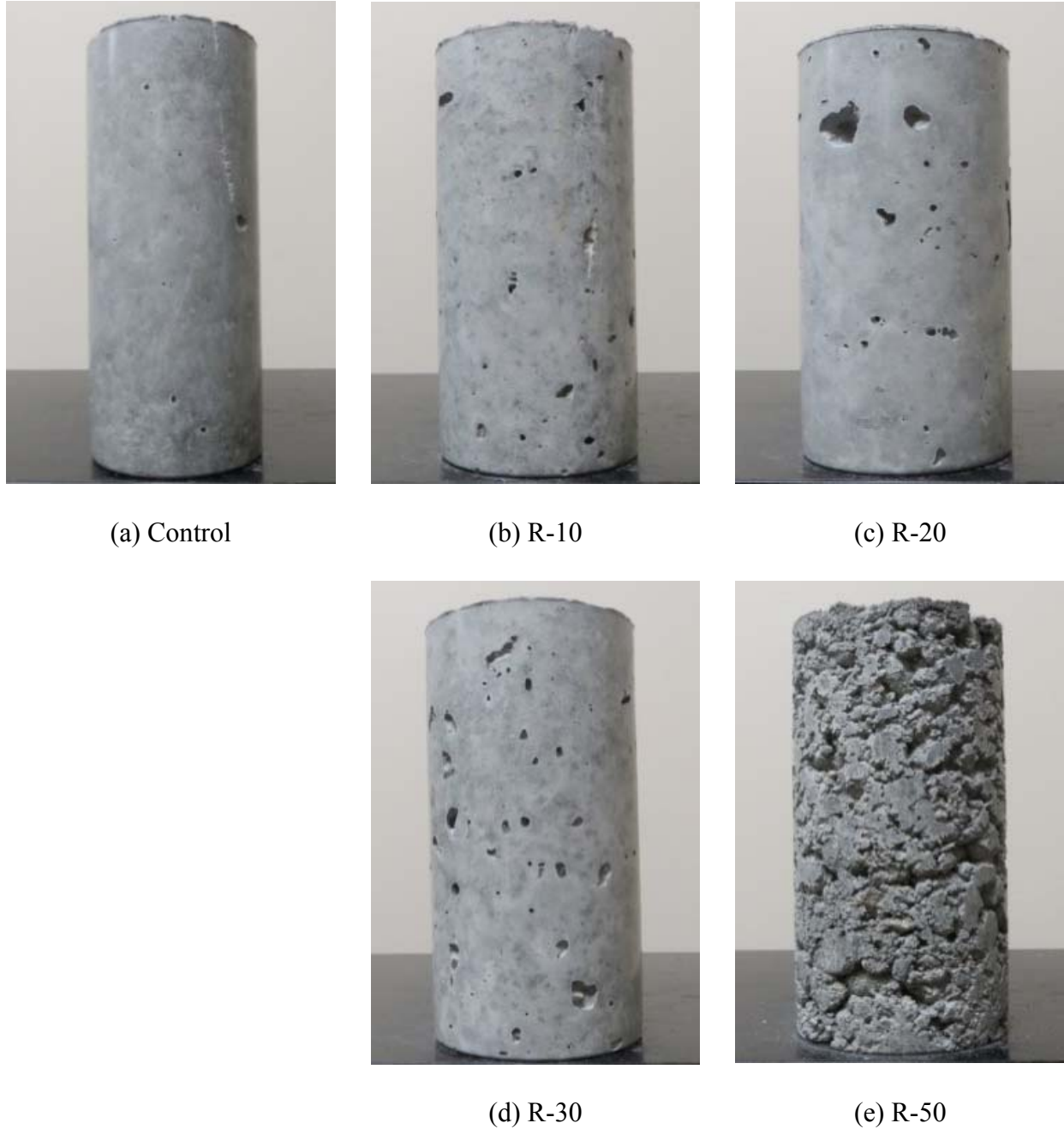
Figure 5.4: Photos of MSWI bottom ash replaced concrete with various replacement ratios
