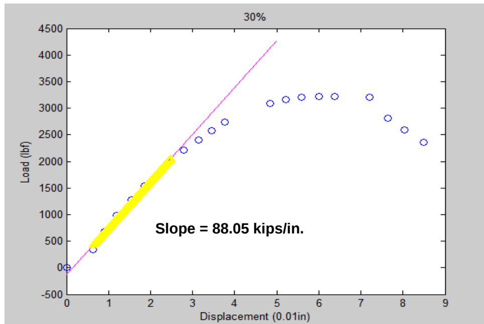
Figure A.4: IDT 'stiffness' for the mixture with 30% BA
