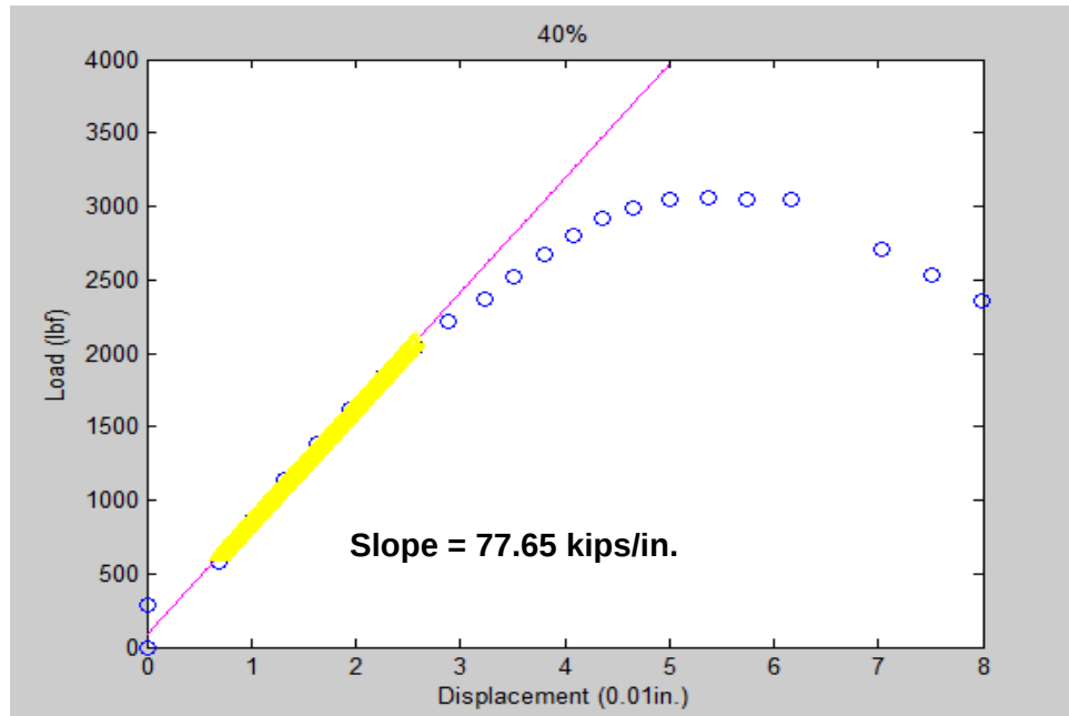
Figure A.5: IDT 'stiffness' for the mixture with 40% BA
