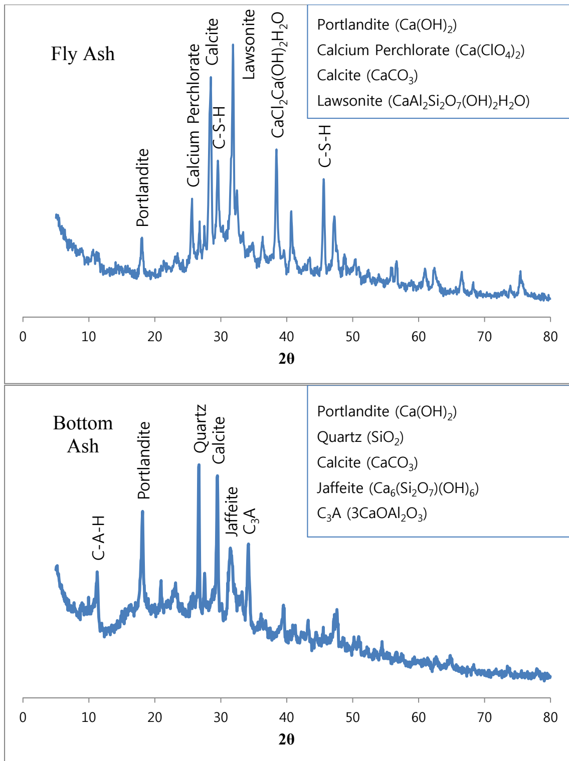
Figure 3.4: XRD of MSWI fly ash (top) and bottom ash (bottom)
