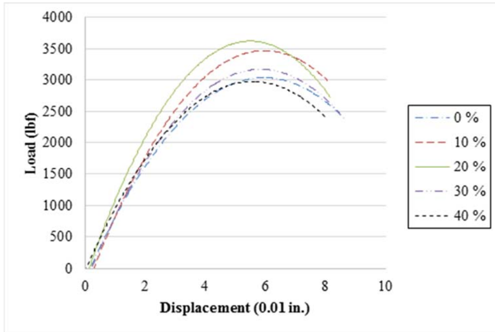
Figure 6.12: Load-displacement curve for dry samples
