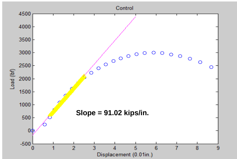
Figure A.1: IDT 'stiffness' for the control mixture (0% BA)
