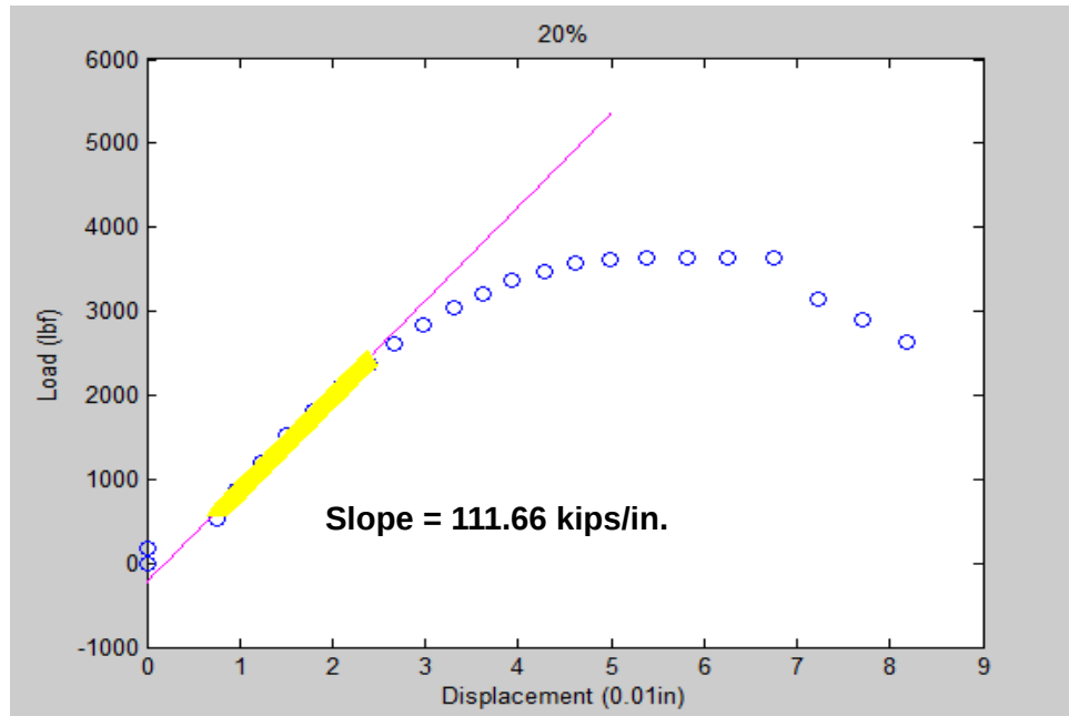
Figure A.3: IDT 'stiffness' for the mixture with 20% BA
