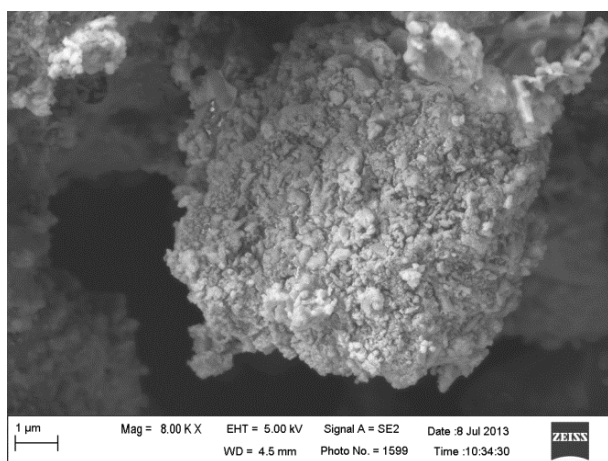
(e) 8,000X
