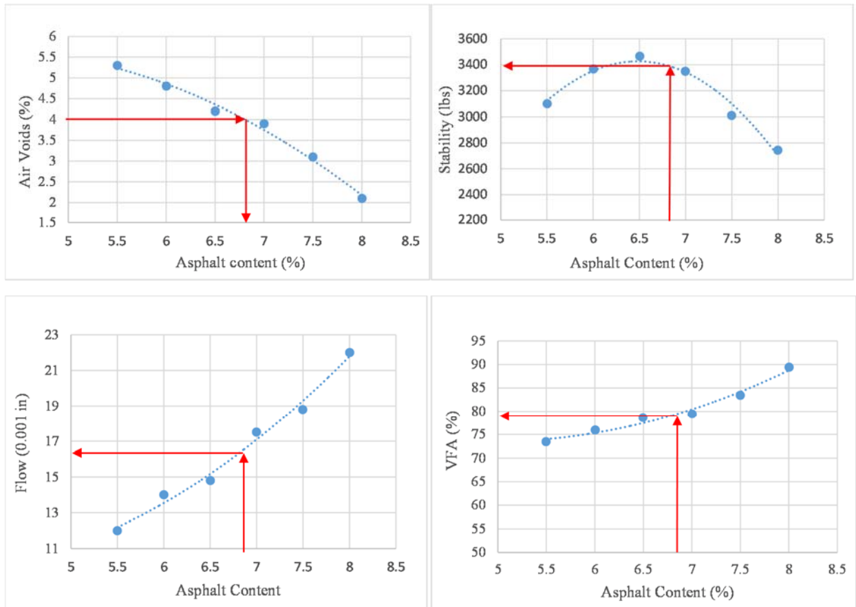
Figure 6.14: Graphical illustration of determining optimum asphalt binder at 20% BA replacement by Marshall Method
