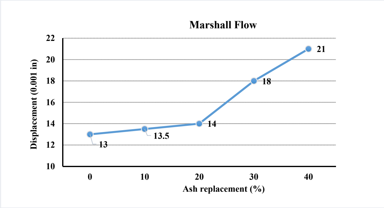
Figure 6.6: Flow test result
