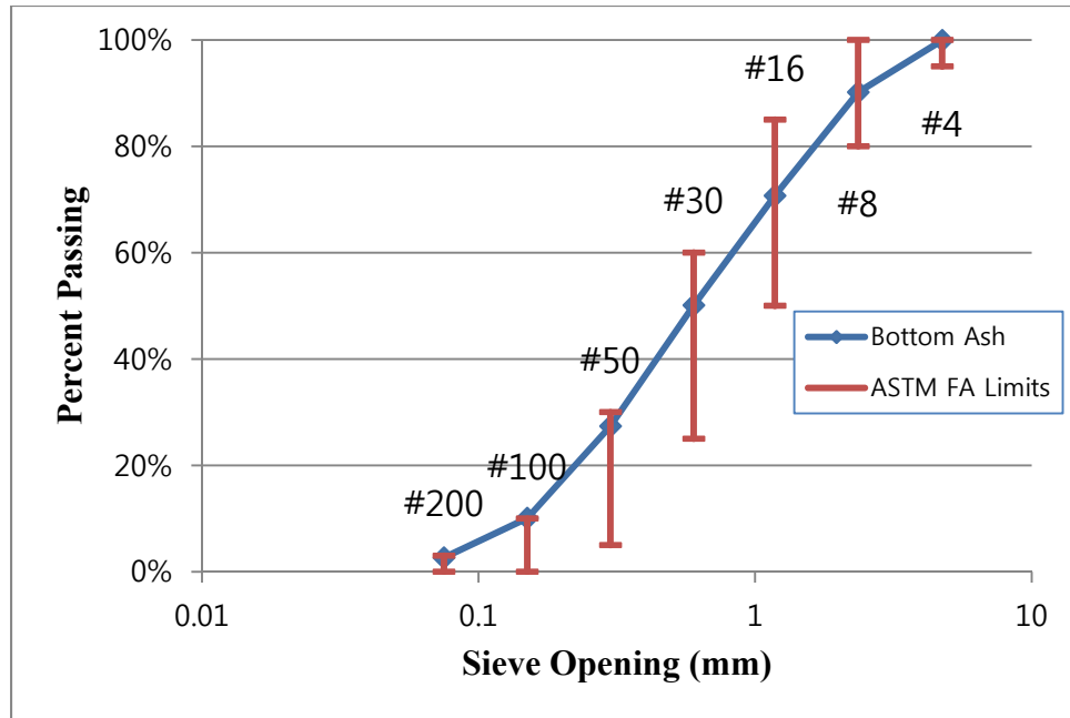
Figure 5.3: Particle size distribution of BA (ASTM C 33)
