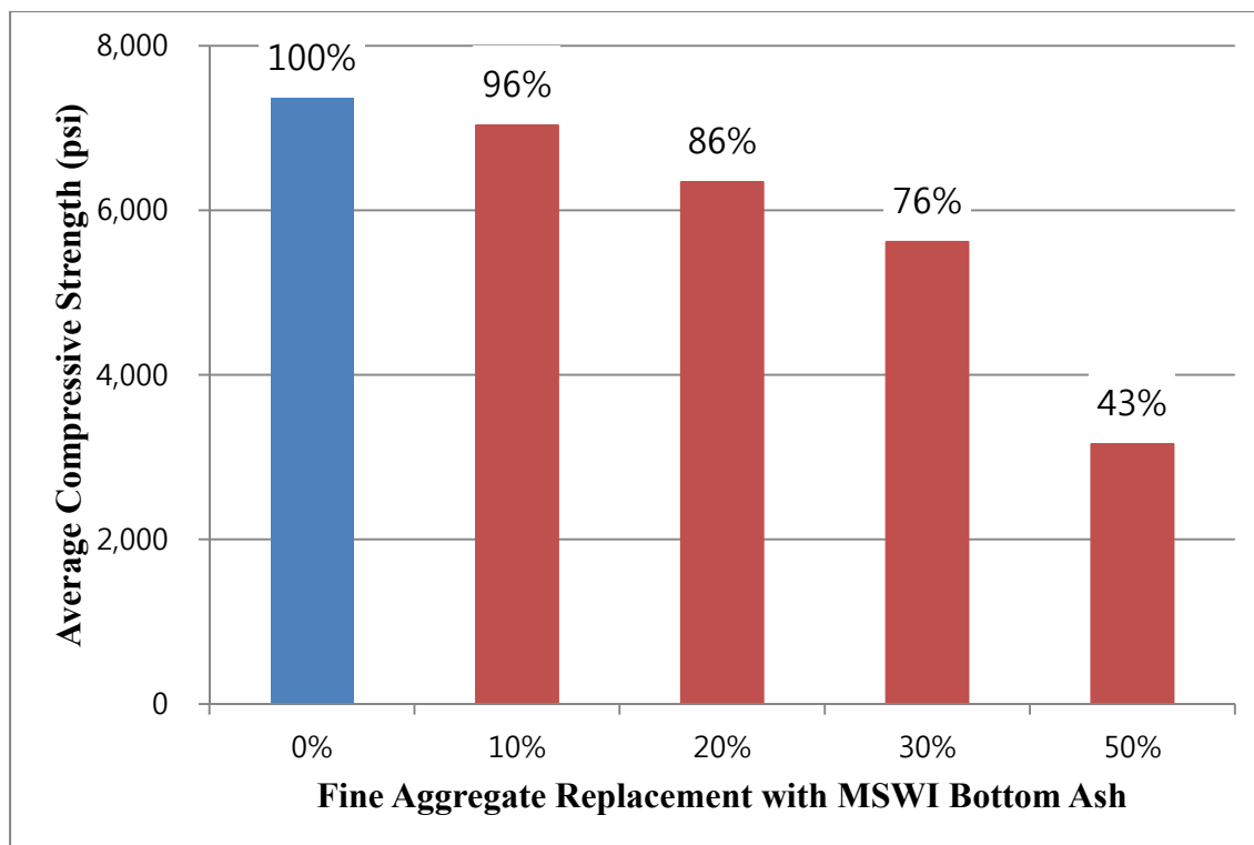
Figure 5.5: Compressive strengths of concrete specimens with different replacement ratios of BA with sand
