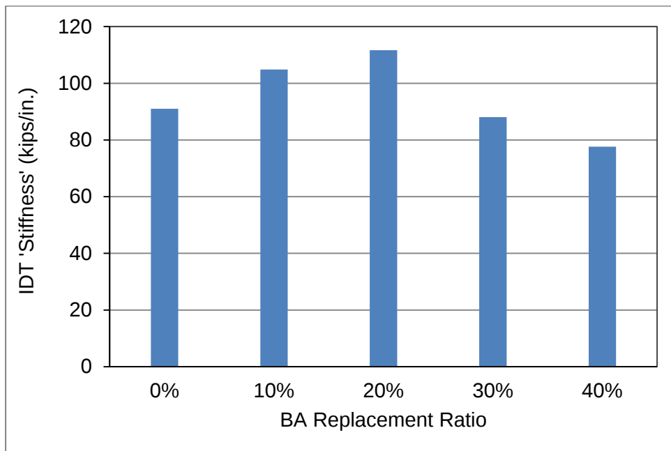
Figure 6.13: IDT 'stiffness' for the HMA specimens
