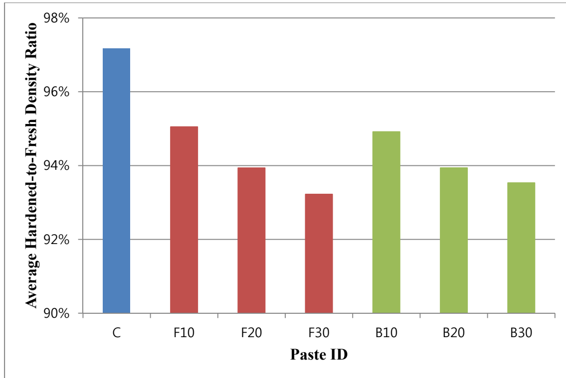
Figure 4.4: Average density ratios (hardened density / fresh density) for all mixtures
