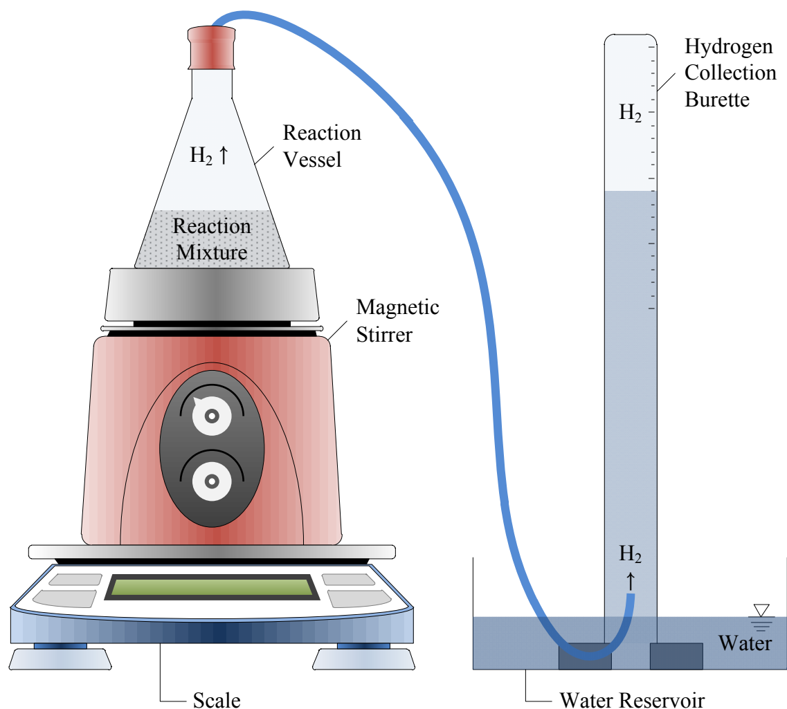
Figure 3.5: Test setup for volume of hydrogen gas measurement
