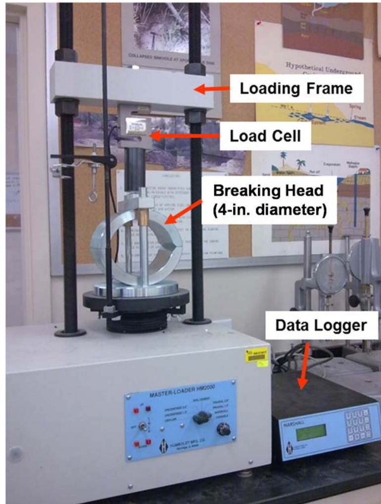
Figure 6.4: Marshall test apparatus and 4-in. breaking head at the UCF geotechnical laboratory
