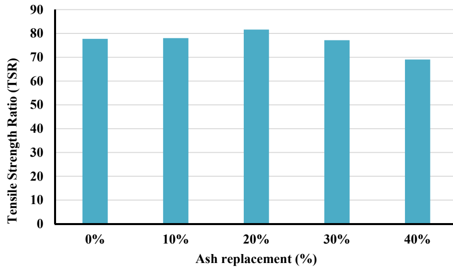
Figure 6.11: Tensile strength ratio
