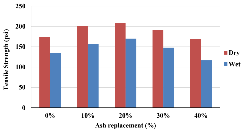
Figure 6.10: Tensile strength of dry and wet samples
