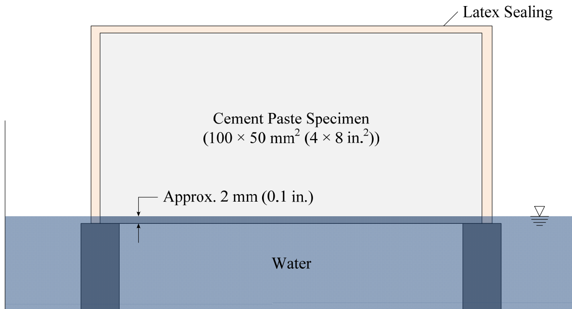
Figure 4.2: Configuration of one-dimensional water absorption test setup
