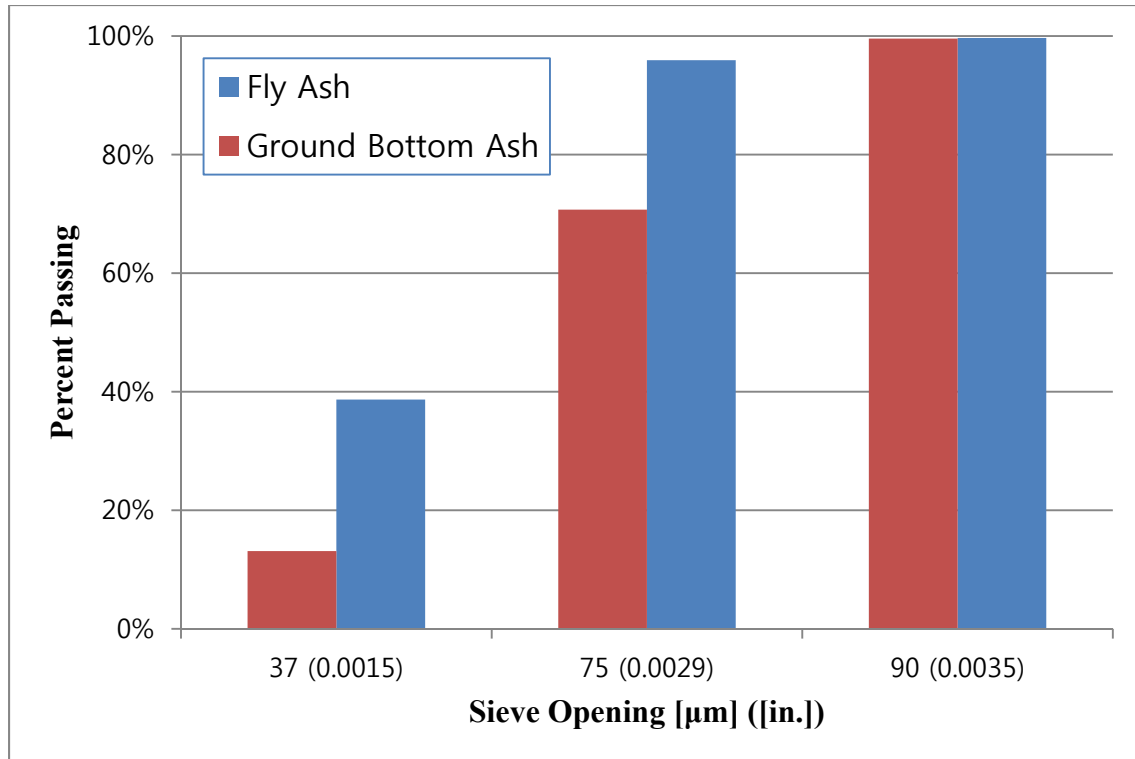
Figure 4.1: Particle size distribution of MSWI ashes
