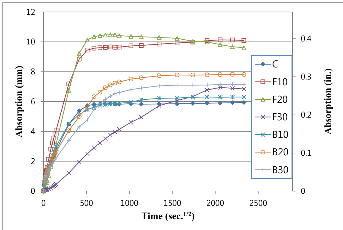
Figure 4.5: Water absorption for all cement paste cylinders
