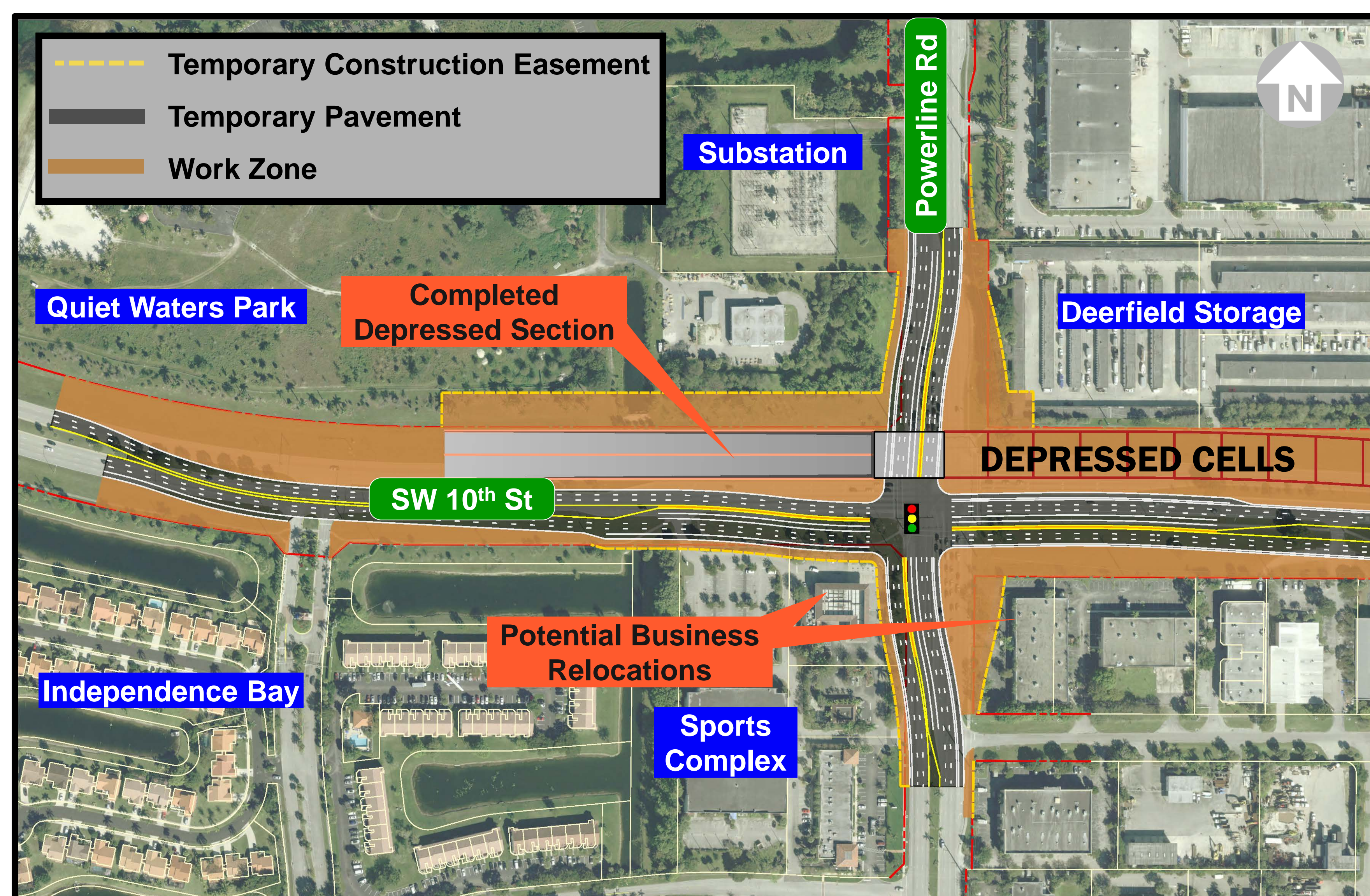
Phase III: Build depressed section east of Powerline Road
