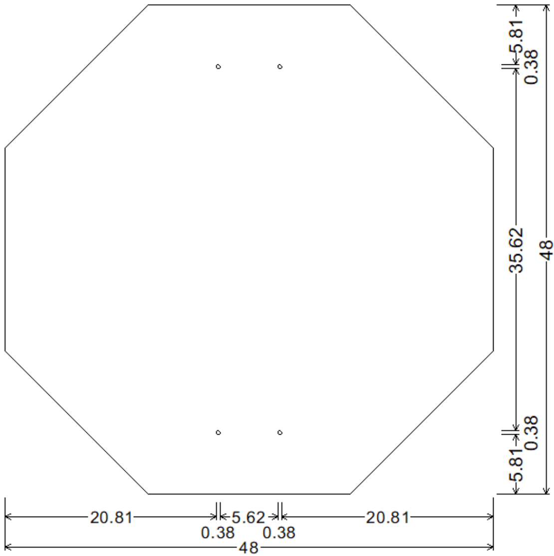
DRAWING 6A 48 INCH OCTAGON; No border, None;
