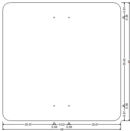
DRAWING 31 48X48; 3.00" Radius, No border, White on, None; Table of widths and spaces
