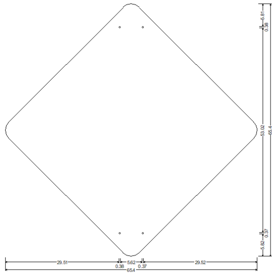
DRAWING 31 48X48 SQUARE; 48.00" across sides 3.00" Radius, No border, None; Table of widths and spaces
