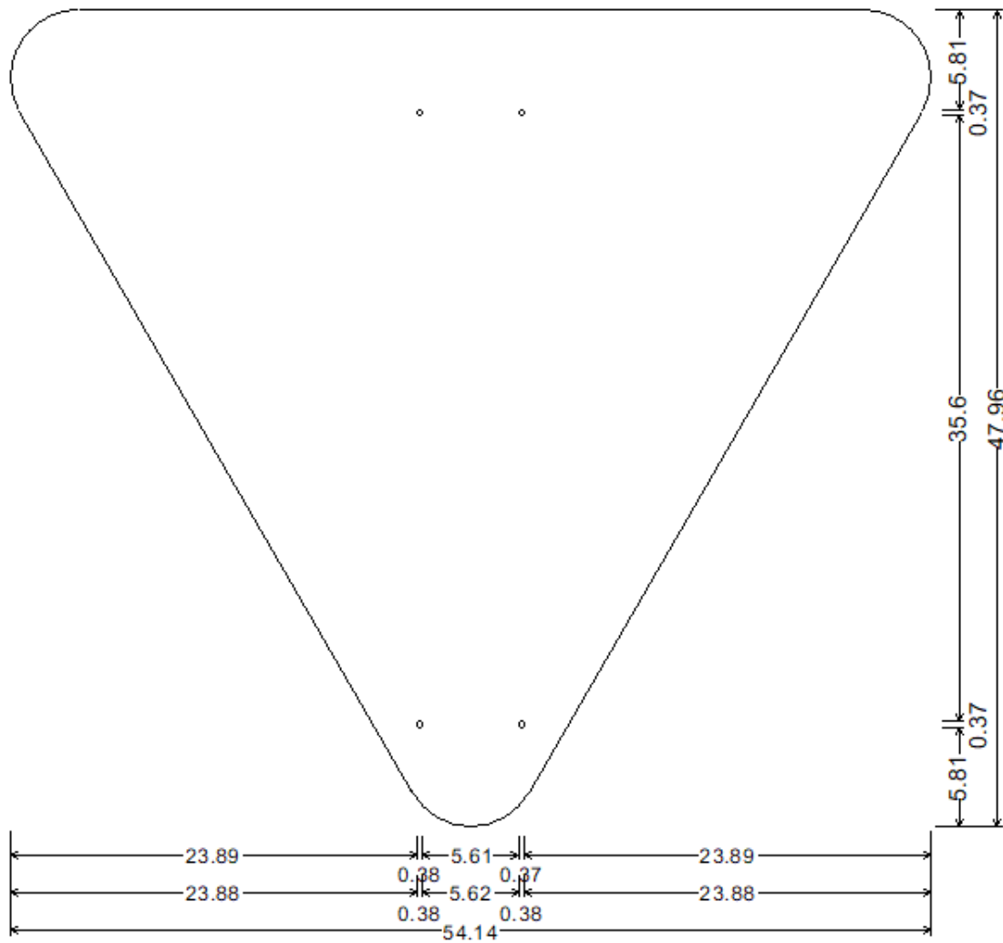
DRAWING 12C 60 INCH YIELD; 60.00" corner to corner 4.00" Radius, No border, None;
