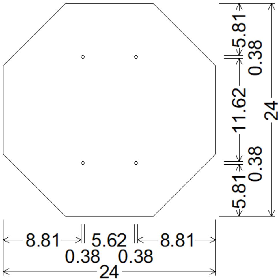
DRAWING 4 24 INCH OCTAGON; No border, None;
