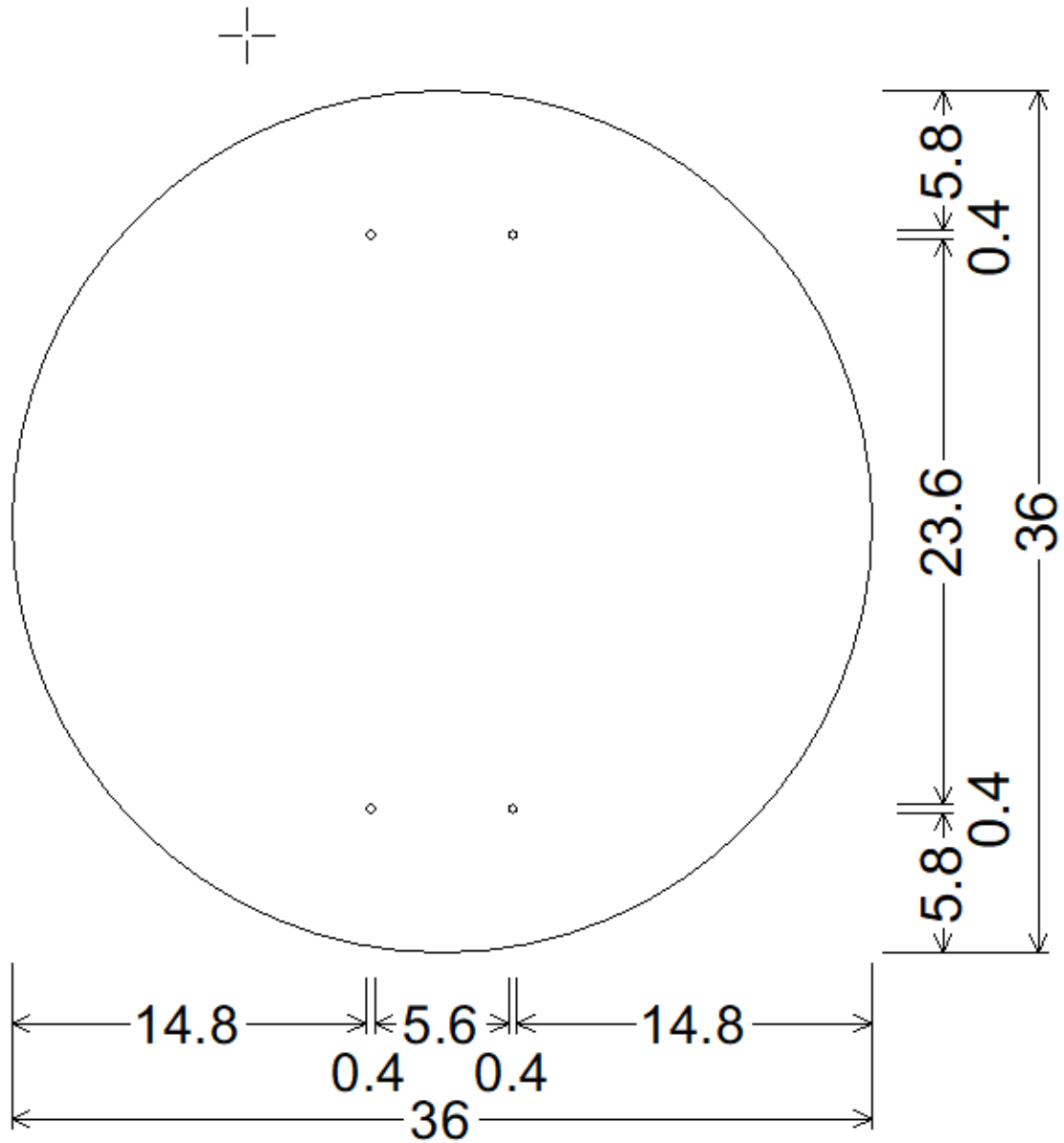
DRAWING 3 36 INCH ROUND; No border, None;
