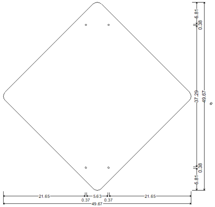
DRAWING 32 36X36 DIA; 36.00" across sides 1.50" Radius, No border, None; Table of widths and spaces
