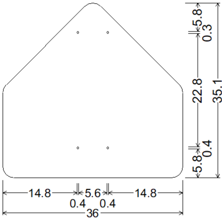
DRAWING 9 36 INCH PENTAGON; 36.0" base to corner 2.3" Radius, No border, None; Table of widths and spaces
