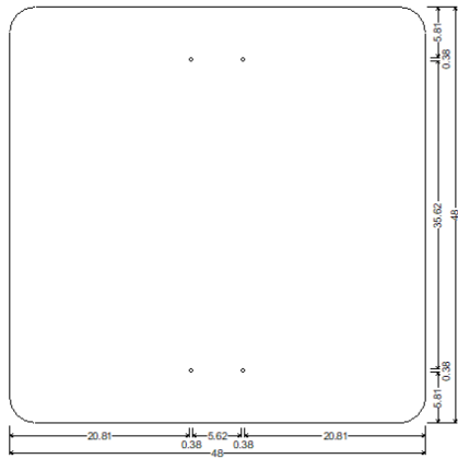
DRAWING 34 48X48; 3.00" Radius, No border, White on, None; Table of widths and spaces
