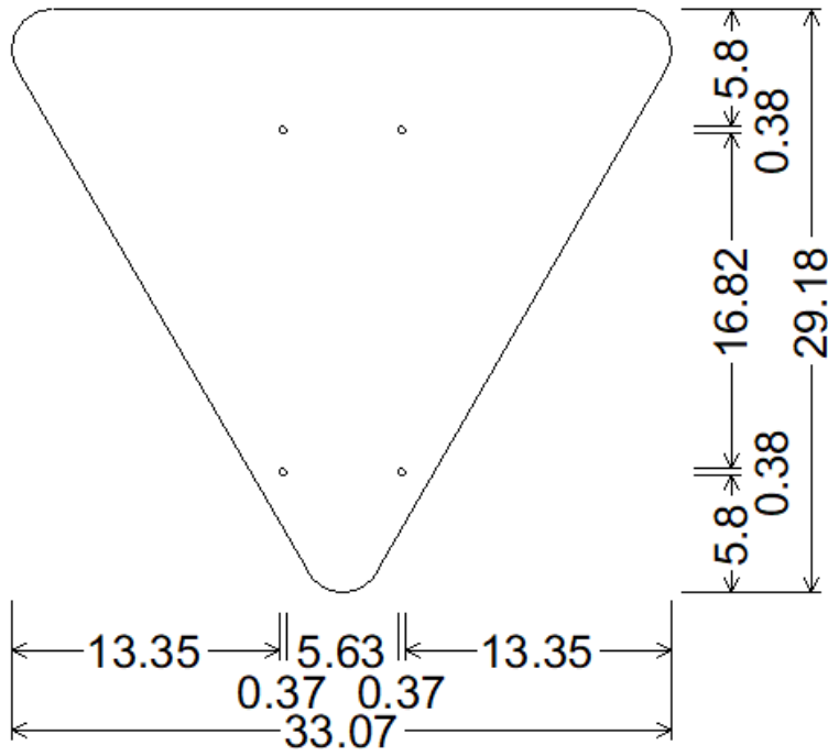
DRAWING 12A 36 INCH TRIANGLE; 36.00" corner to corner 2.00" Radius, No border, None; Table of widths and spaces
