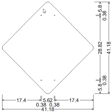
DRAWING 11a 30X30 ON DIAMOND; 30.00" across sides 1.50" Radius, No border, None; Table of widths and spaces
