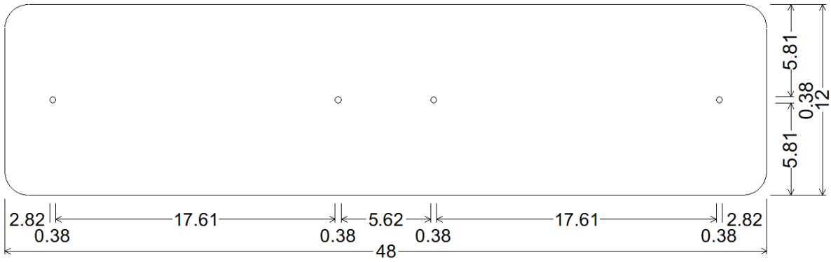
DRAWING 21 12X48; 1.50" Radius, No border, White on, None; Table of widths and spaces
