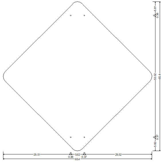
DRAWING 34 48X48 SQUARE; 48.00" across sides 3.00" Radius, No border, None; Table of widths and spaces
