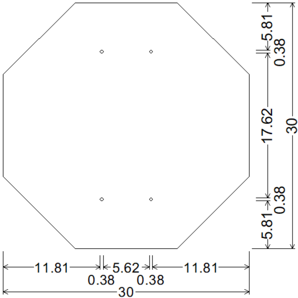
DRAWING 5 30 INCH OCTAGON; No border, None;
