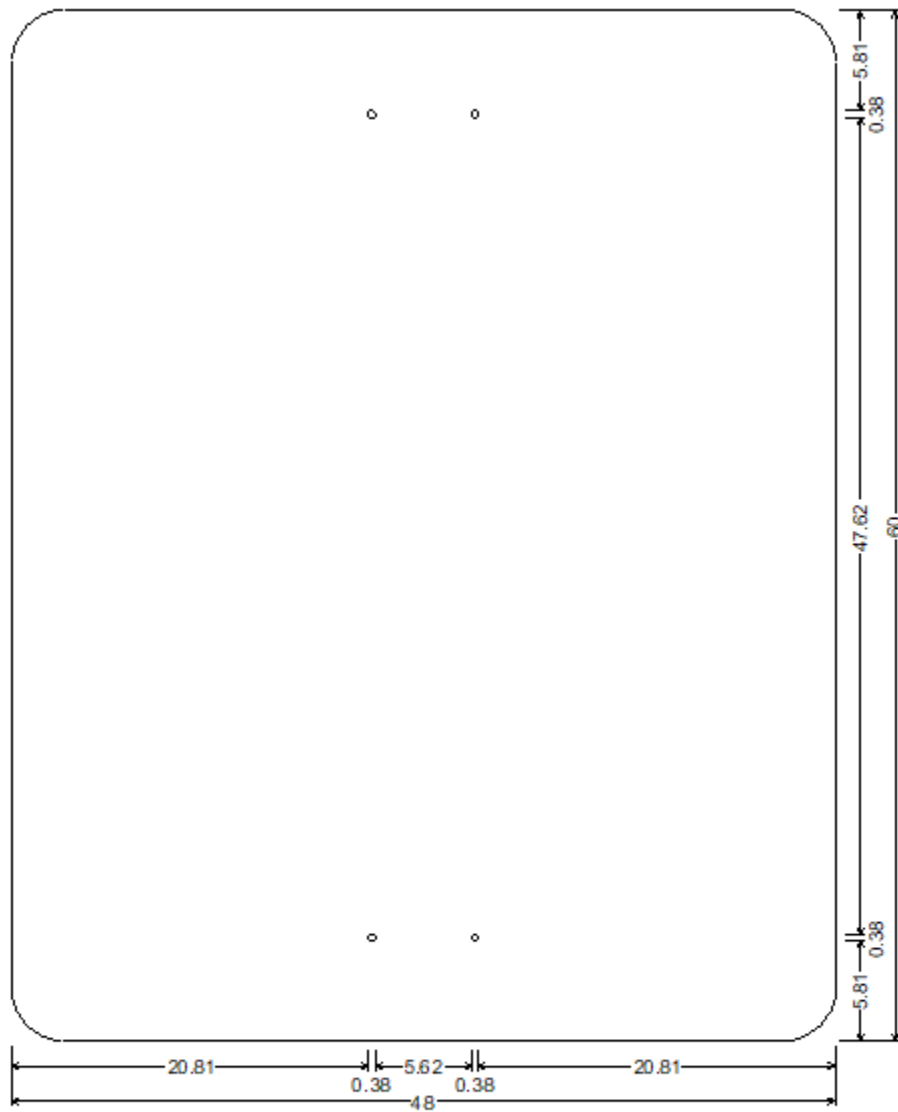
DRAWING 35 48X60; 3.00" Radius, No border, White on, None; Table of widths and spaces
