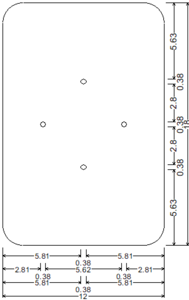
Drawing 18 12x18 Rectangle; 1.50" Radius, No border, White on, None; Table of widths and spaces
