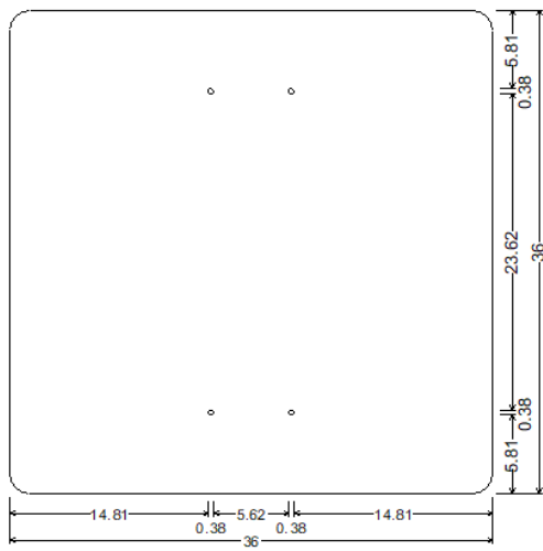
DRAWING 32 36X36; 1.50" Radius, No border, White on, None; Table of widths and spaces
