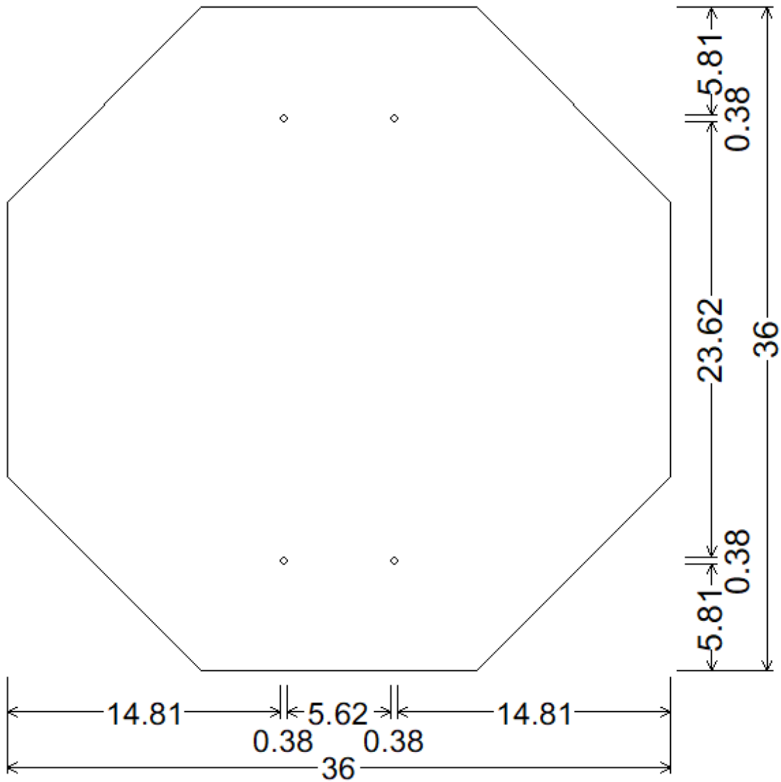
DRAWING 6 36 INCH OCTAGON; No border, None;
