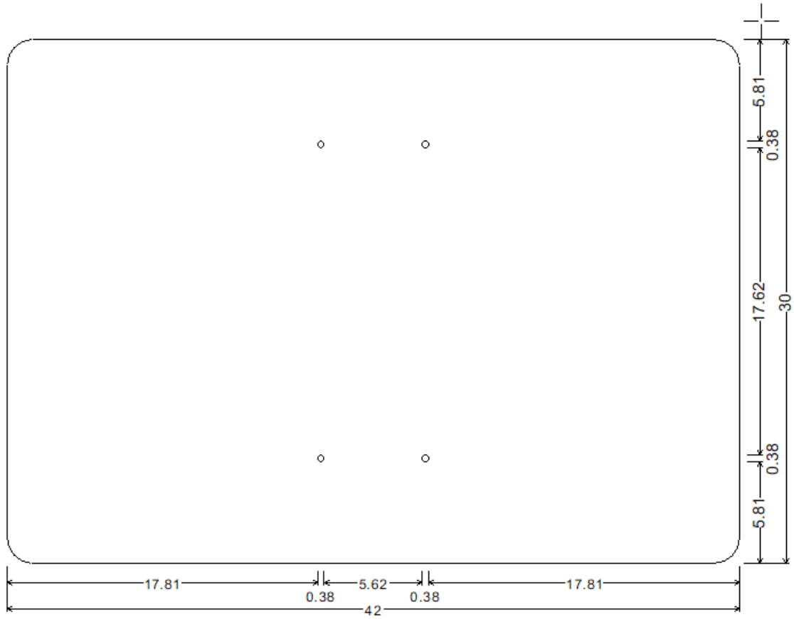
DRAWING 41 30X42; 1.50" Radius, No border, White on, None; Table of widths and spaces
