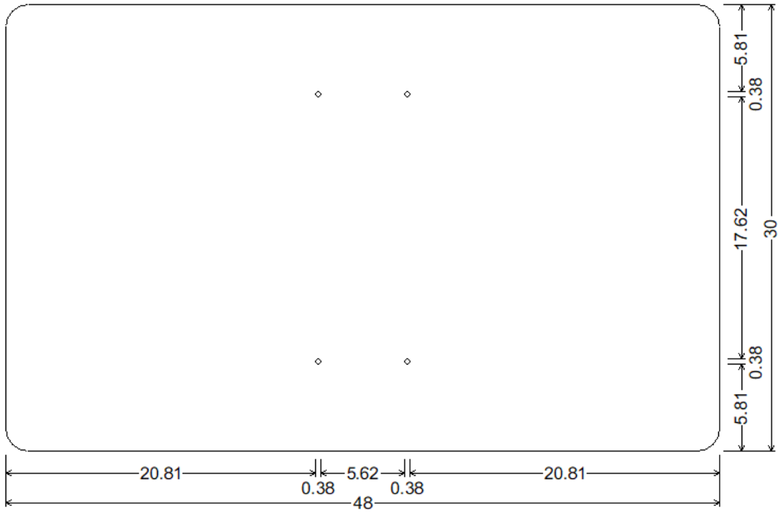
DRAWING 31 30X48; 1.50" Radius, No border, White on, None; Table of widths and spaces
