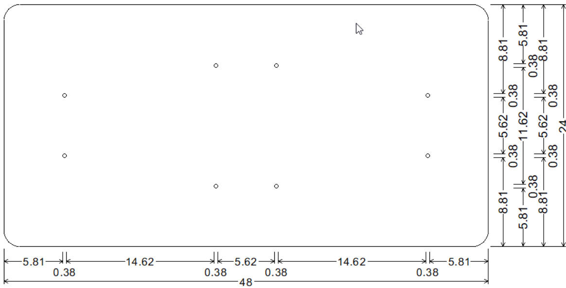
DRAWING 29 24X48; 1.50" Radius, No border, White on, None; Table of widths and spaces
