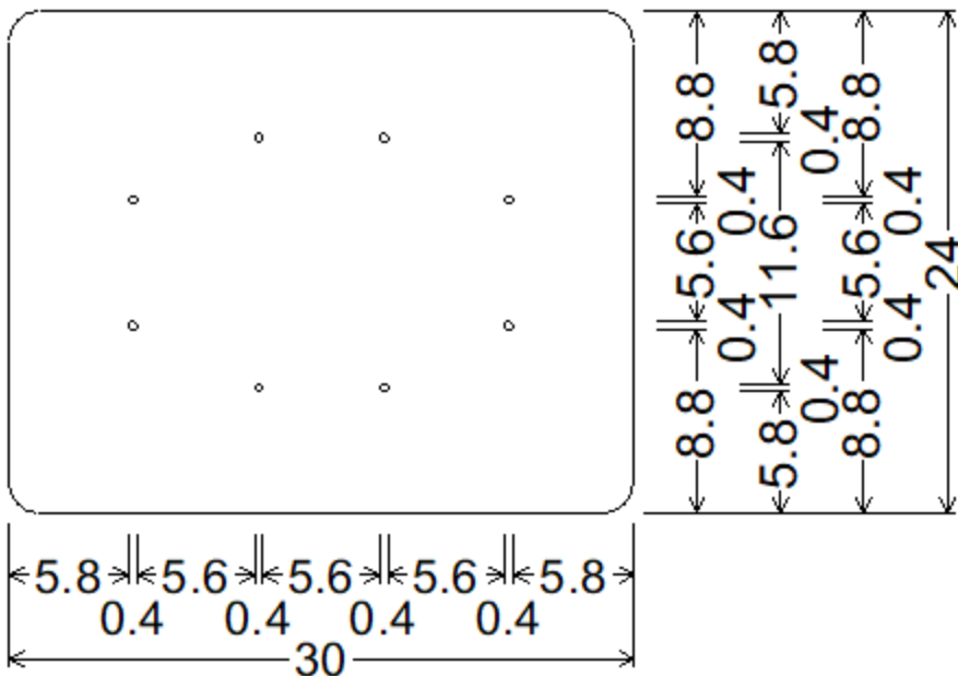
DRAWING 8 24"X30" RECTANGLE; 1.5" Radius, No border, White on, None; Table of widths and spaces
