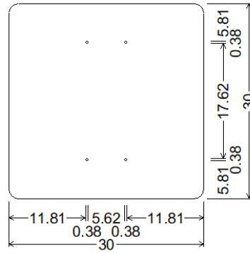
DRAWING 11B GOES WITH DRAWING 11a 30X30 SQUARE; 1.50" Radius, No border, White on, None; Table of widths and spaces
