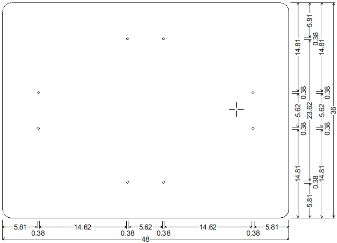
DRAWING 33 36X48; 1.50" Radius, No border, White on, None; Table of widths and spaces
