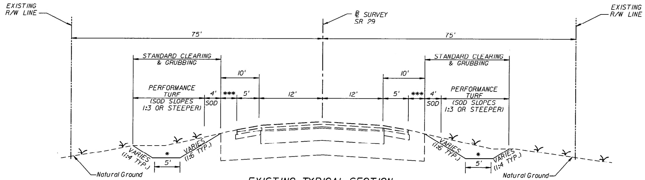
EXISTING TYPICAL SECTION SR 29 STA. 209+40.00 TO STA. 532+00.00 ** RE-GRADE ROADSIDE DITCHES
