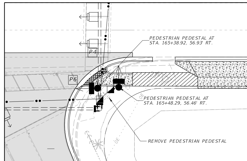
SOUTHEAST QUADRANT SR 544 AT 34 STREET NW
