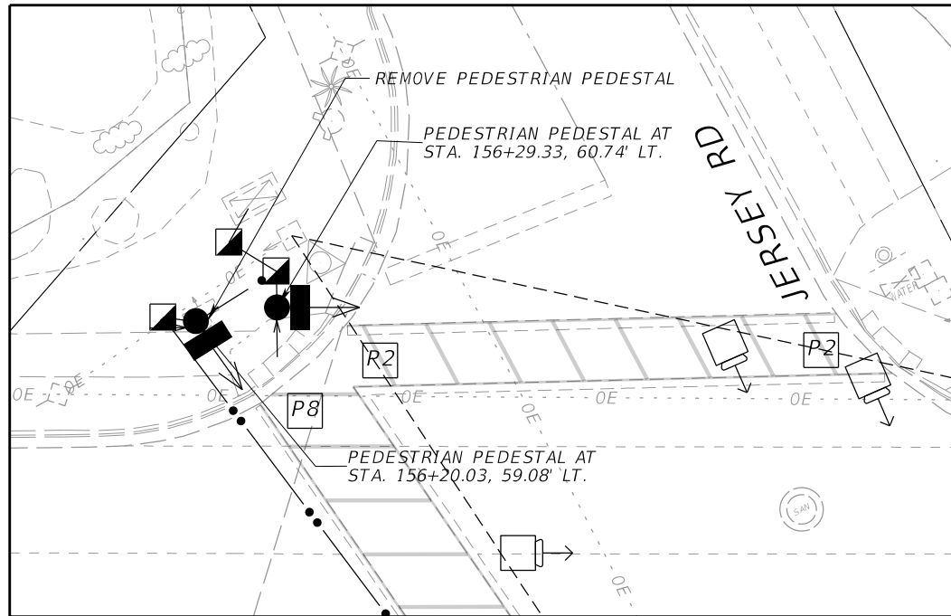
NORTHWEST QUADRANT SR 544 AT JERSEY RD
