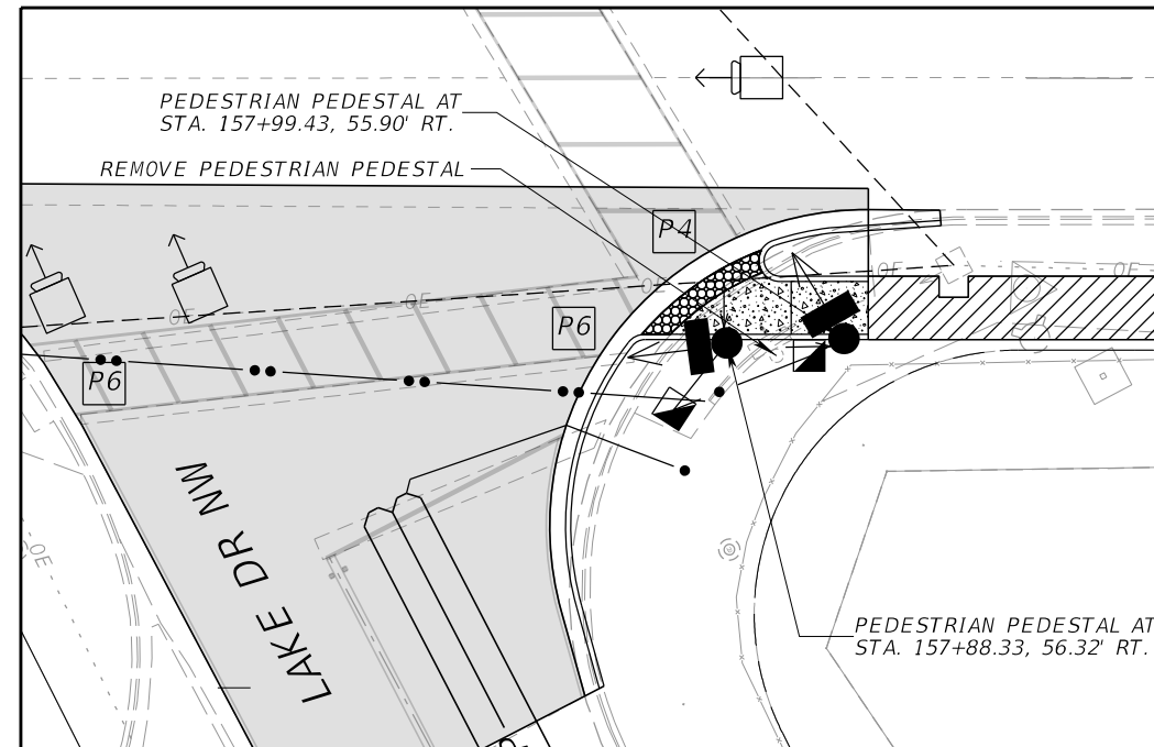
SOUTHEAST QUADRANT SR 544 AT LAKE DR NW
