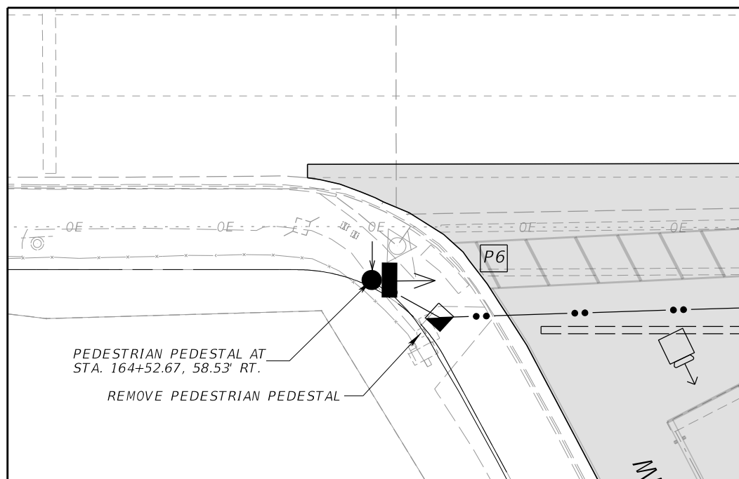
SOUTHWEST QUADRANT SR 544 AT 34 STREET NW
