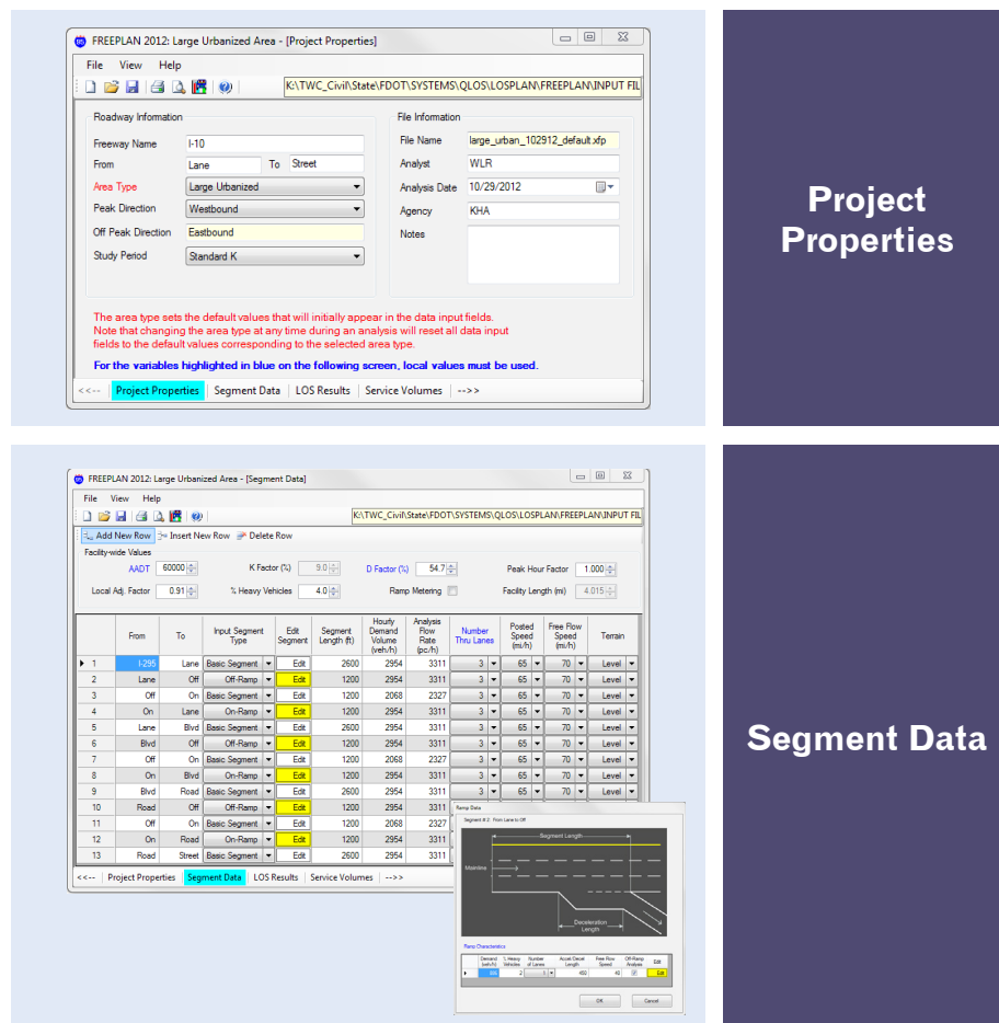
Figure 12-4 FREEPLAN Input Screens
