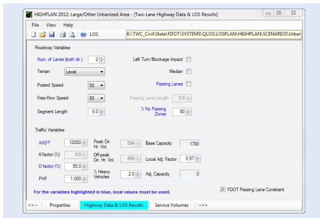
Figure 12-7 HIGHPLAN Output Screens
