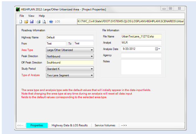
Figure 12-6 HIGHPLAN Input Screens
