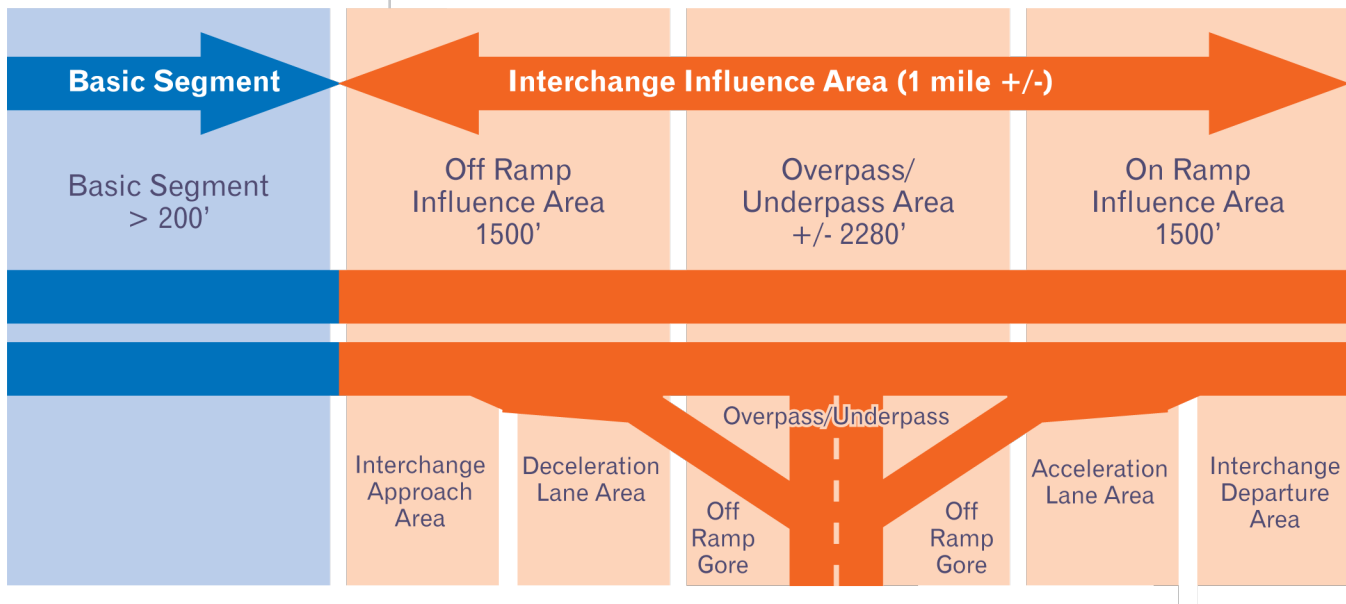
Figure 2-3 Typical Freeway Interchange
