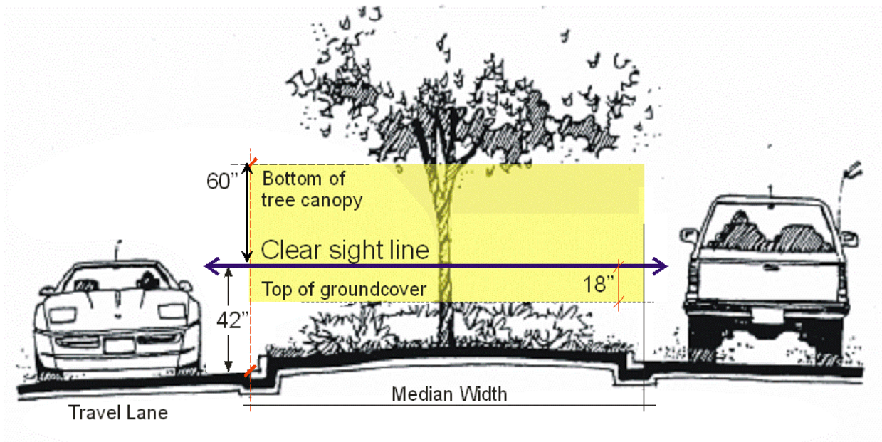
Exhibit 53 Clear Sight Window
