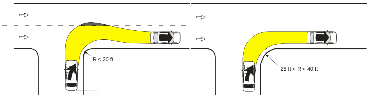
Exhibit 18 Encroachment Due to Inadequate Driveway Design
