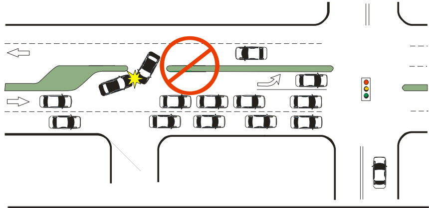
Exhibit 63 No Median Openings Across Left Turn Lane
