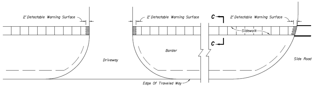
DISCONTINUOUS SIDEWALK
