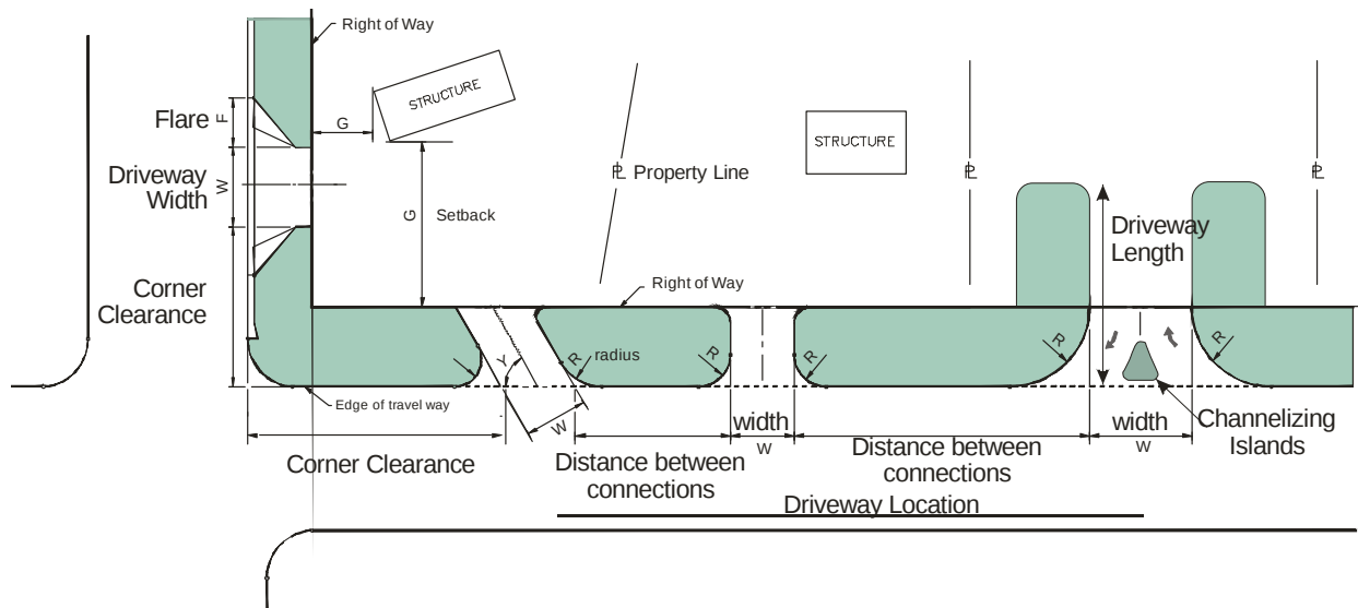
Exhibit 2 Driveway Dimensions
