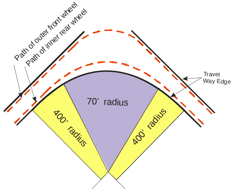
WB-62 SEMITRAILER COMBINATION
