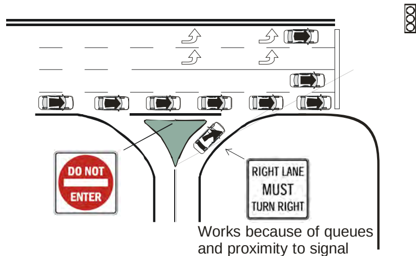
“Pork Chop” Close to an Intersection
