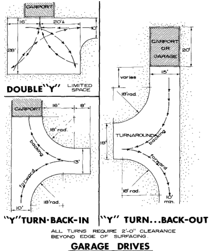
Exhibit 41 Carport Turn-Arounds
