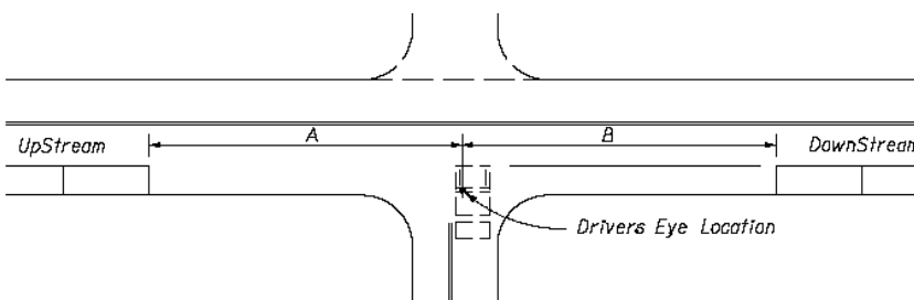
Exhibit 54 Upstream and Downstream Sight Distance
