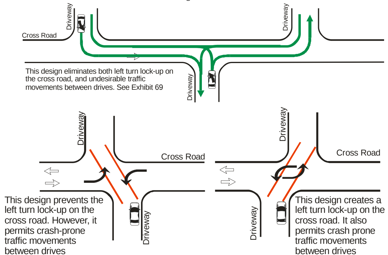
Exhibit 68 Avoid Jog Maneuvers
