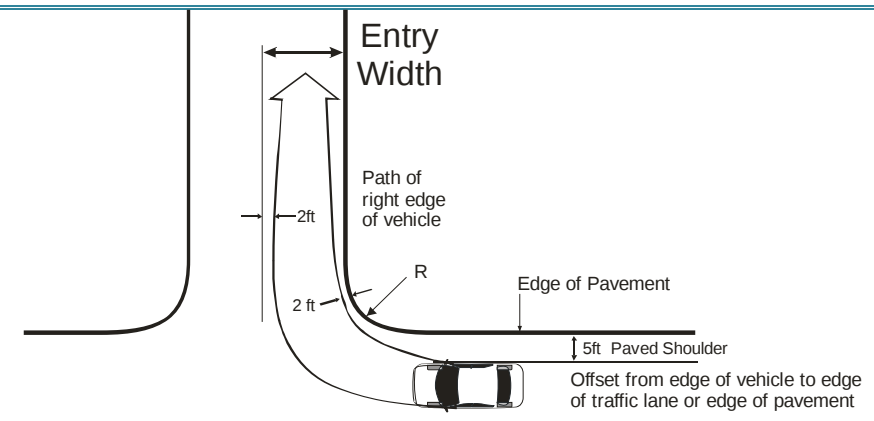
Exhibit 14 Important Measures that Determine the Entry Operations of a Driveway
