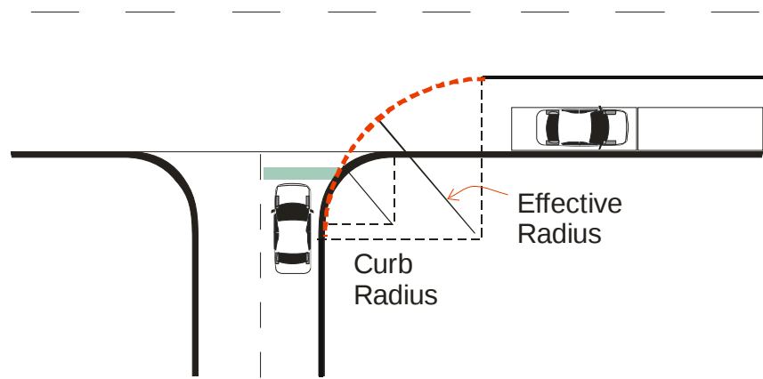
Exhibit 9 A bike lane can add to the effective radius of the driveway – but use it wisely
