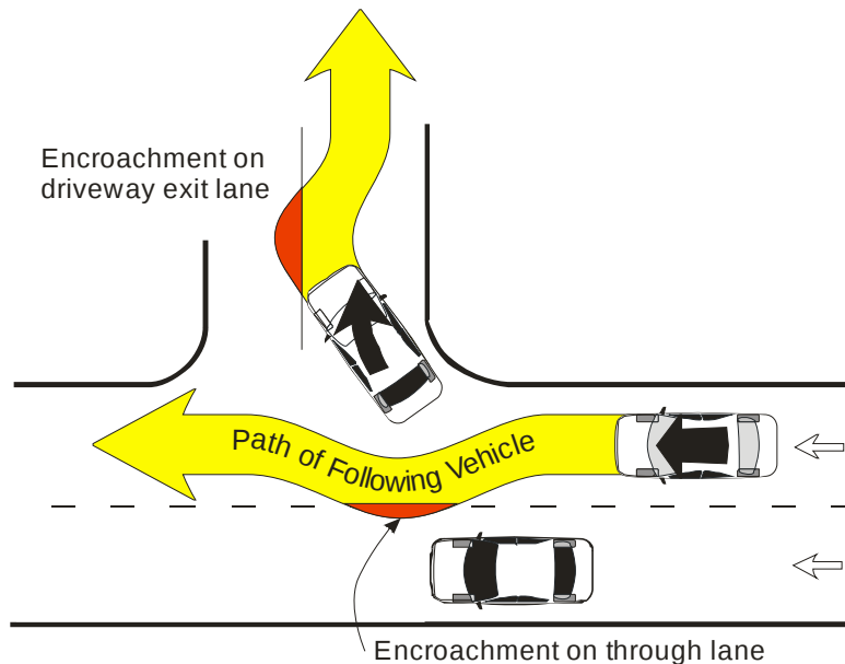
Exhibit 17 Encroachment Due to Inadequate Driveway Design
