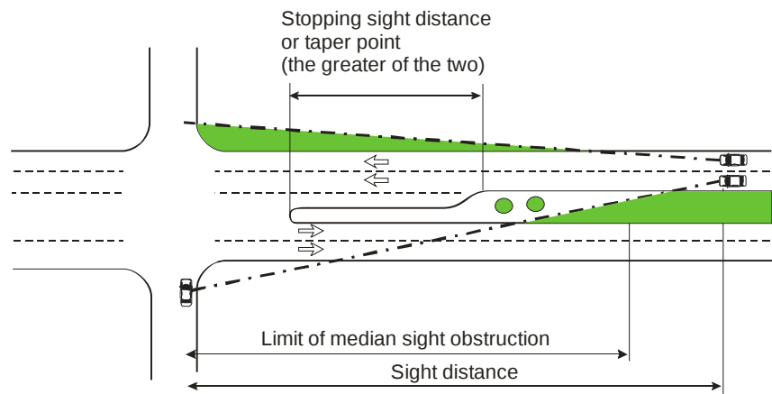
Exhibit 52 Stopping Sight Distance
