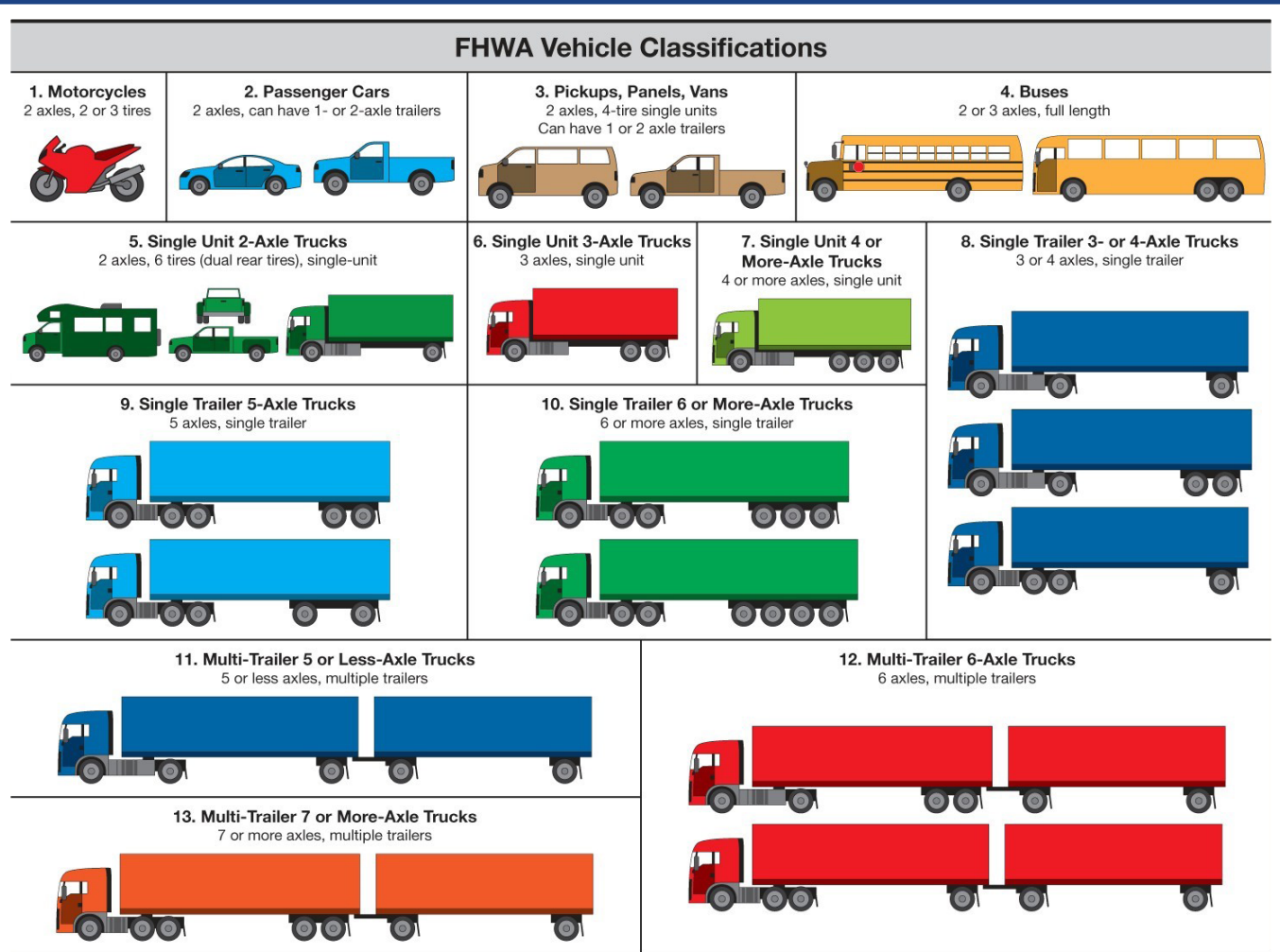
Figure 2-2 FHWA Vehicle Classification Scheme F
