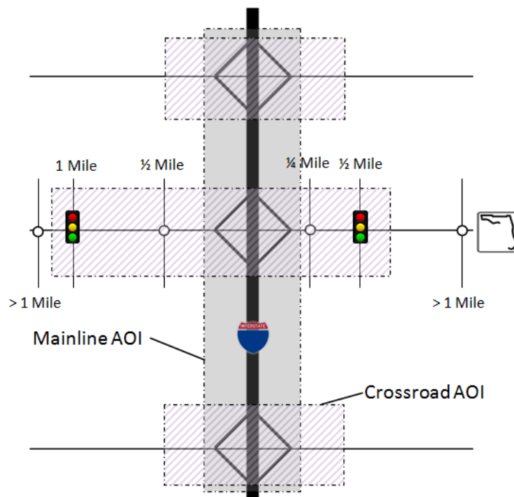
Figure 2- 1 Area of Influence Along Mainline and Crossroad
