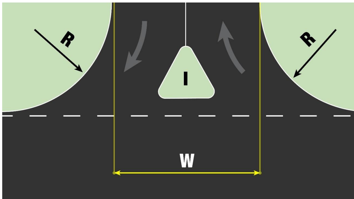
Figure 39 – Driveway Width
