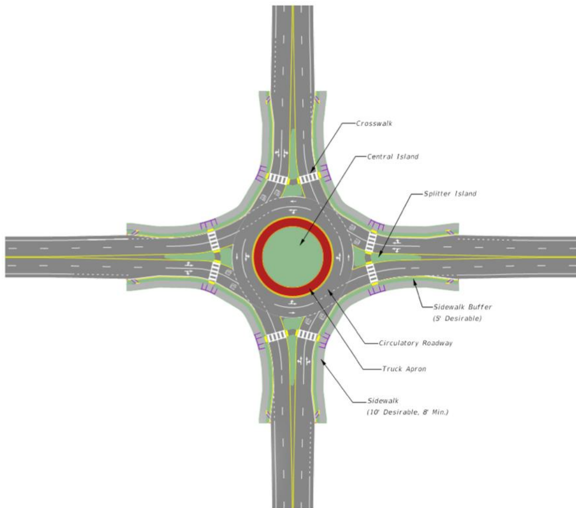
Figure 79 – Roundabout Details
