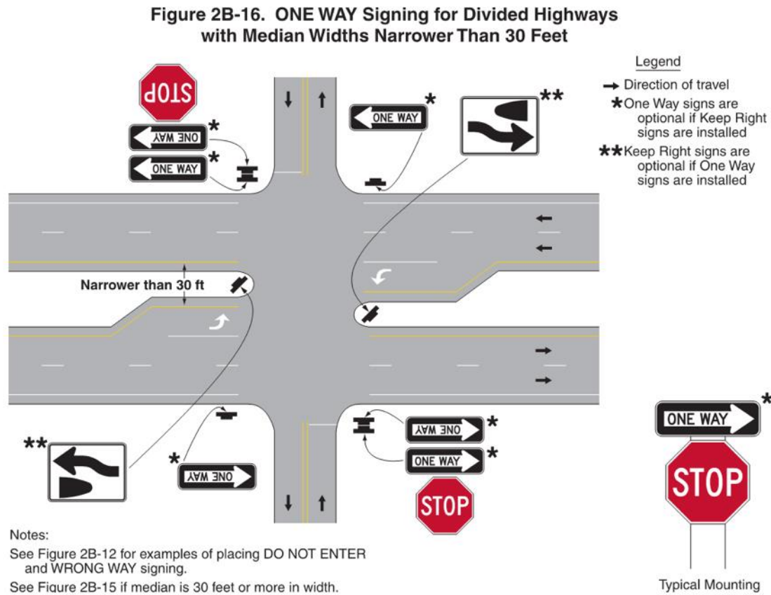
Figure 33 – MUTCD Figure 2B-16
