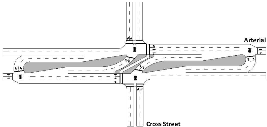
Figure 75 – Signalized Restricted Crossing U-Turn (RCUT), or Superstreet
