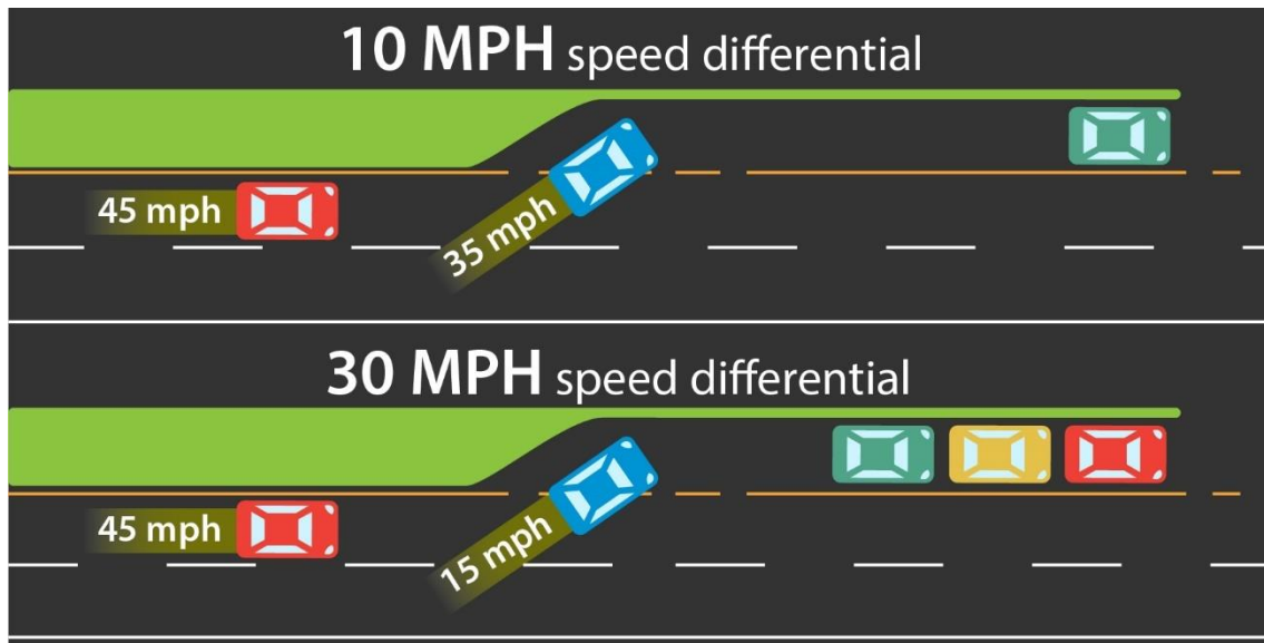
Figure 25 – Excessive Deceleration
