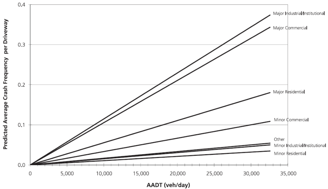
Source: Fig 12-5: Multiple Vehicle Driveway Related Collisions on Two-Lane Undivided Arterials (2U)
