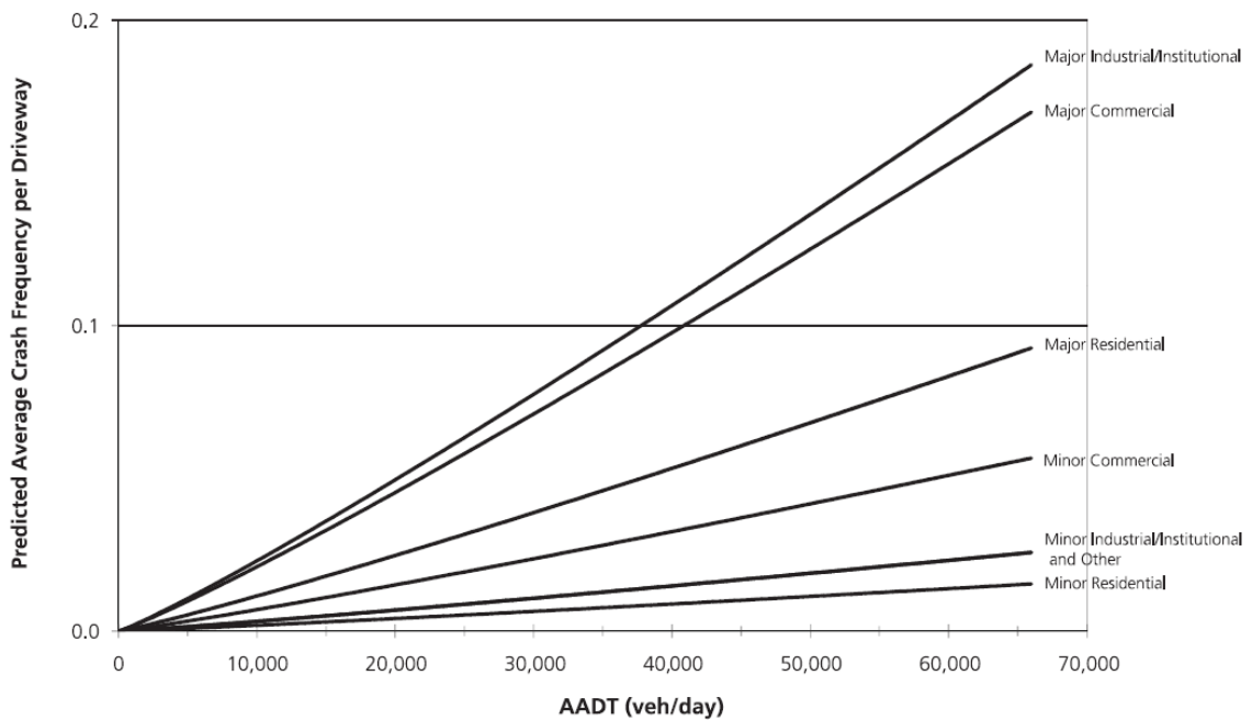
Source: Fig 12-7: Multiple Vehicle Driveway Related Collisions on Four-Lane Undivided Arterials (4U)
