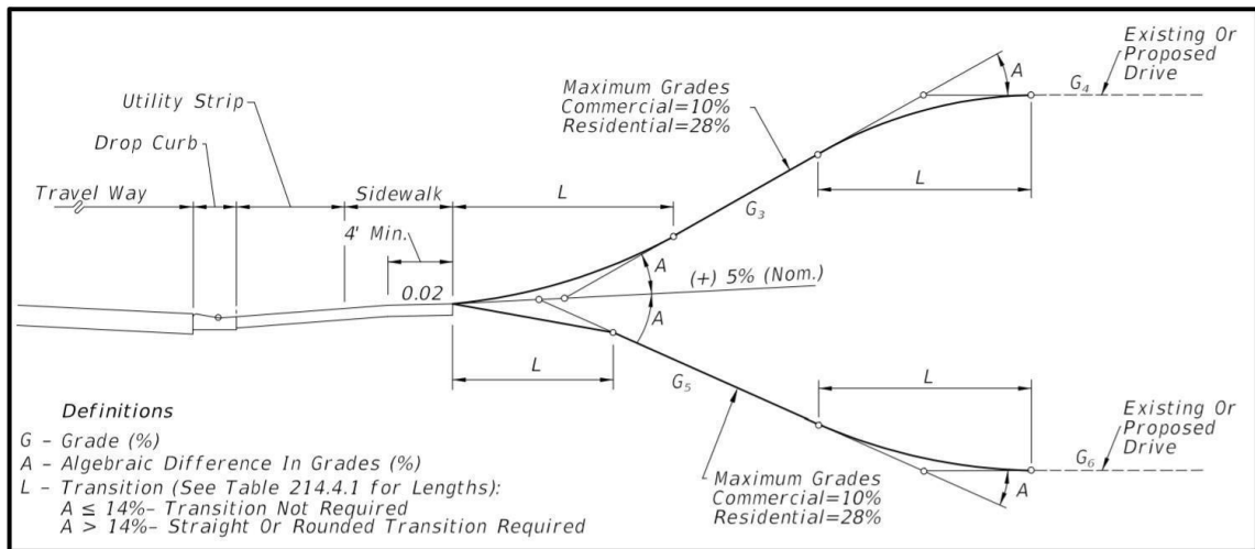
Figure 58 | Curbed Roadway Driveway Profiles
