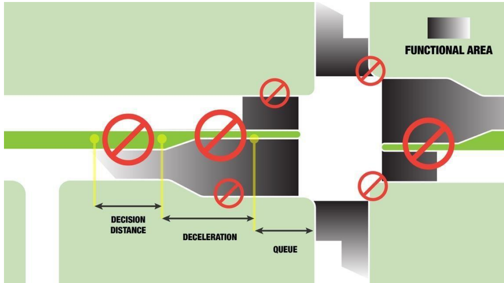
Figure 31 | Functional Area and Medians
