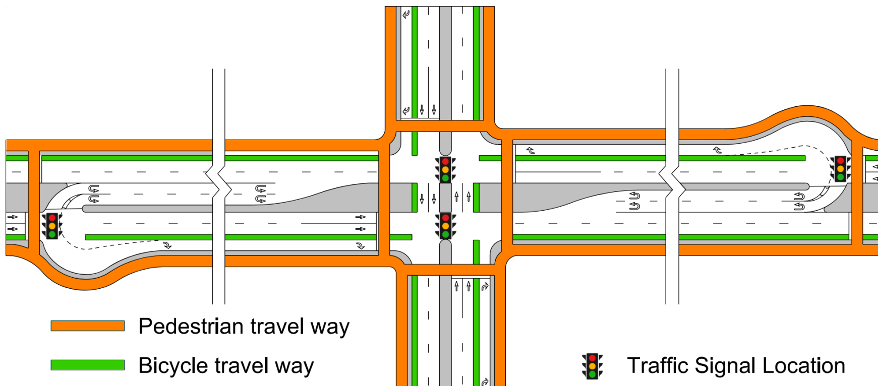
Figure 110 | MUT Intersection Pedestrian Crossing Locations and On-Street Bikeway Concept
