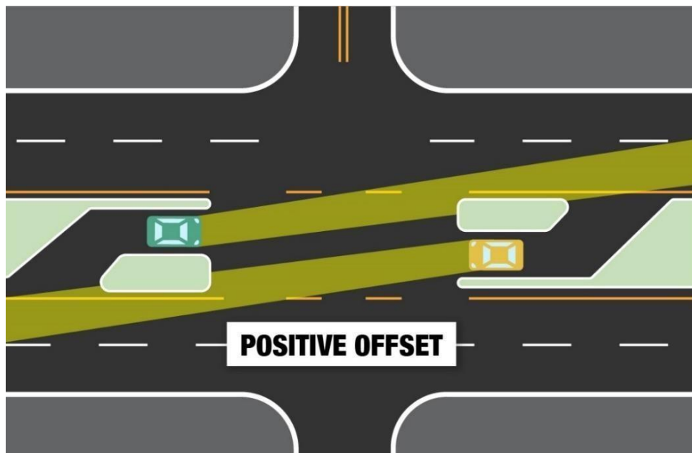
Figure 70 | Positive Offset between Opposing Left-Turn Lanes
