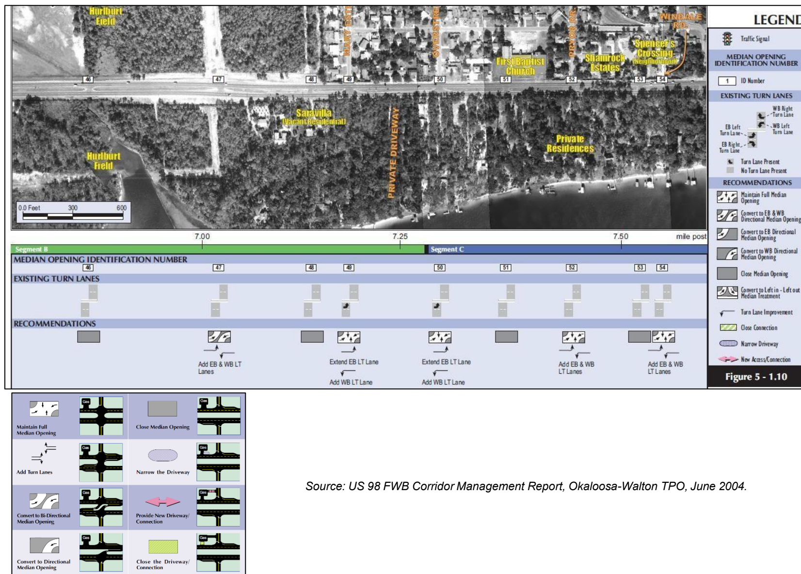
Figure 165 | Recommended Corridor Access Management Plan Example
