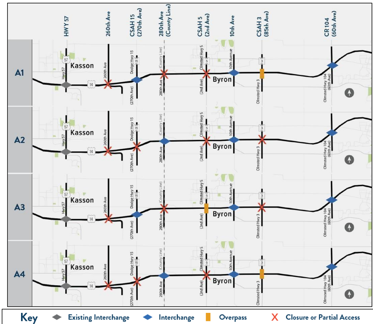
Figure 163 | Access Alternatives Summary Example
