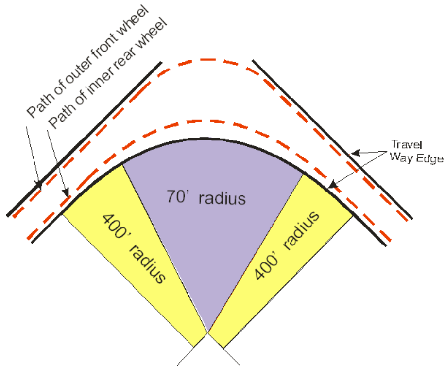
Figure 106 | Equivalent Compound Curves Geometrics for Departure Radii
