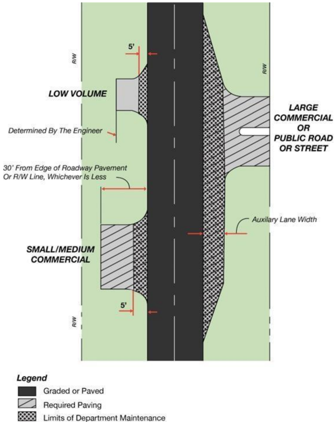
Figure 56 | Limits of Construction and Maintenance for Flush Shoulder “Rural” Section Connections
