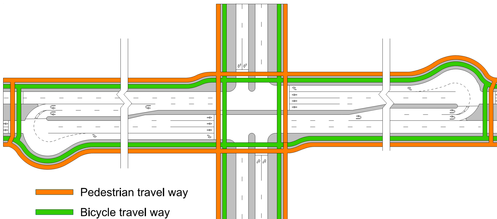
Figure 115 | RCUT Separated Bike Lane Concept
