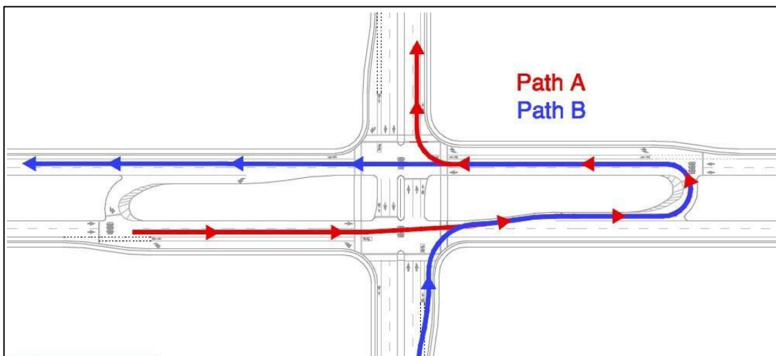
Figure 89 | Median U-Turn Intersection Vehicle Paths
