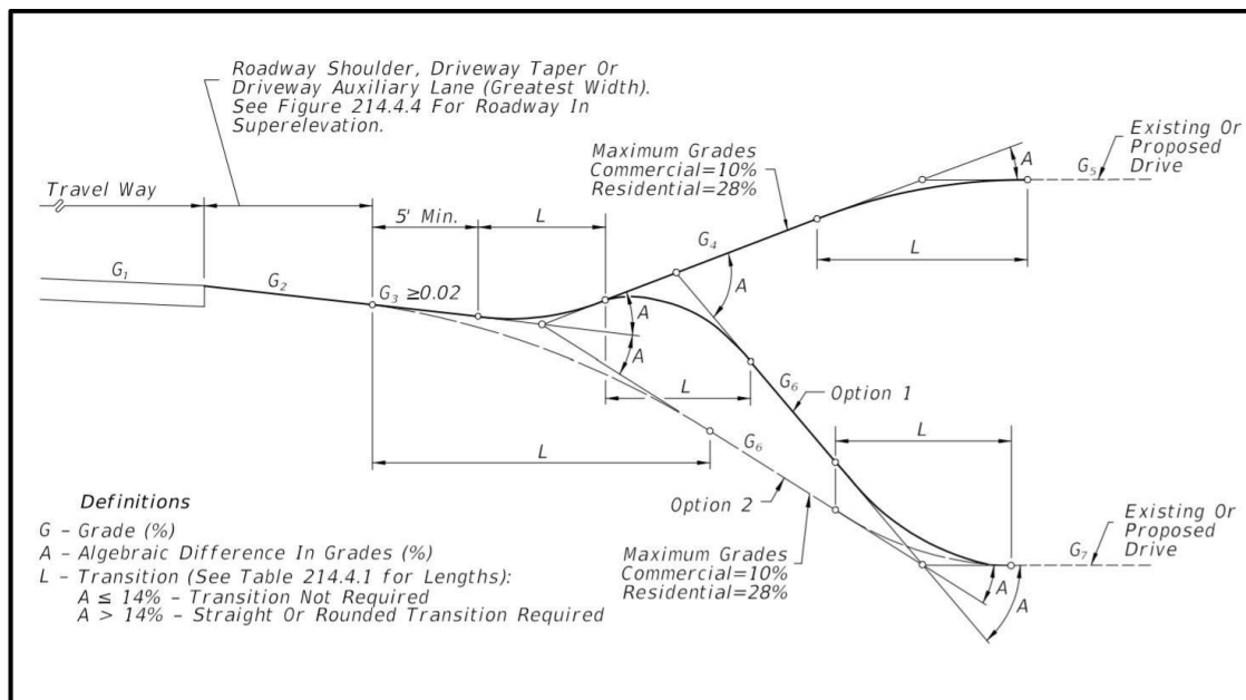
Figure 59 | Flush Shoulder Roadway Driveway Profiles
