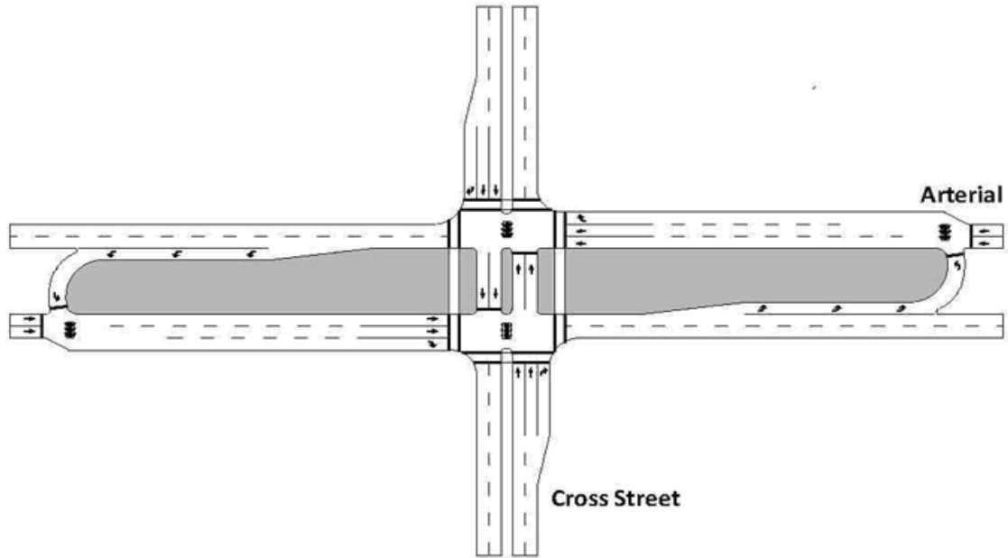
Figure 108 | Signalized Restricted Crossing U-Turn (RCUT), or Superstreet
