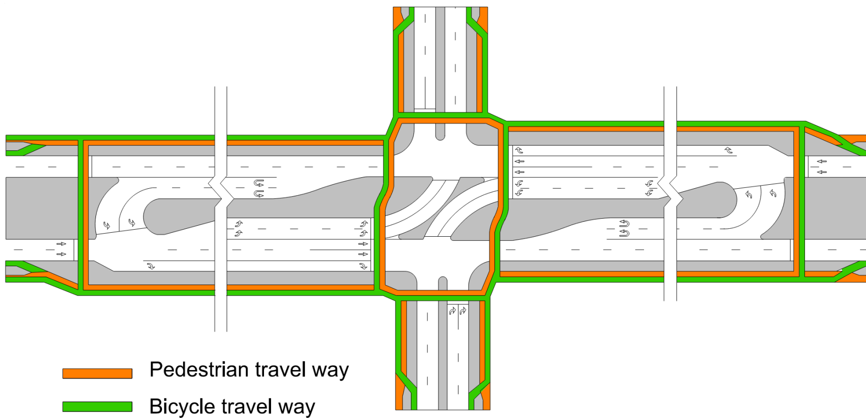
Figure 114 | RCUT Shared Use Path Concept
