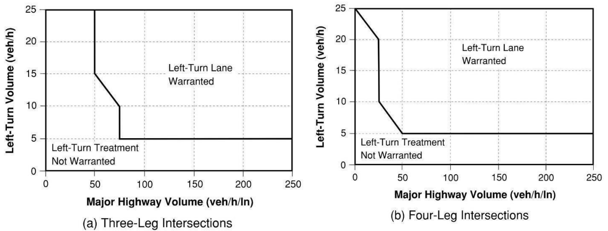
Figure 80 | Left-Turn Lane Warrants for Urban and Suburban Arterials
