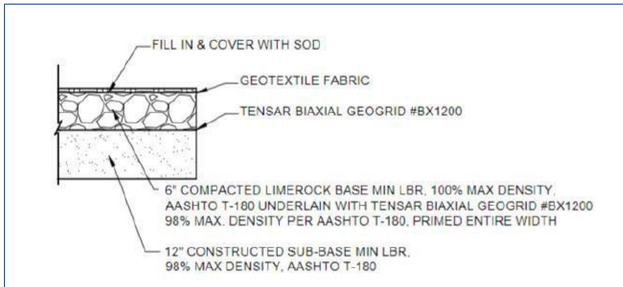
Figure 24 | Example Emergency Access Driveway Stabilization Detail
