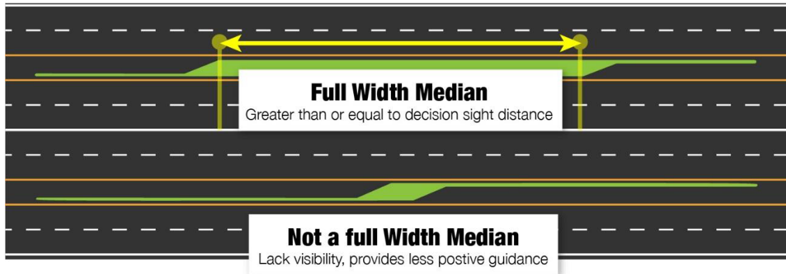
Figure 34 | Length of Full Width Median
