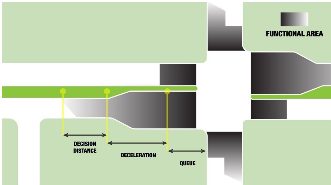
Figure 7 | Functional Area of an Intersection
