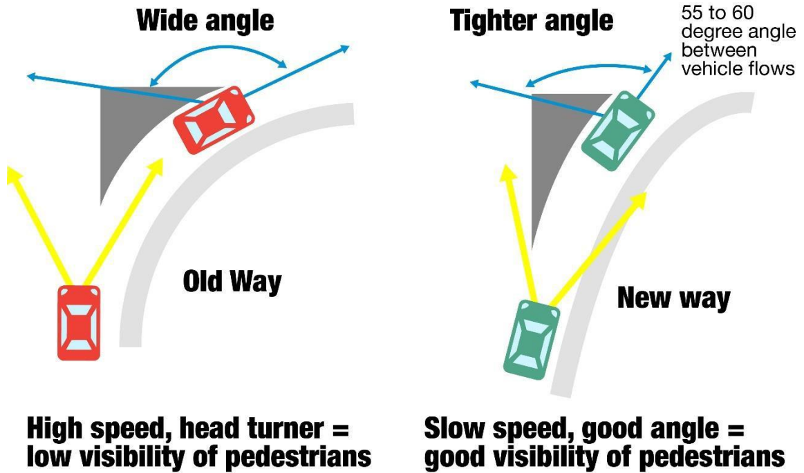
Figure 75 | Right-Turn Channelization
