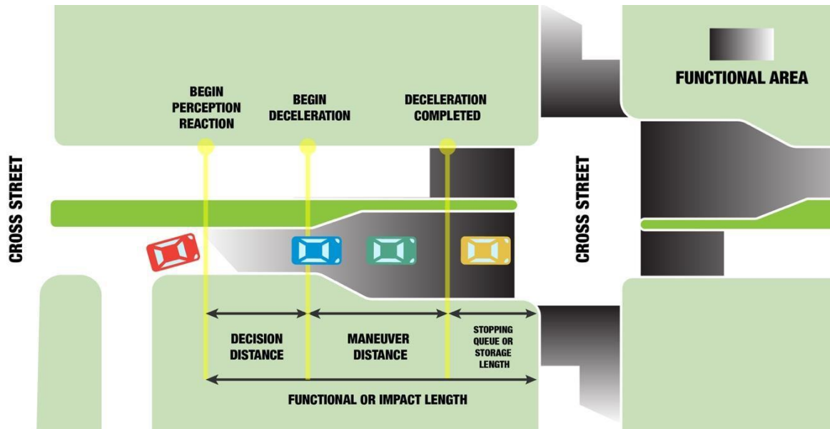
Figure 15 | Functional Area Diagram
