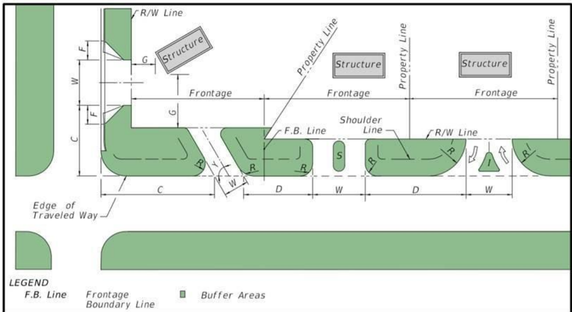
Figure 45 | Driveway Terminology
