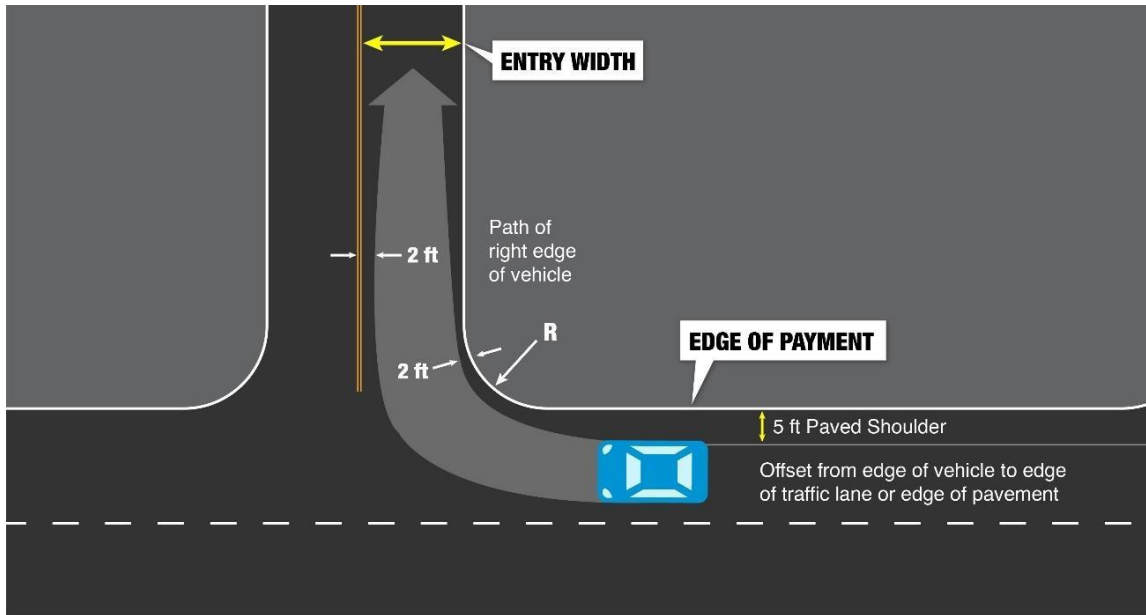
Figure 50 | Driveway Width and Radius
