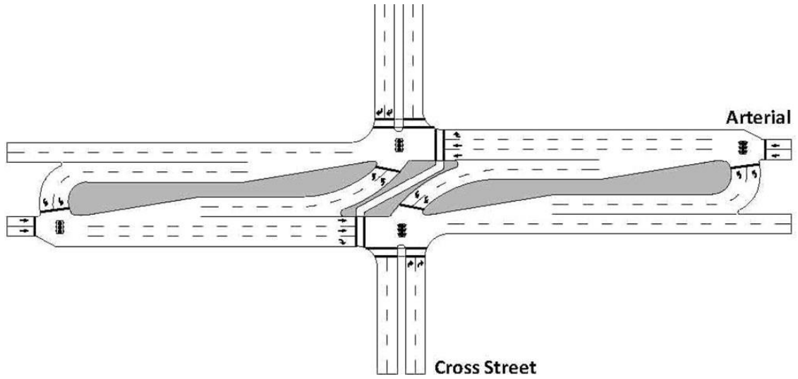
Figure 108 | Signalized Restricted Crossing U-Turn (RCUT), or Superstreet
