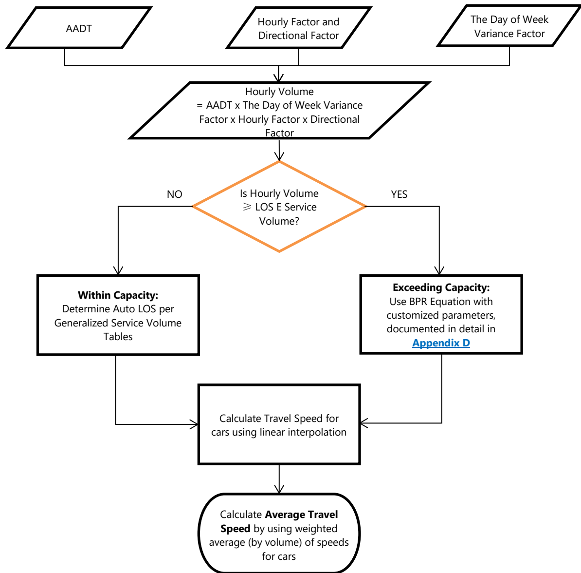
Figure 4.3 Estimation of Average Travel Speed on Arterials
