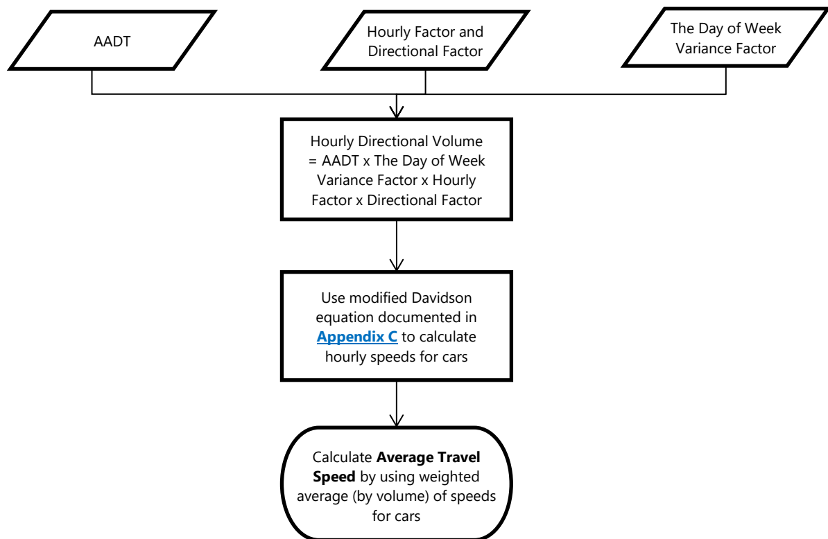
Figure 4.2 Estimation of Average Travel Speed on Freeways
