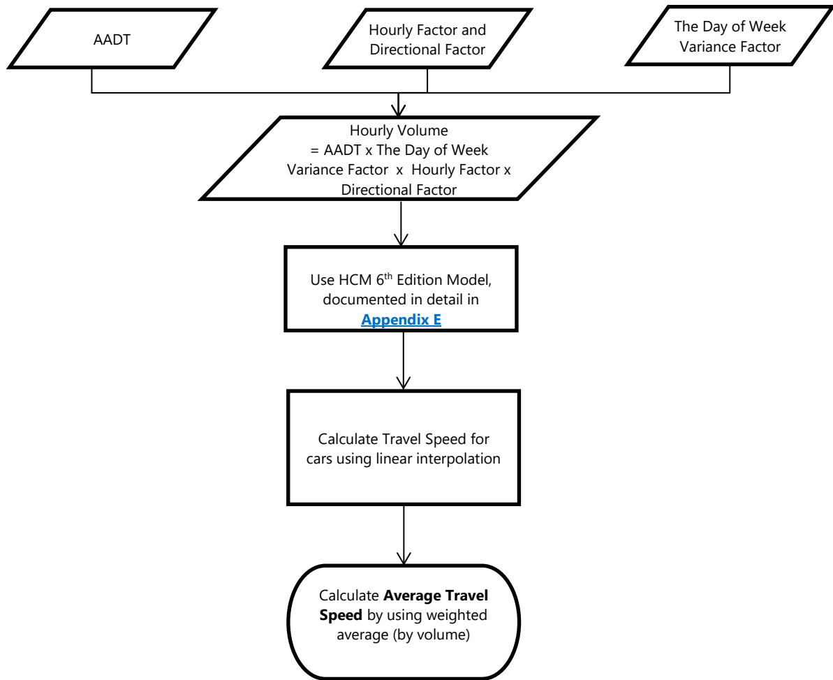
Figure 4.4 Estimation of Average Travel Speed on Two-Lane Highways
