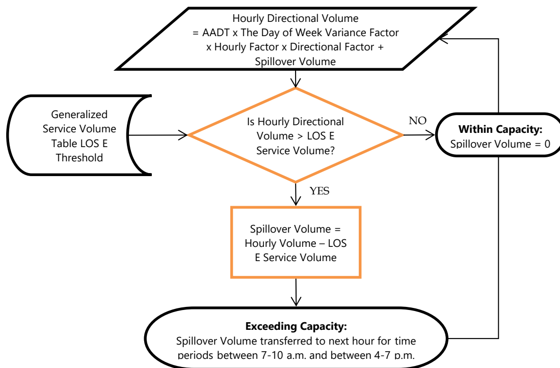
Figure 3.1 Queue Spillover Algorithm
