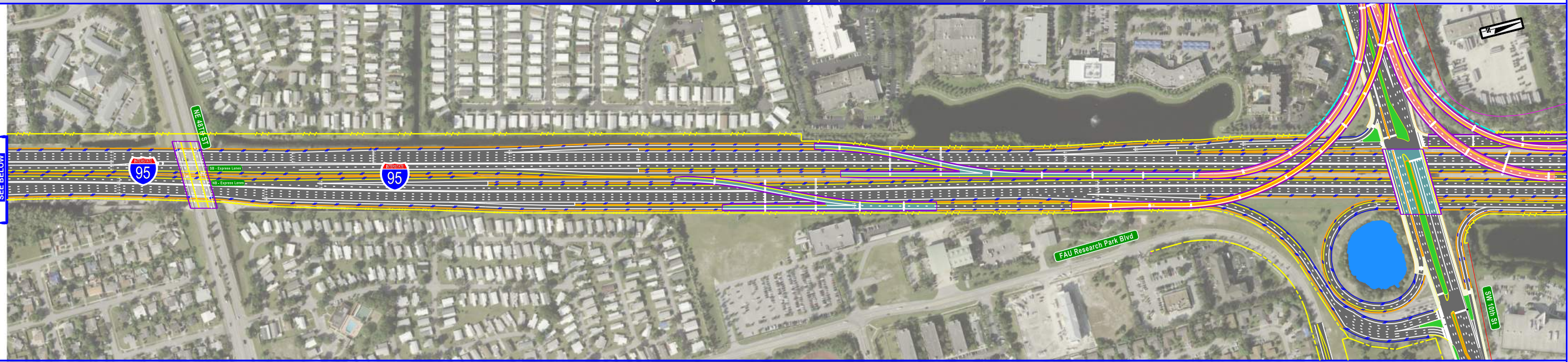
Build 2 - I-95 at SW 10th Street Interchange and Managed Lanes PD&E Study: I-95 (NE 48th Street to SW 10th Street)
