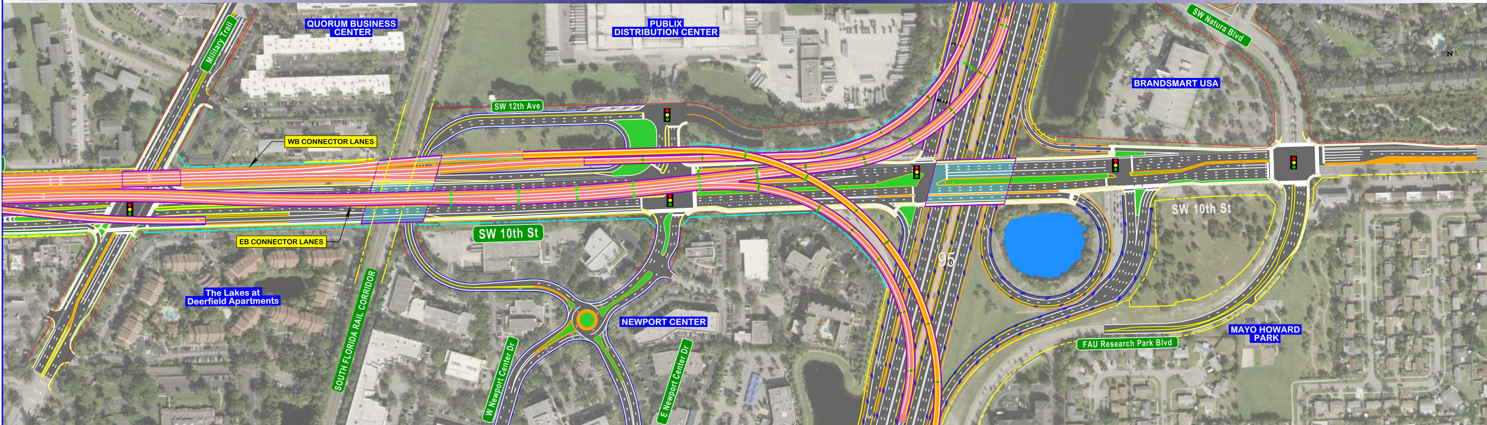
Build 2A - I-95 at SW 10th Street Interchange and Managed Lanes PD&E Study: SW 10th Street at I-95 Interchange (Without Bridges)
