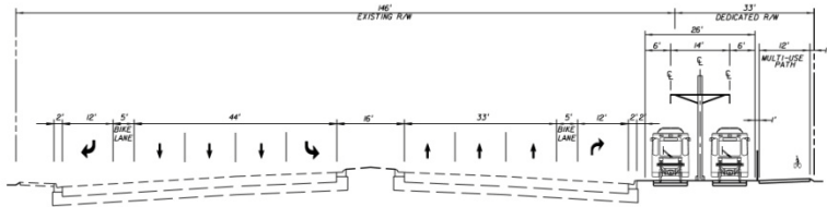
PROPOSED CONDITION - DEDICATED DOUBLE TRACK ON WEST SIDE
