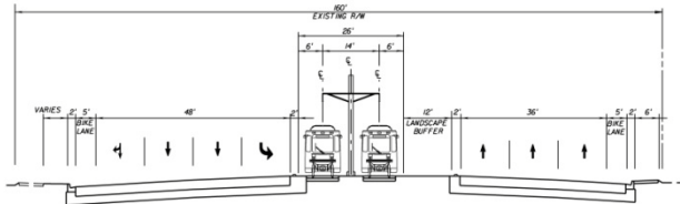
PROPOSED CONDITION - DEDICATED DOUBLE TRACK IN MEDIAN
