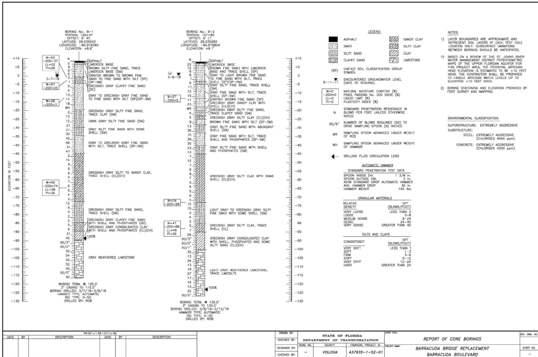
Figure 9-4: Typical Report of Core Borings Sheet
