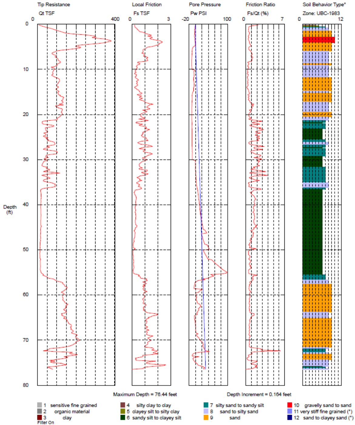
Figure 4-3: Typical Log from Electric Piezocone
