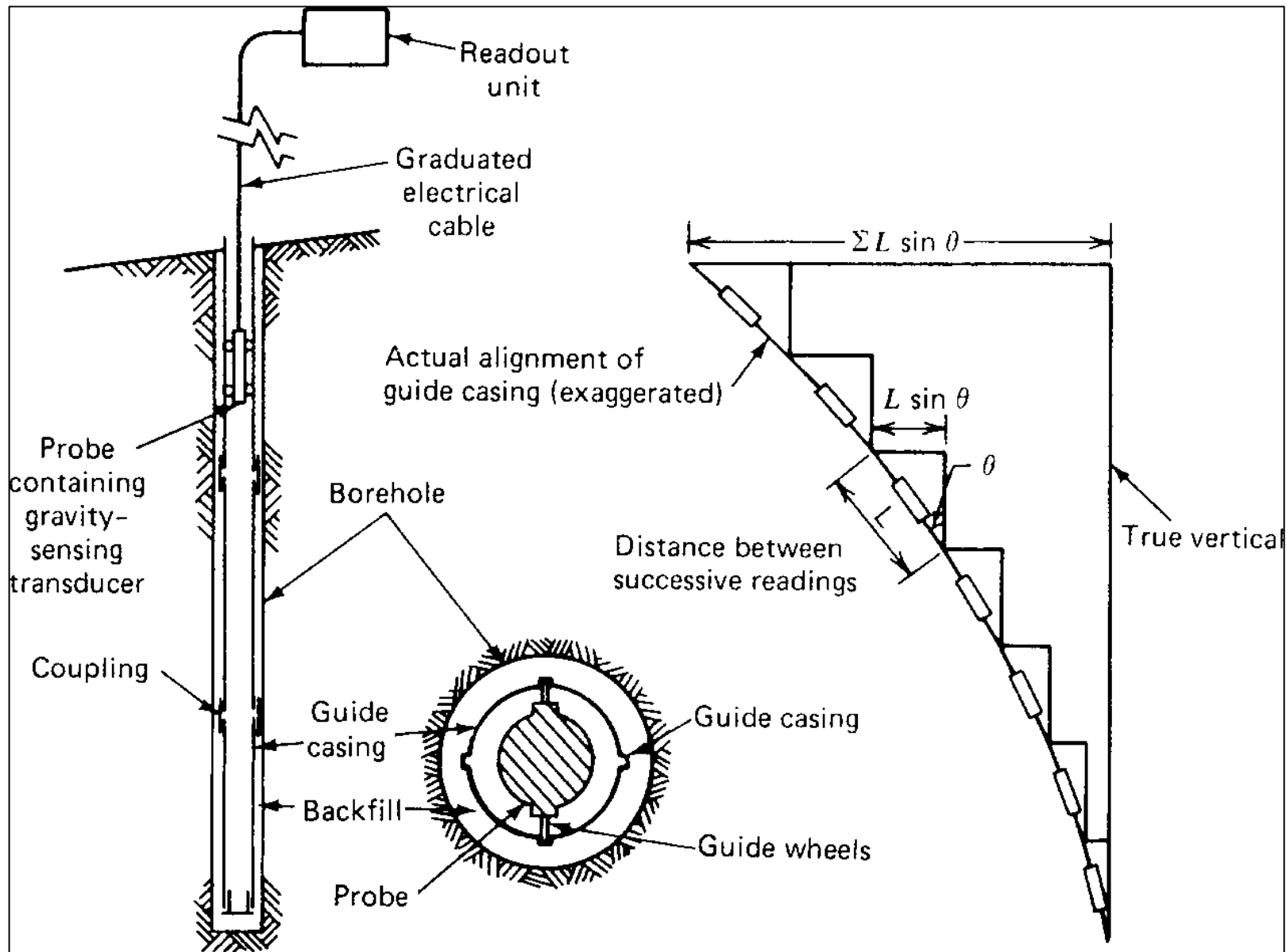
Figure 7-1: Principle of Inclinometer Operation (After Dunnicliff, 1988)
