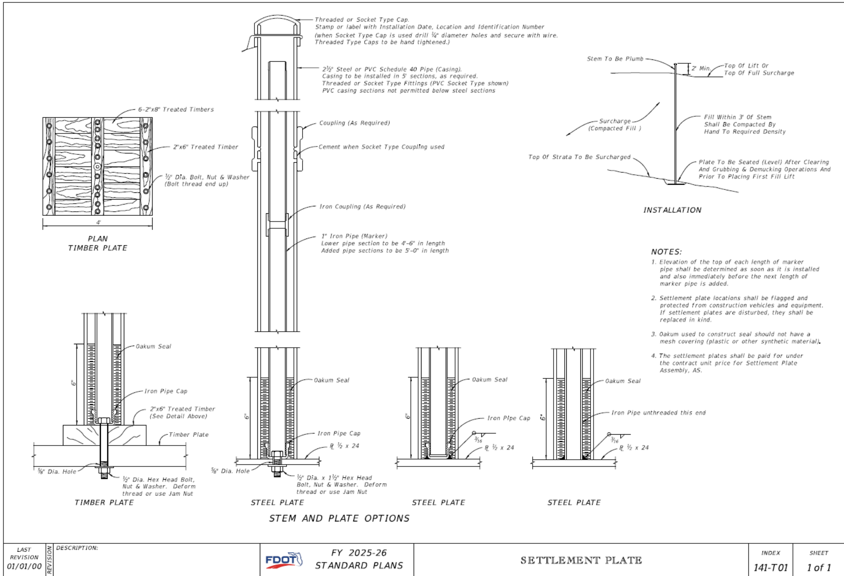
Figure 7-2: Typical Settlement Platform Design (Standard Plans, Index 141-T01)
