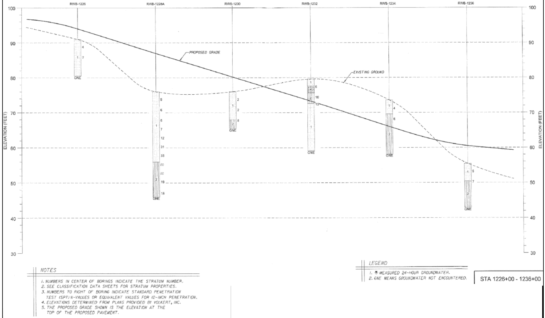
Figure 9-3: Example of Generalized Soil Profile
