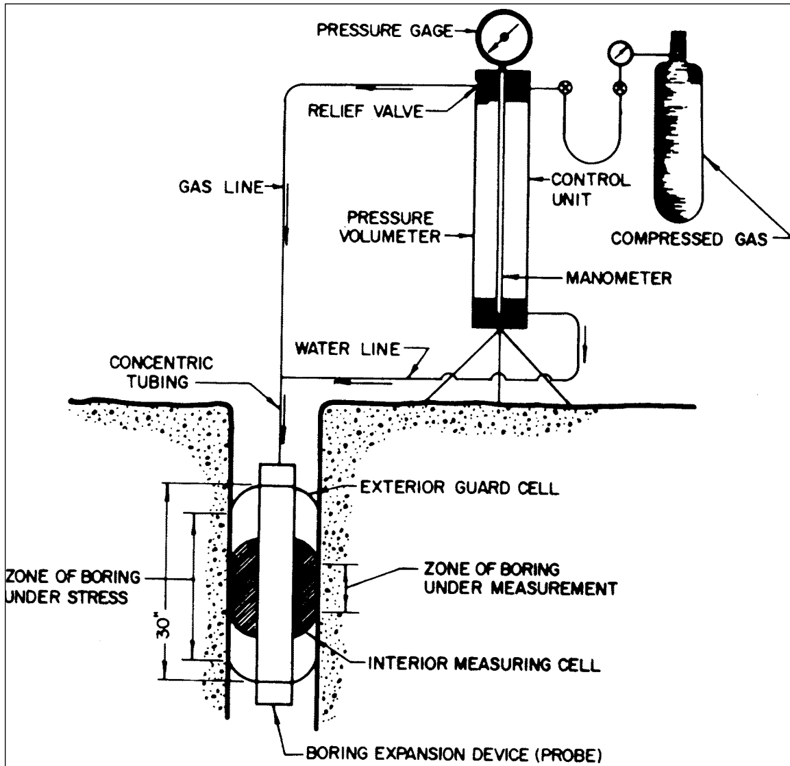
Figure 4-7: Menard Pressuremeter Equipment (After NAVFAC, 1986)
