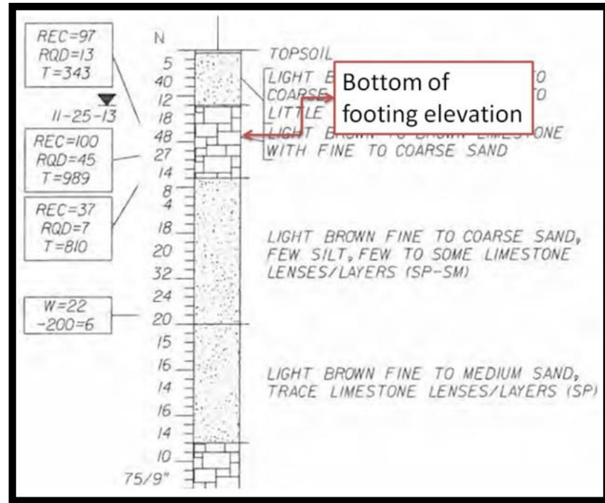
Figure 8-2: Example of Rock Lens Punching Condition
