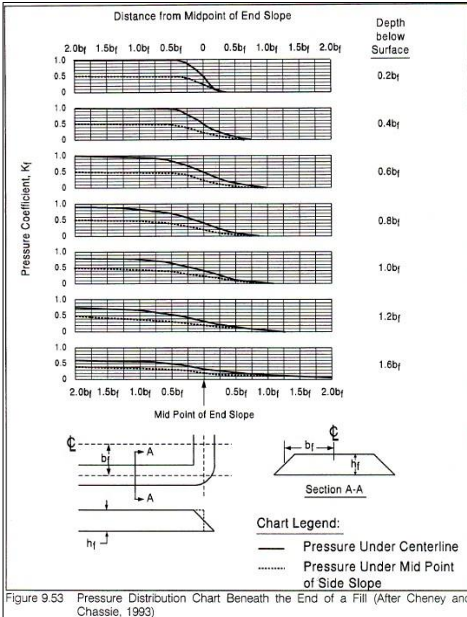
Figure C-1: Pressure Distribution Chart Beneath the End of a Fill
