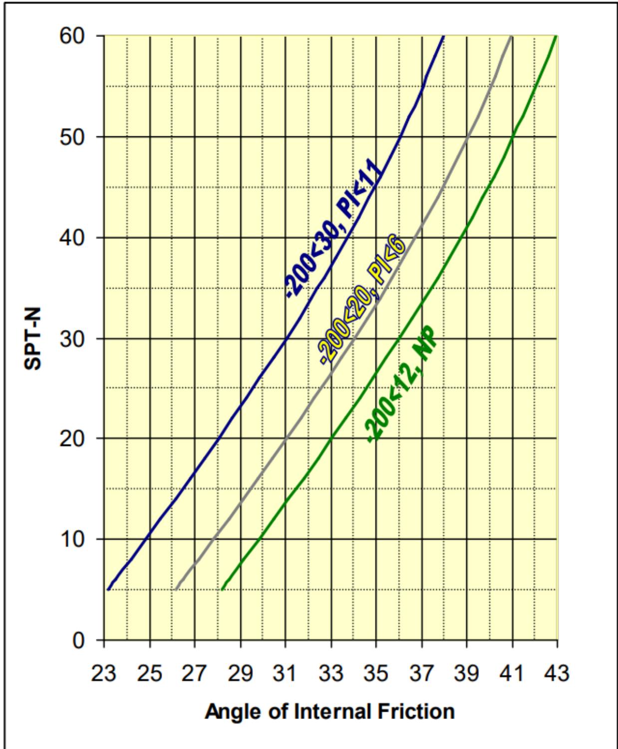
Figure 6-1: Angle of Internal Friction vs. SPT-N (After Peck, 1974)
