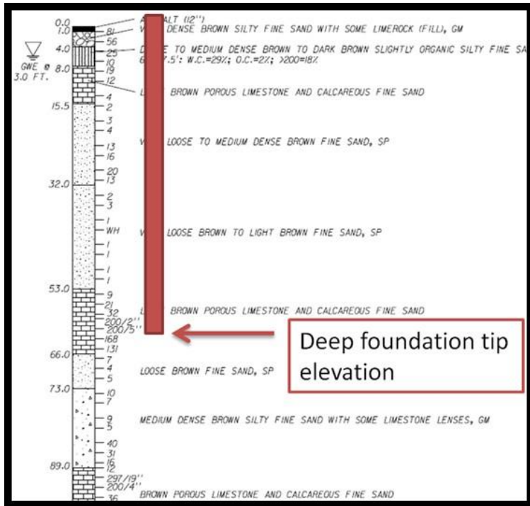
Figure 8-2: Example of Rock Lens Punching Condition
