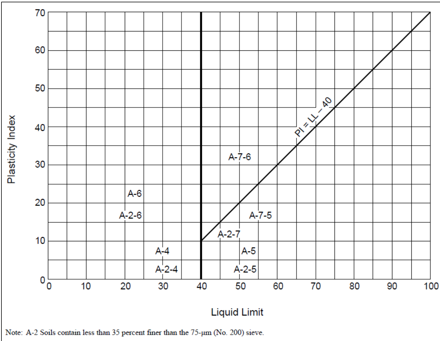
Figure 6-4: AASHTO Soil Classification System (AASHTO M 145, 2025) Continued
