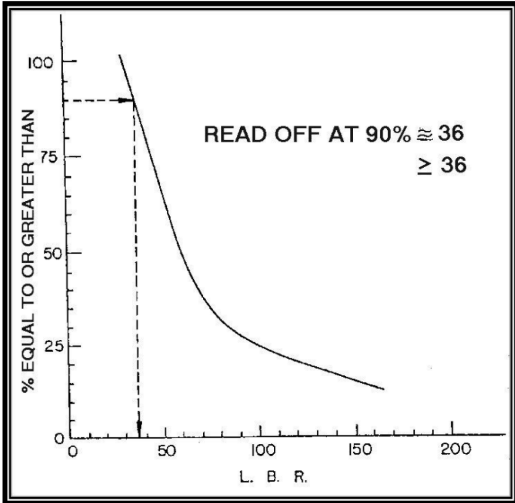
Figure 8-1: Design Example 1 (LBR Design Methods) 90% Method
