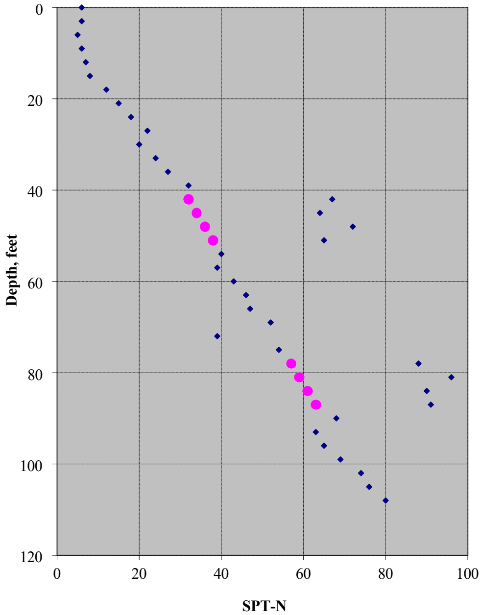
Figure 4-1: Example SPT N Adjustments Due to Plugged Sampler
