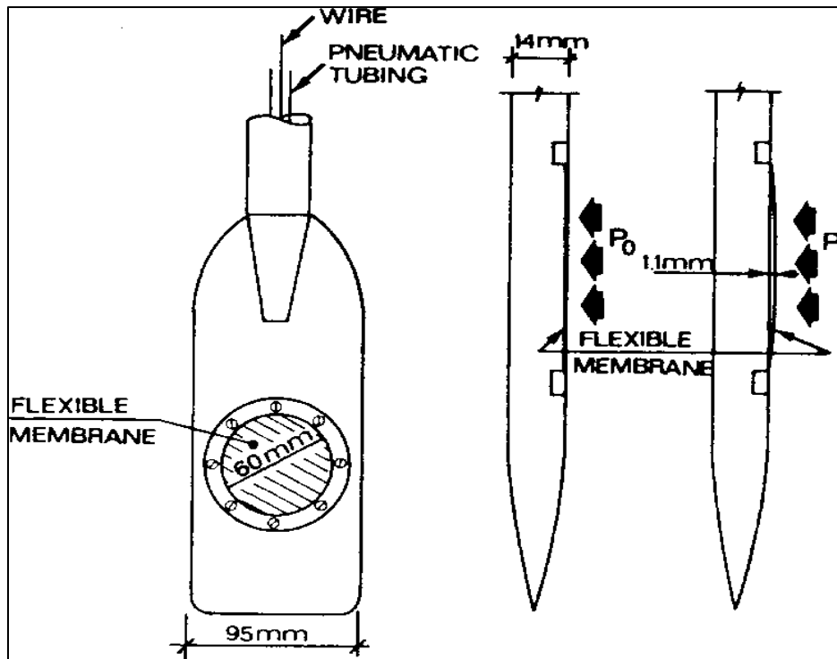
Figure 4-5: Schematic of the Marchetti Flat Dilatometer (After Baldi, et al., 1986)
