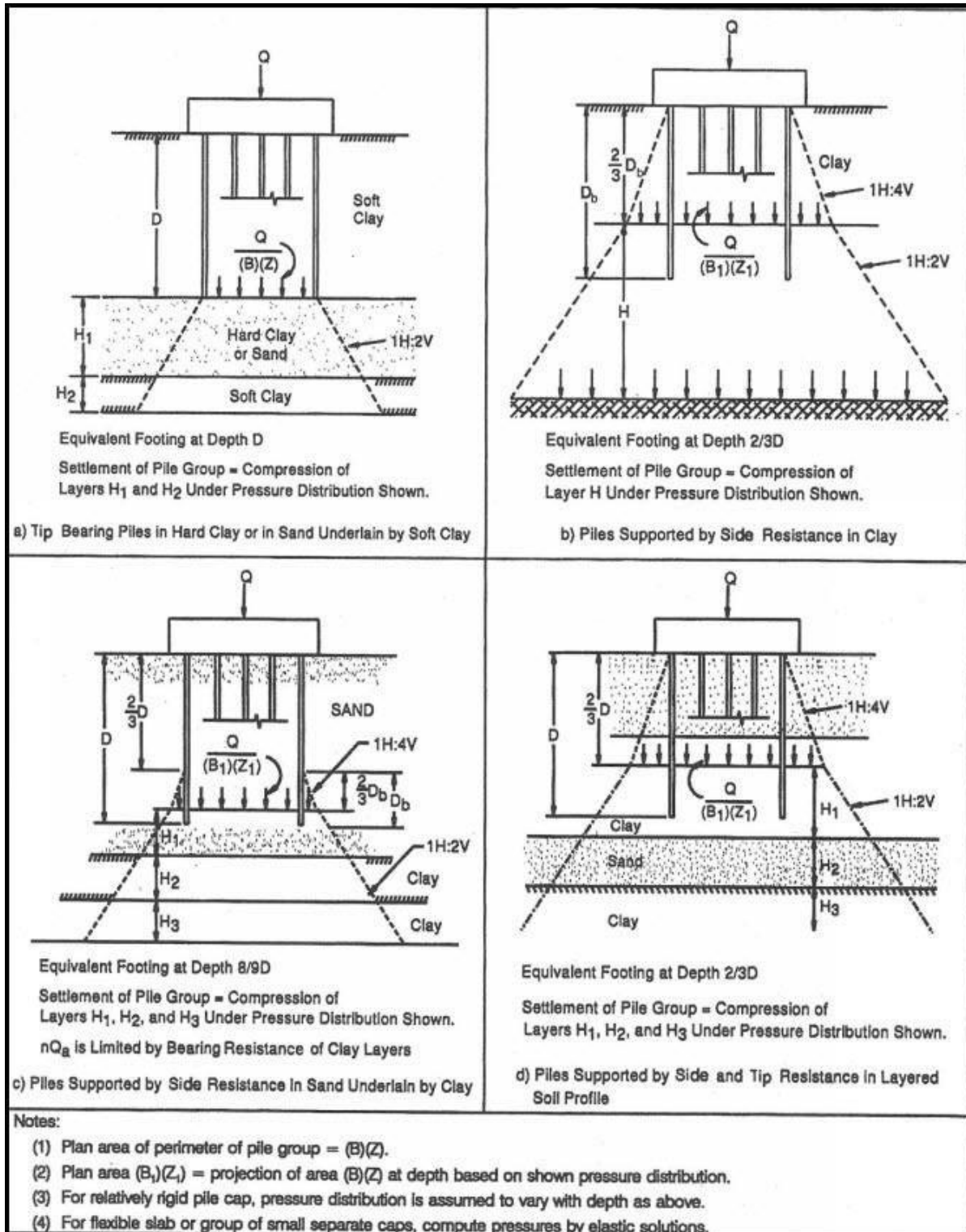
Figure 3-1: Stress Distribution Below Equivalent Footing for Pile Group (AASHTO 2020)
