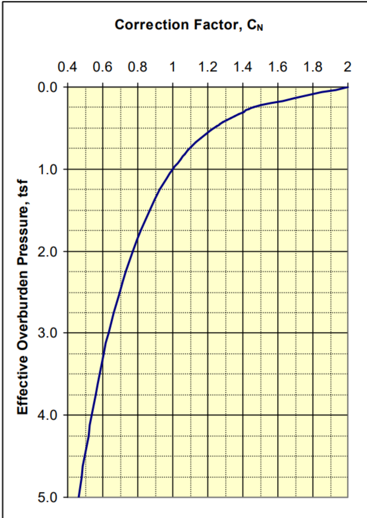
Figure 6-2: C_N vs. Effective Overburden Pressure (After Peck, 1974)
