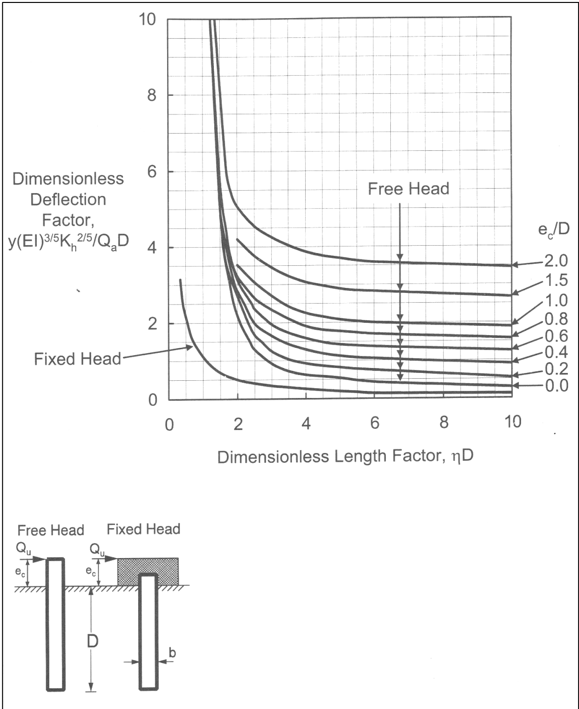
Figure G-1: Broms' Deflection Factor vs. Length Factor
