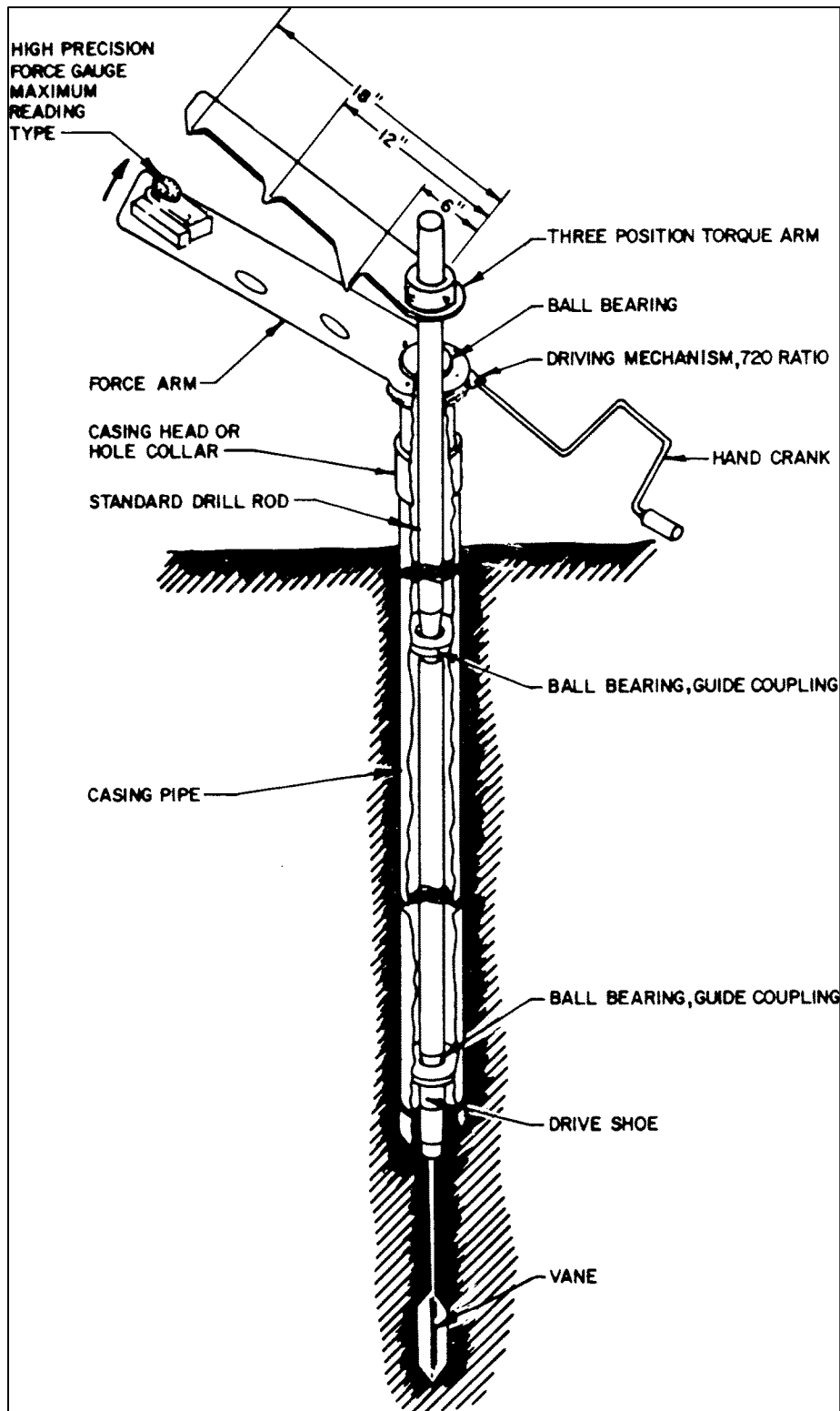
Figure 4-8: Vane Shear Test Equipment (After NAVFAC, 1986)
