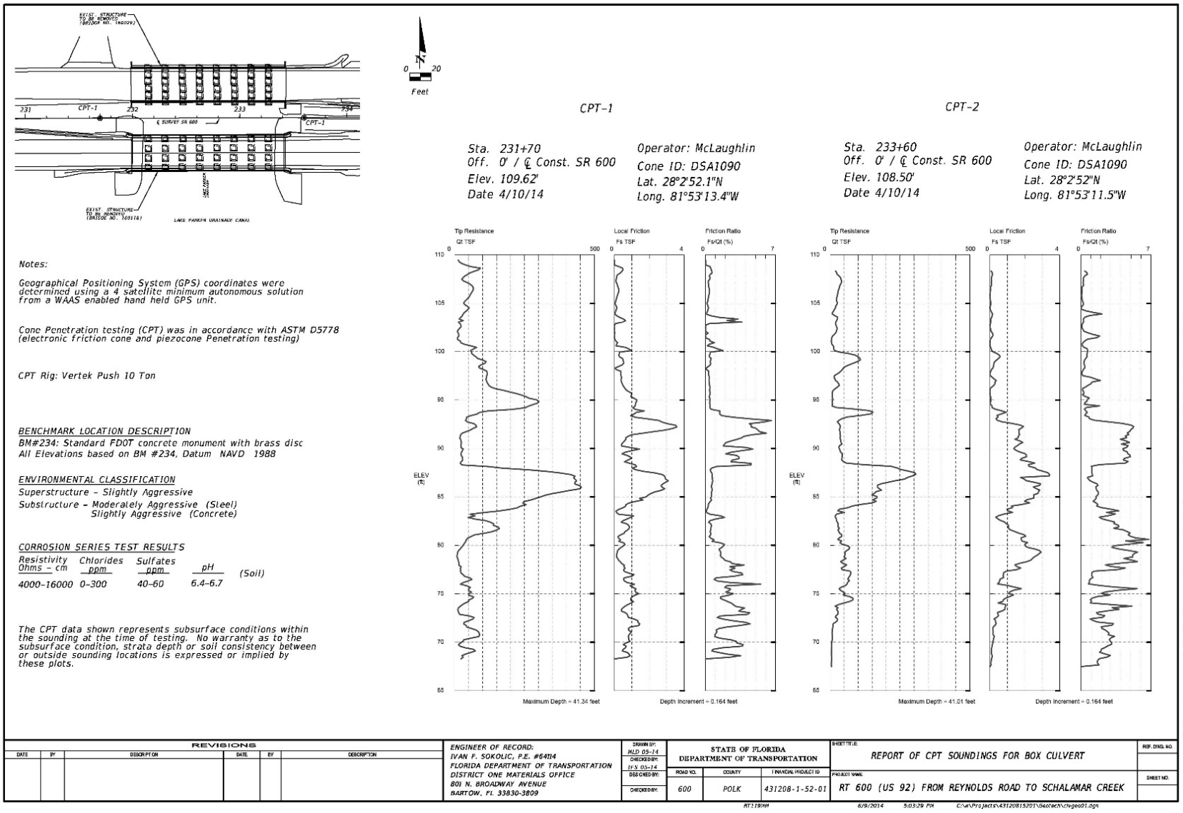
Figure 9-5: Typical Report of Cone Soundings Sheet
