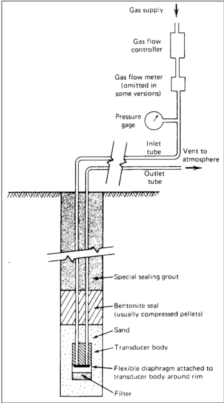
Figure 7-3: Example Schematic of Pneumatic Pore Pressure Transducer
