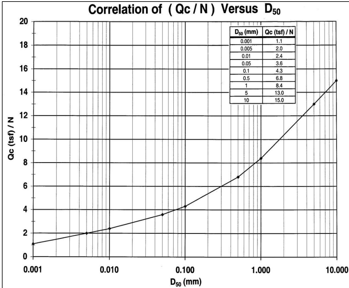
Figure B-2: Correlation of ( Q_c/N ) vs. D_{50}
