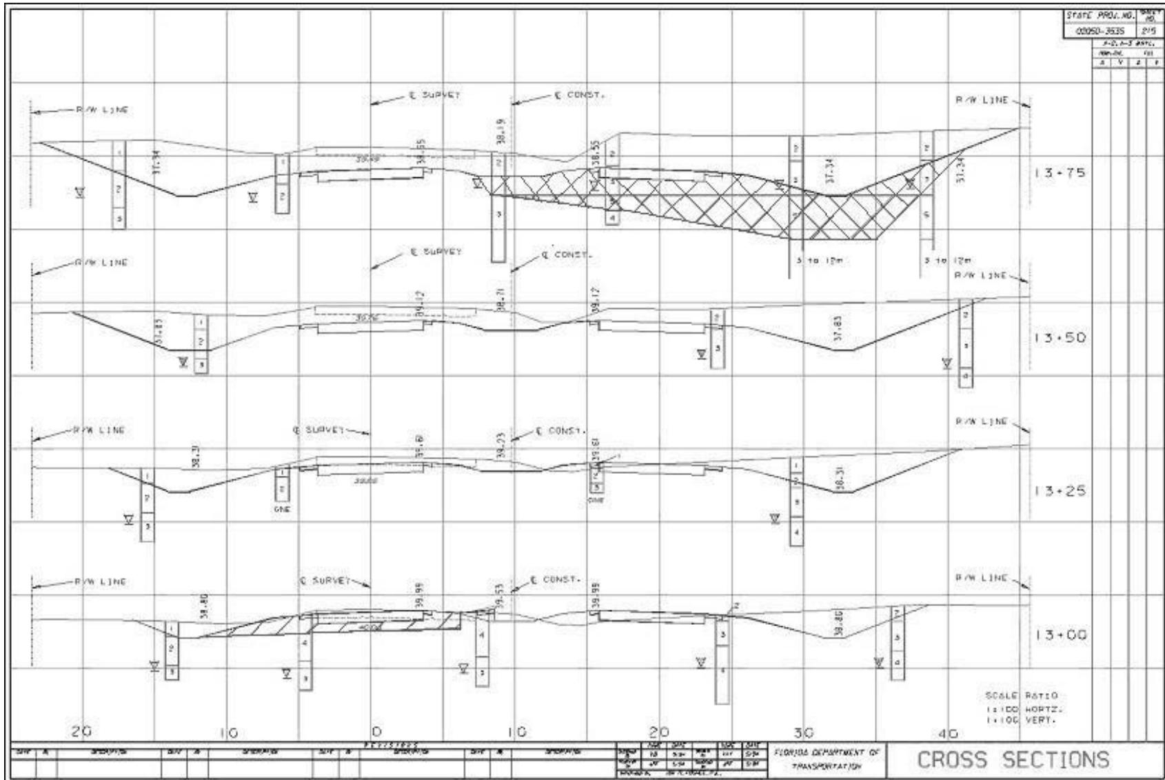
Figure 9-2: Typical Roadway Cross-Section Sheet
