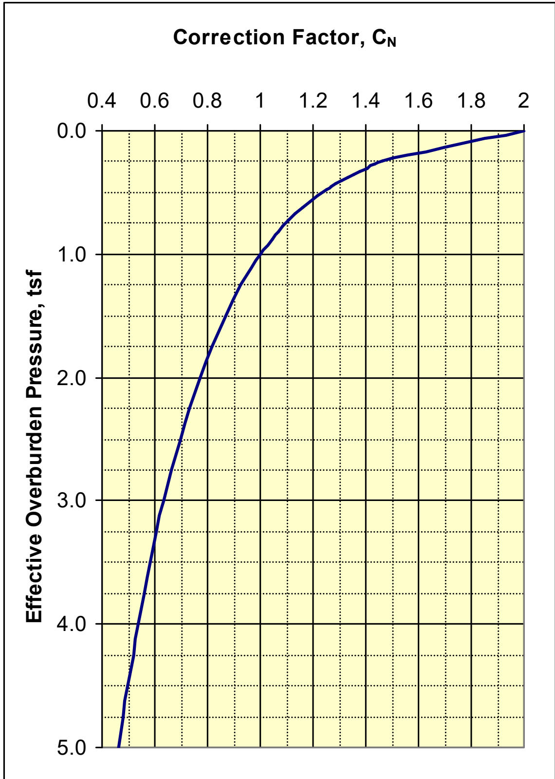
Figure 17, C_N vs. Effective Overburden Pressure (After Peck, 1974)
