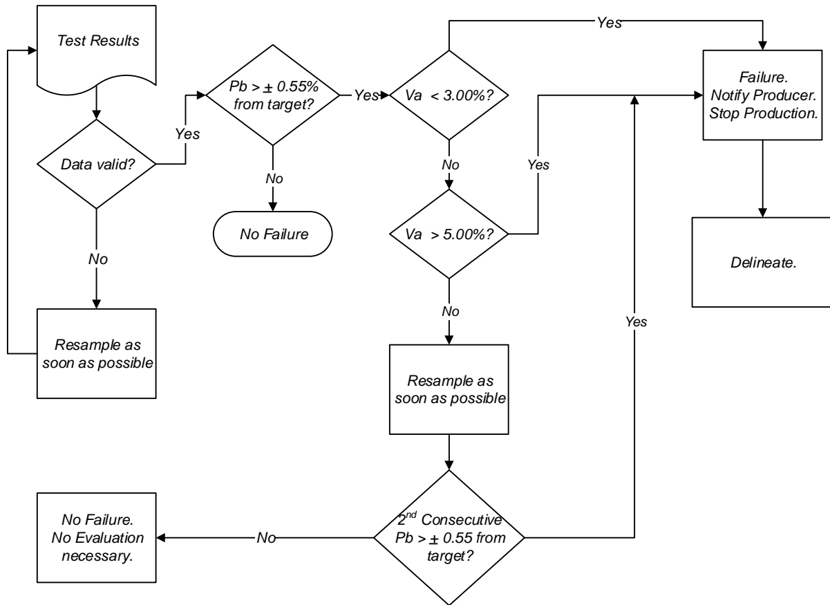
Figure 3 Asphalt Binder Content (P b ) – Dense Mixes
