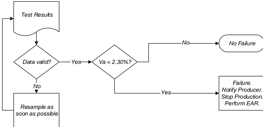
Figure 1 Low Air Voids at the Asphalt Plant – Dense Mixes
