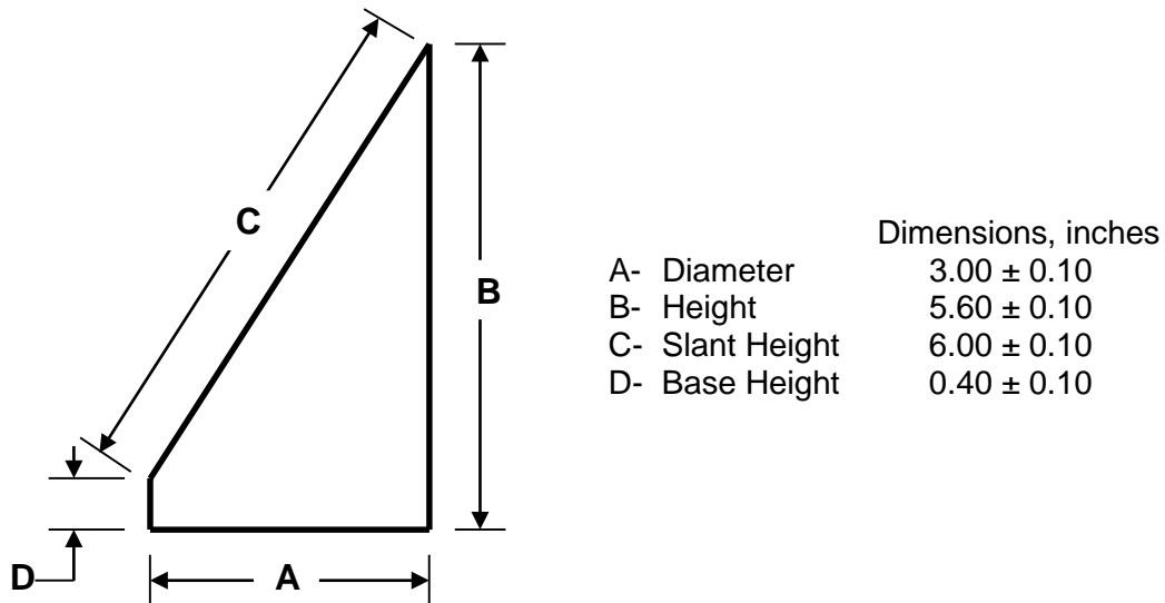
Fig. 1 – Concrete Test Specimens
