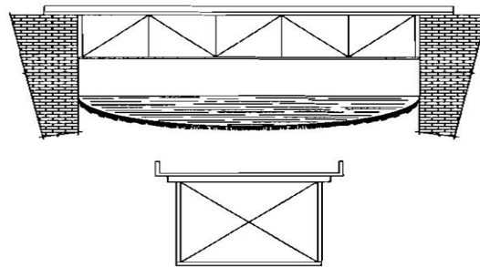
DECK TRUSS
