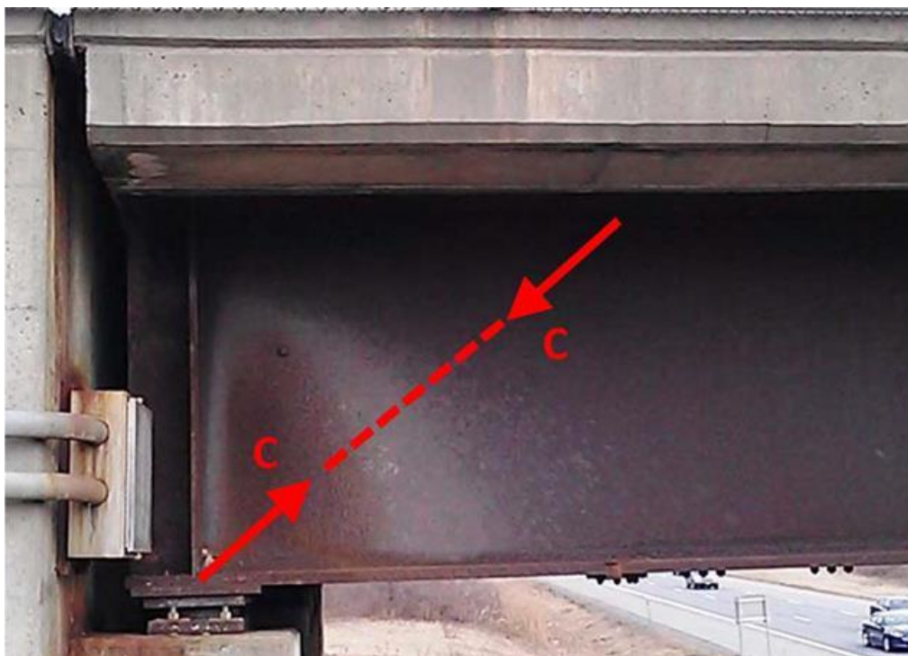
Figure 4.10 Steel Bridge Girder. Diagonal Line Represents a Compression Path.
