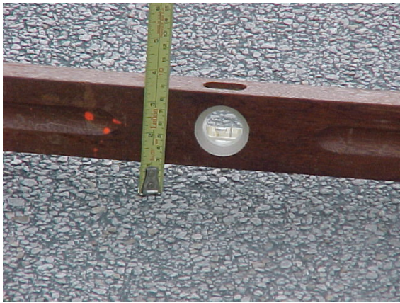
Measuring the depth of a depression.
