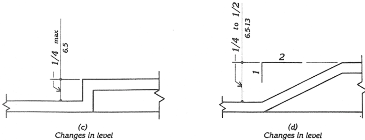
Fig. 7 Accessible Route
