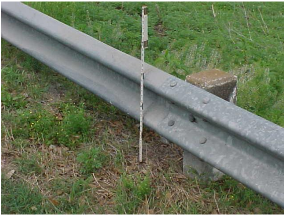
This guardrail section may not meet MRP standards, because the height above the ground is incorrect.
