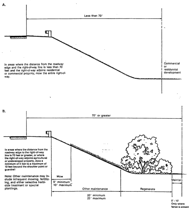
Figure 5 Slope mowing limits: Rural arterial and all limited access
