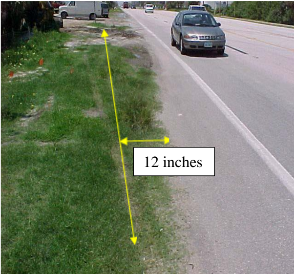
Measure encroachment on to the paved shoulder, if it is one foot or greater for more than 25 continuous feet then it would not meet desired maintenance conditions.
