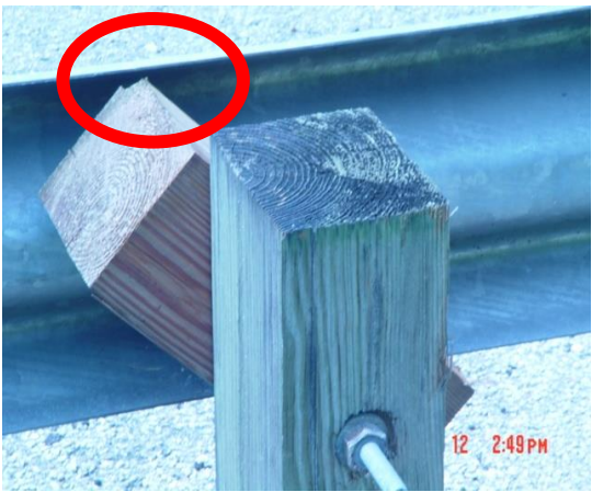
A guardrail block is considered twisted if there is a gap between the top edge of the block and the guardrail.
