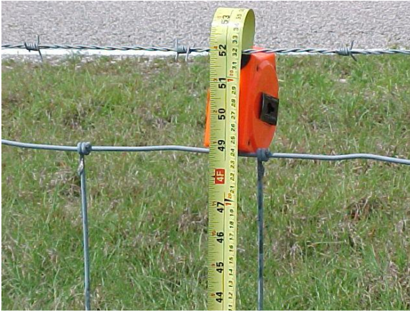
Measure the height of the fence from natural ground to the top of the fence fabric.
