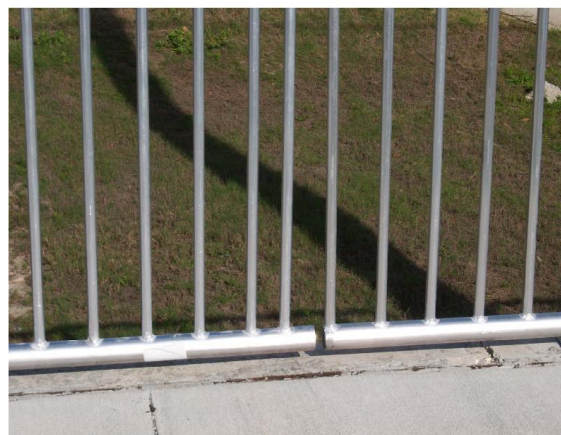
Picket railing missing steel sleeve at expansion joint. This does not meet MRP standards.
