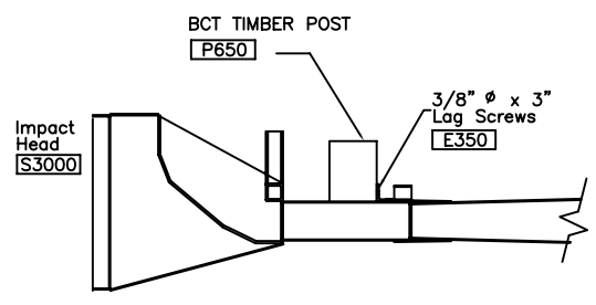
IMPACT HEAD CONNECTION DETAIL
