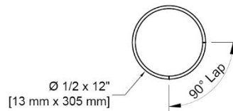
Grade 60 Ø 1/2 x 12" [13 mm x 305 mm] Rebar ring
