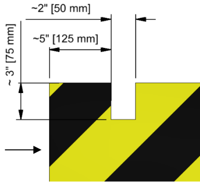
NOTCH DETAIL TYPICAL AT ALL 4 CORNERS
