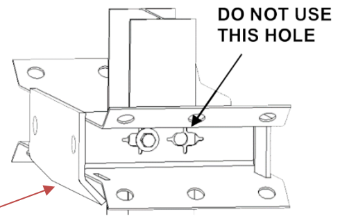
Orientation of the MATT™ Double Spacer Detail
