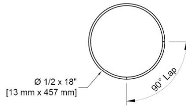
Grade 60 Ø 1/2 x 18" [13 mm x 457 mm] Rebar ring
