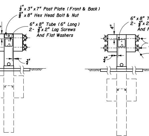
SECTION DD POST NO. 4
