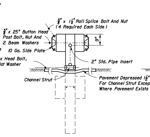
SECTION BB POST NO. 2
