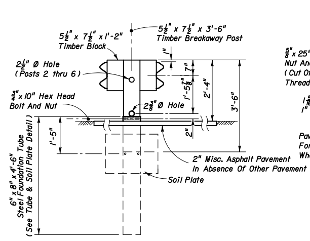
TYPICAL DIMENSIONING
