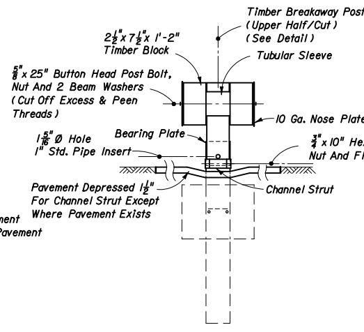
SECTION AA POST NO. 1
