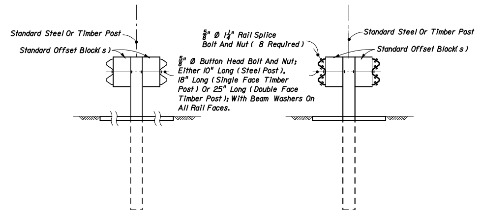
SECTION FF POST NO. 7
