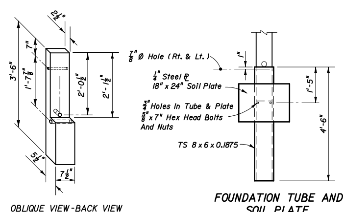
OBLIQUE VIEW-BACK VIEW POST NO. 1
