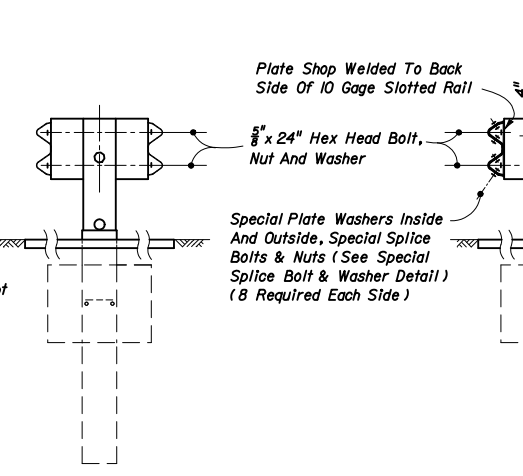
SECTION CC POST 3 & 5
