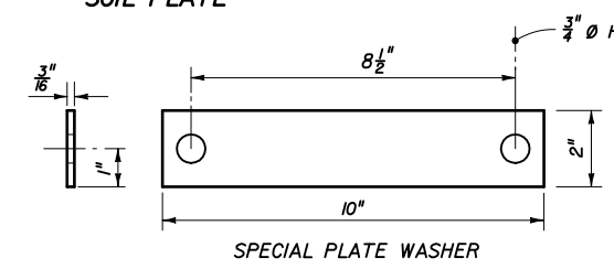
SPECIAL PLATE WASHER
