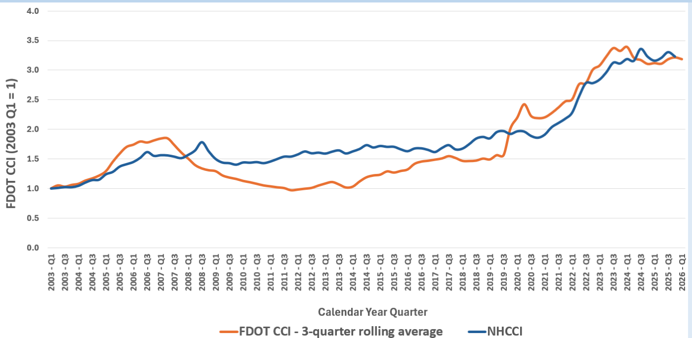
Figure 1. Quarterly FDOT CCI, Updated to Calendar Year 2026 Q1 (FY 2026 Q3)
