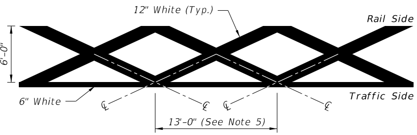
RAILROAD DYNAMIC ENVELOPE (RDE) PAVEMENT MARKING DETAIL
