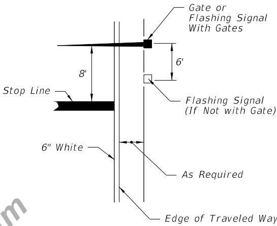
RELATIVE LOCATION OF CROSSING TRAFFIC CONTROL DEVICES
