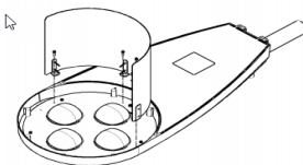
Figure 2 – House Side Shield
