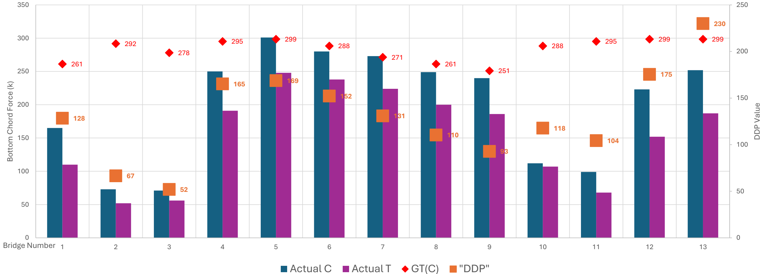
STR I Bottom Chord Forces (k)
