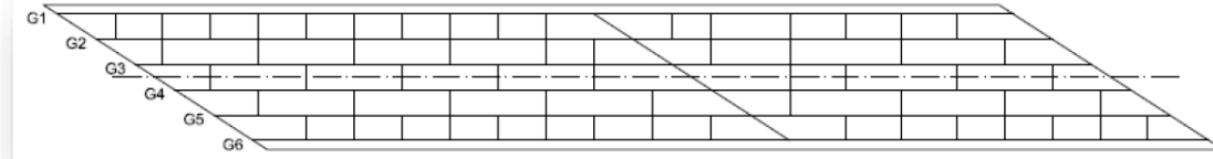
Bridge 10 ( L_s = 202 ft, 158 ft; w_g = 57.5 ft; \theta = 57.2^\circ, 57.2^\circ, 57.2^\circ ; I_s = 0.47 ) BE535
