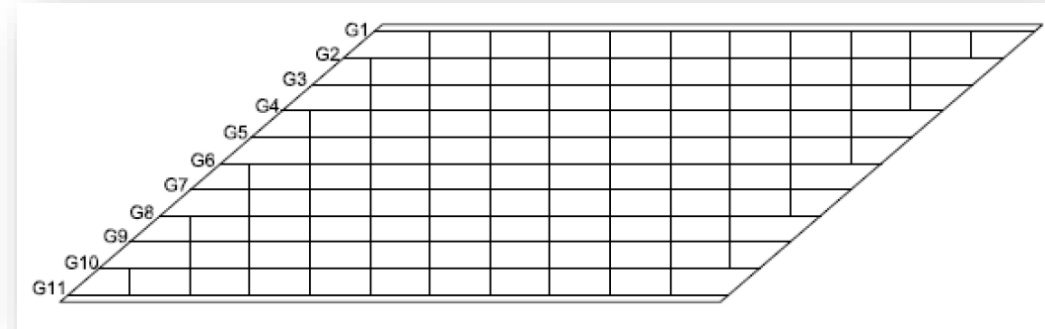
Bridge 1 ( L_s = 208 ft; w_g = 82.5 ft; \theta = 49.4^\circ, 49.4^\circ ; I_s = 0.46 ) BE535
