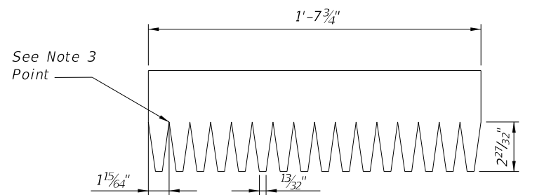
SHELL STENCIL FOR SCRIBING AND CUTTING BOTTOM TAPER FOR PART 1 (Not to Scale)
