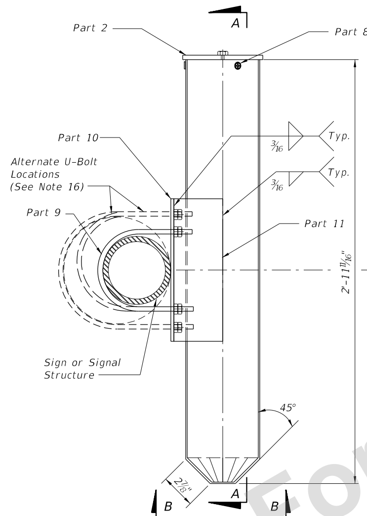
SIDE VIEW DAMPING DEVICE
