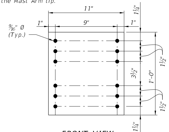
FRONT VIEW PART 10 BACKING PLATE
